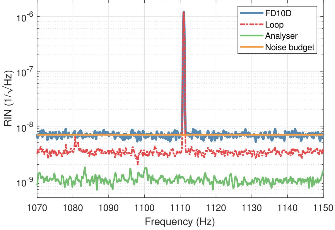
Figure 7.3: The bias of the FD10D was set to 0.6 V, and it was exposed to 15 mW of 1.55\,\mu\text{m} light. 15 mA of photocurrent was generated. The noise of the photocurrent produced by the FD10D (blue line) corresponds to the level predicted by Equation 7.3 (orange line) meaning that the increase in photocurrent can only be explained by an increase in quantum efficiency. The 1111 Hz signal was used to calibrate the measurement as this modulation also could be measured on the high-performance in-loop photodiode.
