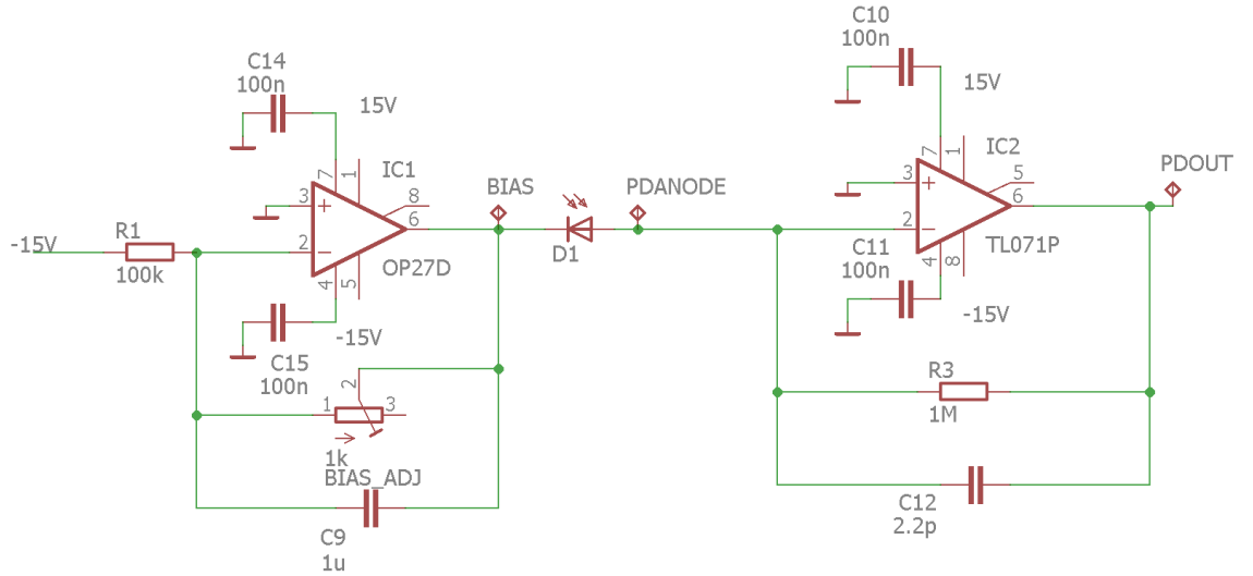
Figure B.2: Circuit used to measure the dark noise of photodiodes. The transimpedance amplifier used is identical to the one shown in Figure B.1. The bias voltage was generated using an OP27 op amp (OP27D) configured with so that the gain between the inverting input and the output of OP27D was > 1 .
