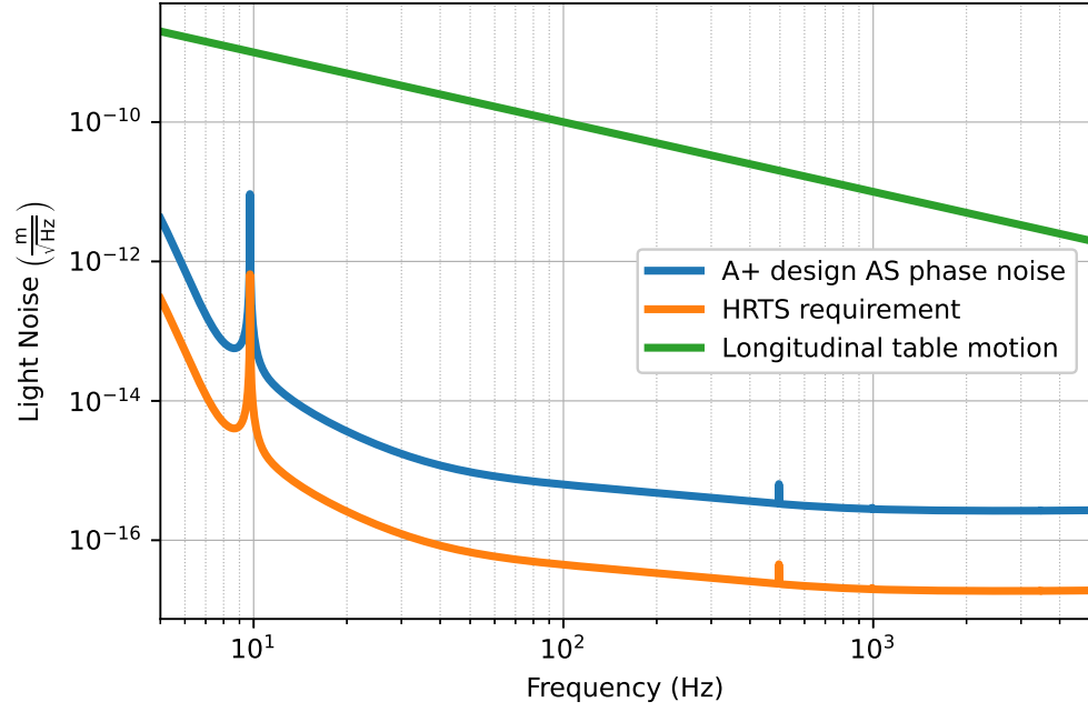
Figure 1.6: The phase noise between the LO and the AS beams causes noise. The sensitivity curve for A+ sets the limit on how much path length noise is acceptable between the AS and LO beams. The blue line shows sensitivity curve is shown in units of path length noise between the AS and LO beams, and the orange line shows the requirement of HRTS mirror motion. Replot, the y axis is shit!
