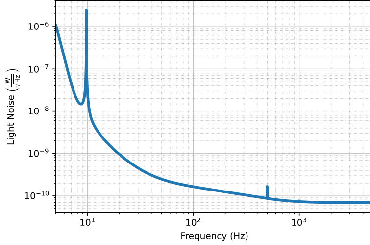
Figure 1.4: The intensity noise of the light at the AS port for the A+ detector. This was obtained by deconvolving the detectors sensitivity curve[11] with the function shown in figure 1.3.
