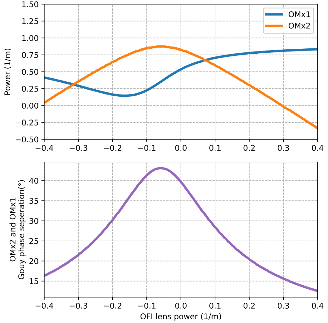
Figure 1.9: OFI lens power effects the optimal combination of OMx1 and OMx2 power required for 100% mode matching. The best choice of these lenses is the pair which gives the Gouy phase separation closest to 45^\circ .
