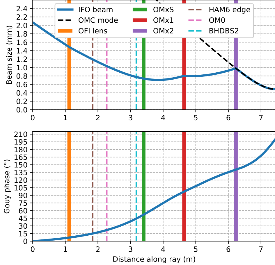
Figure 1.8: Top panel: the radius of the beam as it travels from the SRM ( z = 0 ) to the waist of the OMC. Significant points along the axis are marked with vertical lines. Bottom panel: The gouy phase shift accumulated by the beam as it propagates along the optical axis.
