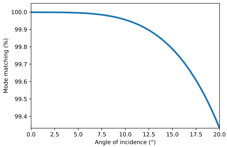
Figure 1.10: Mode matching degradation as a function of angle of incidence for OMx1 and OMx2.
