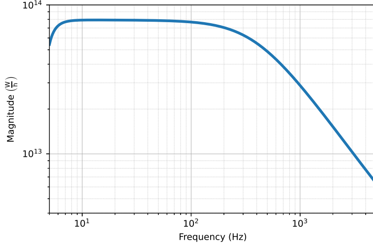
Figure 1.3: The linear response function between strain and light power at the AS port was obtained from a FINESSE simulation of the LLO detector[10]. The corner frequency at \approx 300 Hz comes from the pole of the coupled SRC-arm cavity. The behaviour below 6 Hz is due to optical spring effects.
