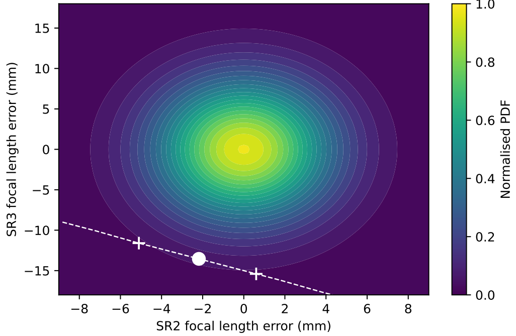
Figure 3.11: The measurement error of SR3 and SR2 follows a normal distribution. These were combined to make a 2-D normal distribution. Dark blue corresponds to the least likely combinations of SR3 and SR2, and bright yellow corresponds to the most likely. The measured Gouy phase was 21.3^\circ [150]; this is indicated by the white dashed line. The white circle marks the most likely combination of SR3 and SR2 which gives 21.3^\circ of Gouy phase, and the white crosses show one standard deviation from this. The white circle and crosses indicate that the focal length of SR2 is -3.205 \pm 0.003 m and the focal length of SR3 is 17.971 \pm 0.002 m.
