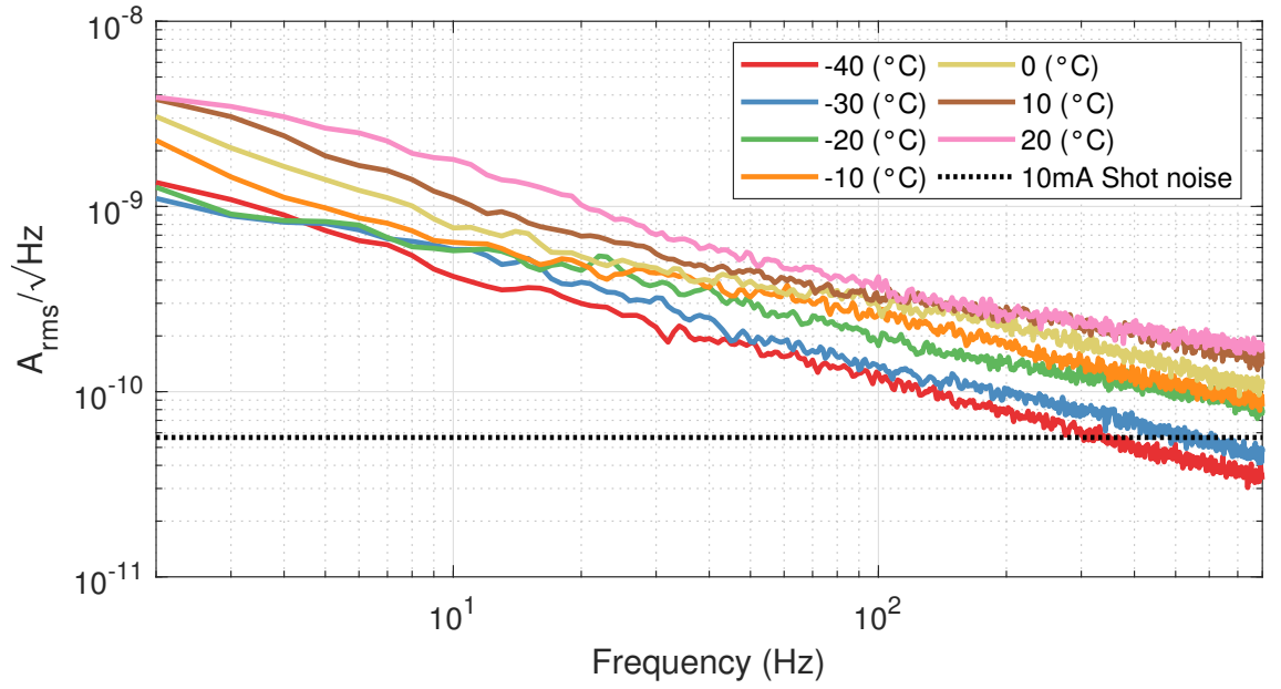
Figure A.14: IG26x500S4i at 1.0V reverse bias.
