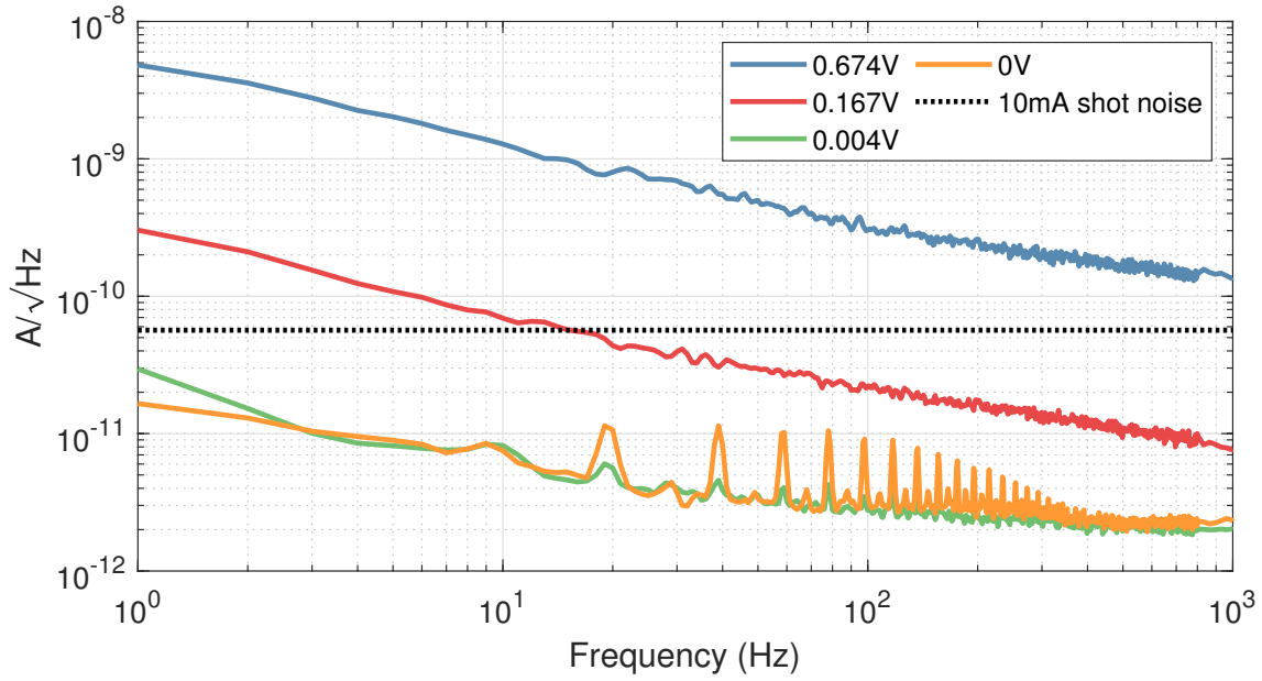
Figure A.2: Dark noise of the IG26x500S4i at 22°C for a series of reverse biases.
