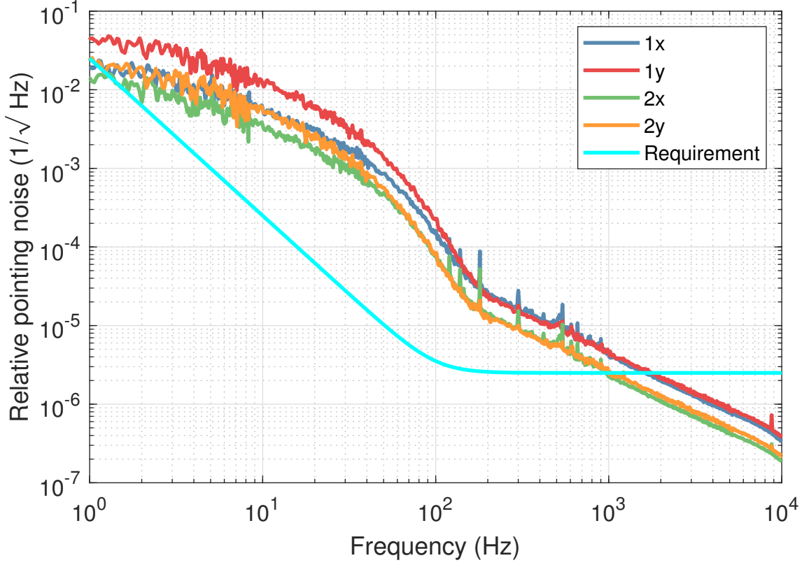
Figure 2.22: The four relative pointing degrees of freedom for the beam into the PMC was measured with the DBB. The requirement [128] is shown in light blue. The pointing noise is above the requirement, however the TnT lab has a higher amount of environmental noise than the PSL. Measurements below 200 Hz were be affected by scattering.
