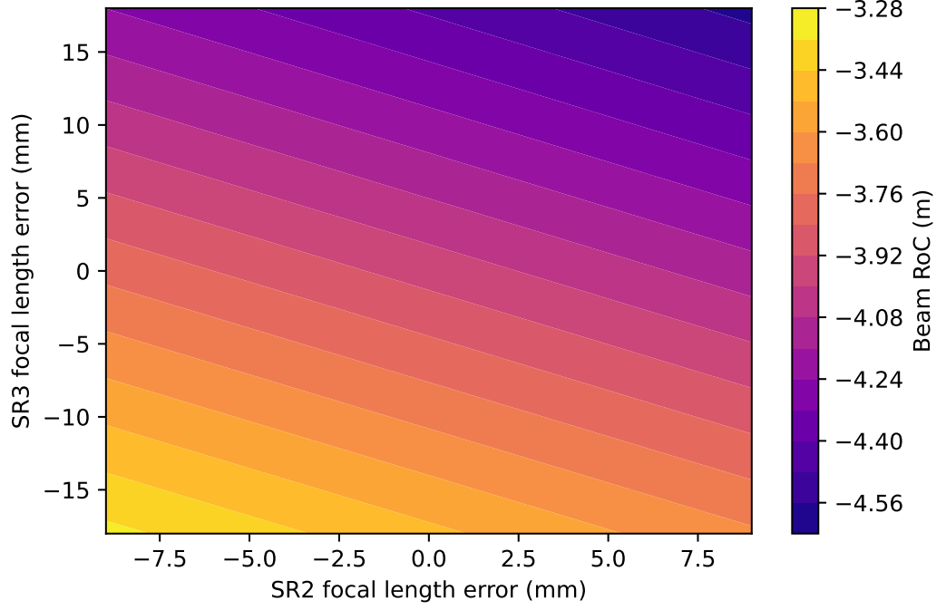
Figure 3.7: The RoC of the beam that is transmitted through the SRM as a function of the error ( \pm 3\sigma ) in focal length of SR3 and SR2. If the arm cavities and the SRC are well mode matched, then the RoC of the beam transmitted through the SRM would be \frac{5.67\text{m}}{1.45} = 3.91\text{m} .
