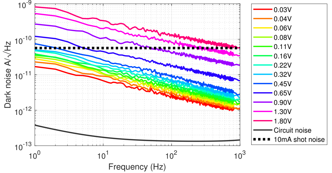
Figure 6.5: The dark noise of the FD10D increases as the reverse bias is increased. Above 0.6 V, the dark noise of the FD10D would limit the noise of a 10 mA current above 10 Hz. As the noise spectral densities have no knees, the function i_c/f^\beta can be fitted to the data. See Appendix A.1 for the dark noise spectra of other photodiodes. Below 0.9 V reverse bias, the spectra fall as f^{-0.45} and above 0.9 V bias the spectra fall as f^{-0.4} . The values for \beta are typical for ‘1/f’ noise [189]. The dark noise at 10 Hz for each reverse bias is shown in Figure 6.6 alongside the results for the other photodiodes that were tested.
