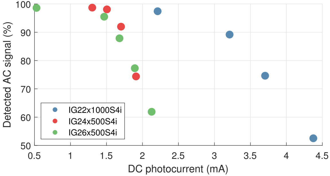
Figure 6.10: The saturation limit of the IG22x1000S4i, IG24x500S4i and IG26x500S4i photodiodes was measured. The photodiodes were biased so that their noise at 10 Hz was equal to the shot noise of a 10 mA current. The IG24x500S4i and IG26x500S4i were exposed to a beam with a 3\sigma width of 220 \mu m and the IG22x1000S4i was exposed to a beam with a 3\sigma width of 1000 \mu m. The size of the light modulation of known size was tracked as the DC photocurrent was increased. As the photodiodes saturated, the relative size of the AC signal decreased. The uncertainty in these measurements was \pm 1\% . These photodiodes had low saturation limits compared to the FD10D, which showed no signs of saturation up to 16.5 mA (see Figure 6.4).
