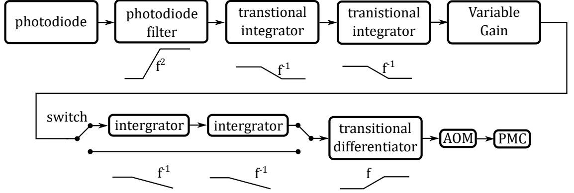
Figure 2.20: Block diagram of the components in the the intensity stabilisation servo. The transfer function of each block is described in Section 2.5.4.1 and Table 2.1. Additional integrators can be activated with a digital switch. The overall gain of the servo depends on a variable gain IC and the amount of light on the photodiode. The shaping of each block is indicated below it.
