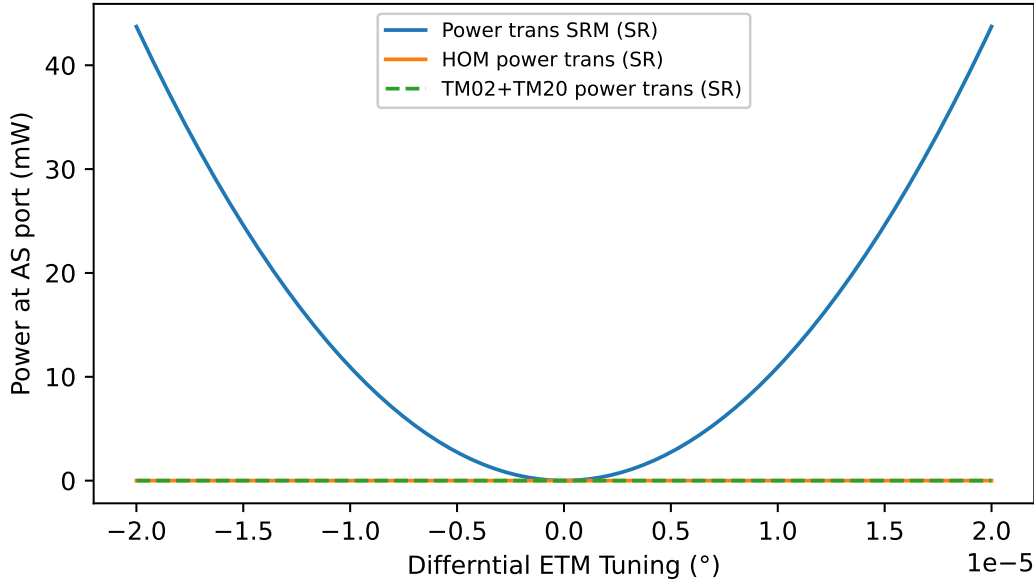
Figure 3.4: The minimum of the dark fringe is at 0° differential ETM detuning, as shown by the blue line. A slight offset causes light to be at the AS port. This result was used to determine tunings for simulating what effect focal length errors in SR3 and SR2 have on the beam transmitted through the SRM. The orange line and dashed green line show that the beam has a negligible HOM content.
