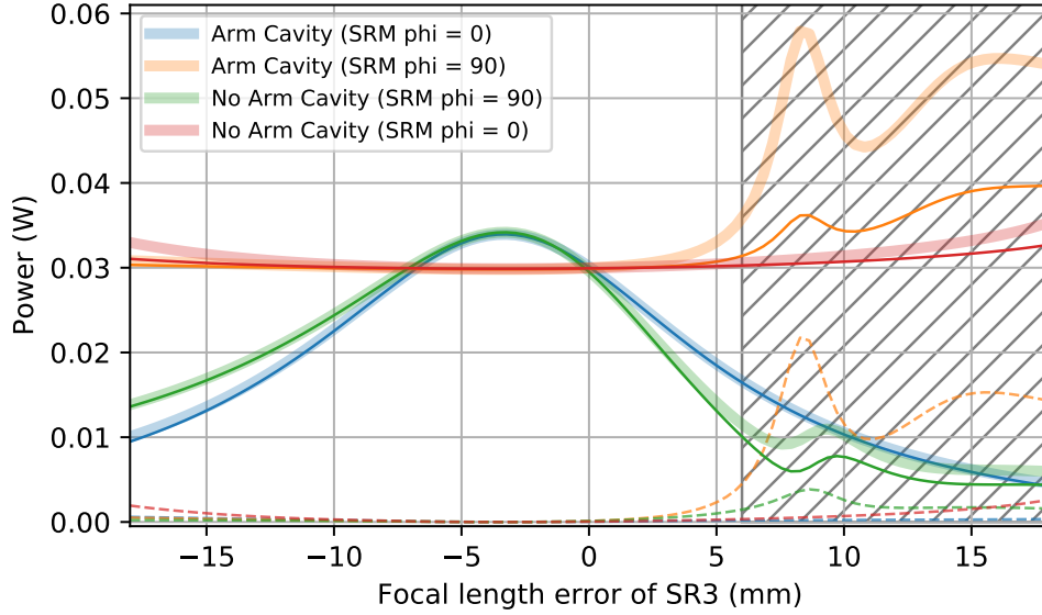
Figure 3.14: The total power transmitted through the SRM for each simulation is shown by the thick pale lines. The thin solid lines correspond to the power in the HG00 mode, and the thin dashed lines correspond to the power in the higher order modes. Blue lines show the behaviour when the interferometer has arm cavities and is in signal recycling mode, and the orange lines shows when it is in RSE mode. Green lines show how the power changes when the interferometer is configured for a single-bounce measurement and is in signal recycling mode, and the red line shows when its in RSE mode. The hatched region indicates where the SRC becomes unstable, and so the behaviour of the interferometer cannot be accurately simulated for these values of focal length.
