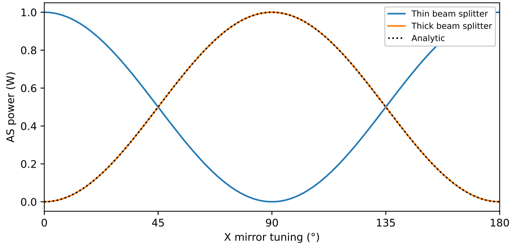
Figure 3.2: The simulation of a Michelson interferometer with thin a beam splitter is shown in blue. The same simulation was done with a thick beam splitter, this is shown in orange. The analytic behaviour of a Michelson interferometer (Equation (3.1)) is shown by the dashed black line. The tuning of one of the arm mirrors was changed and the power at the AS port was simulated. Comparing the outputs of the simulation to Equation (3.1) shows that thick beam splitters should be used.
