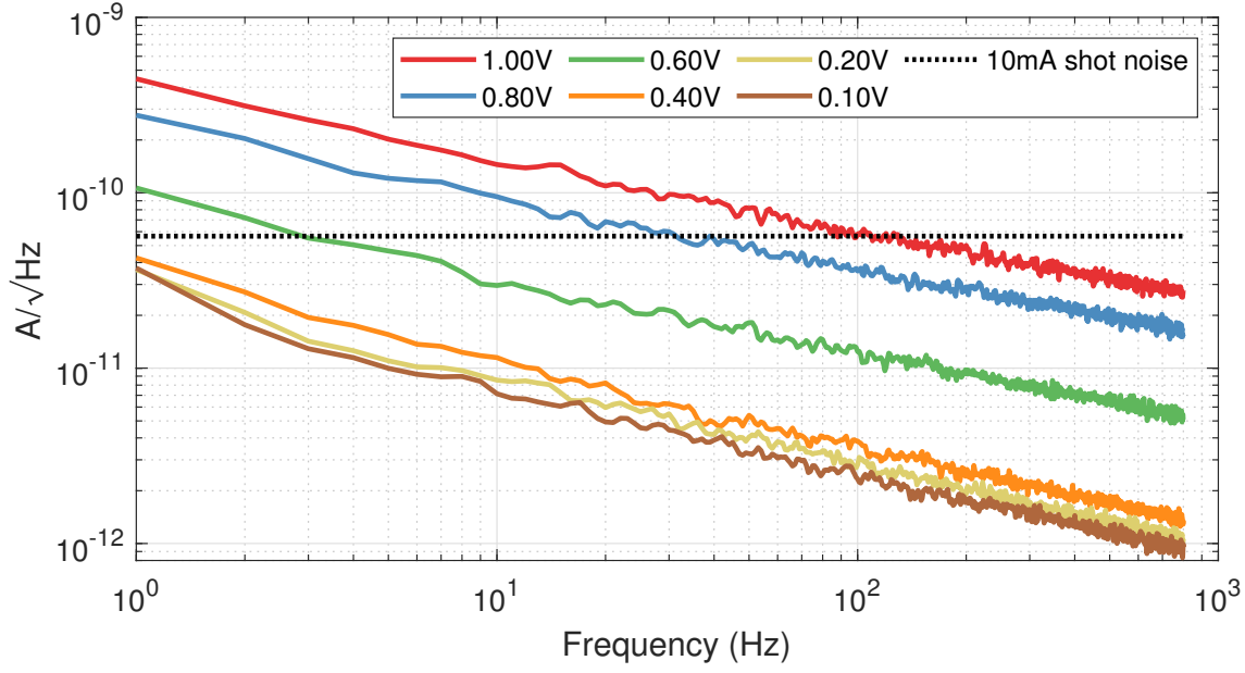
Figure A.5: Dark noise of the G12183-005k at 22°C for a series of reverse biases.
