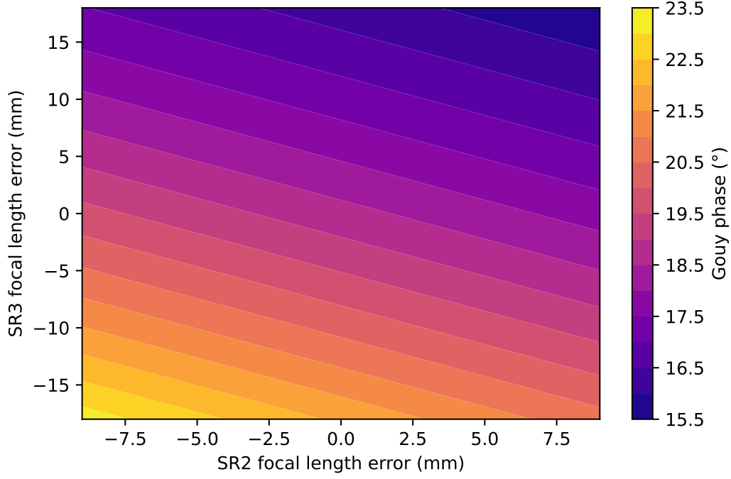
Figure 3.8: The Gouy phase between the ITMs and the SRM as a function of the error ( \pm 3\sigma ) in SR3 and SR2. When the SR3 focal length error > 6 mm and SR2 error is zero, the SRC is unstable (see Figure 3.10), so this area of the parameter space is unlikely to correspond to the beam at the SRM at LLO.
