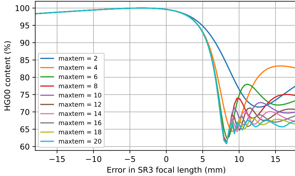
Figure 3.10: The percentage of HG00 light transmitted through the SRM as a function of SR3 focal length for the Michelson interferometer with Fabry-Perot cavities in its arms was simulated. Each simulation used a different maxtem command. The focal length of SR3 was changed. For focal lengths with a positive error greater than 7.5 mm, the cavity becomes unstable and FINESSE does not produce reliable results. For a stable SRC, the minimum number of TEM modes for sub 1% accuracy is six.
