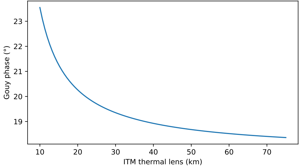
Figure 3.9: The Gouy phase between the ITMs and the SRM as a function of the thermal lens in the ITMs for the default values of SR3 and SR2. The nominal ITM thermal lens focal lengths are 50 km, and this corresponds to about 19°. More heating results in a greater thermal lens, however the LIGO detectors compensate for this with the thermal compensation system.
