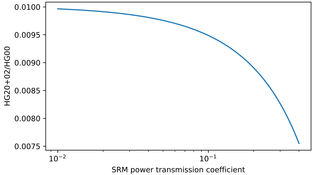
Figure 3.15: Ratio of HG20+02 to HG00 as the transmission of the SRM is increased for a mode mismatch between the arm cavity and the SRC. The interferometer is in RSE mode. A mode mismatch was introduced by setting the focal length of SR3 to be 12 mm shorter than the default amount.
