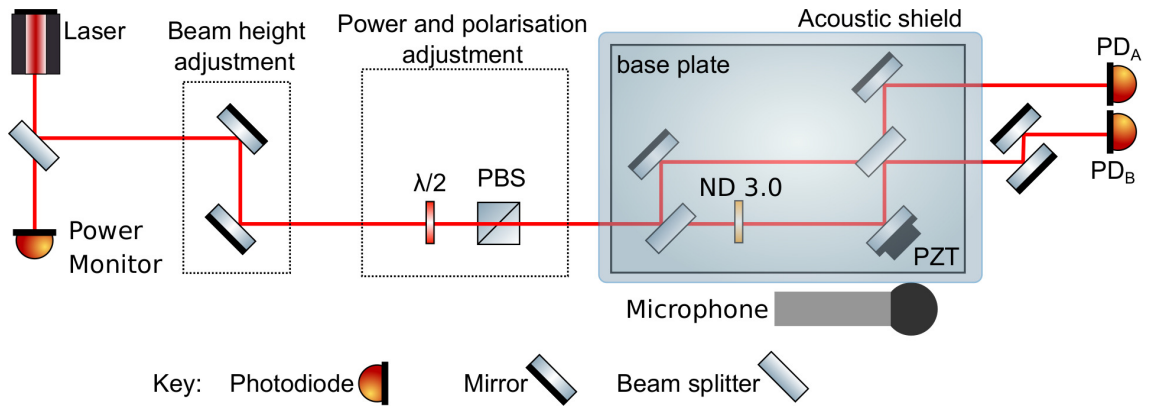
Figure 7.3: Sketch of the optical layout. The laser was generated by an NPRO. The power of the laser was monitored using a photodiode immediately after the laser. The beam's power and polarisation were controlled with a half wave plate and polarising beam splitter (PBS). The Mach-Zehnder was mounted on a base plate, and it was acoustically shielded by a plastic box and rubber feet. The splitting ratio of the BS2 was measured to be 50:50. An neutral density (ND) filter was used to decrease the power in one of the paths within the Mach-Zehnder.
