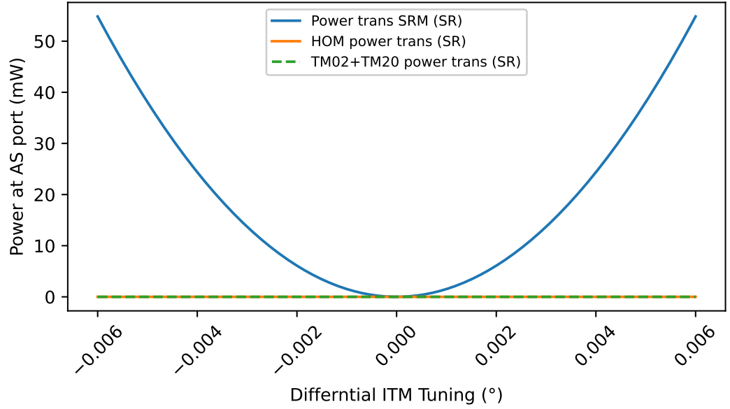
Figure 3.5: The minimum of the dark fringe is at 0^\circ differential ITM detuning, as shown by the blue line. A slight offset causes light to be at the AS port. This result was used to determine tunings for simulating what effect focal length errors in SR3 and SR2 have on the beam transmitted through the SRM. The orange line and dashed green line show that the beam has a negligible HOM content.
