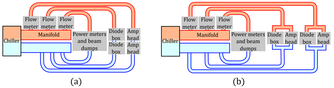
Figure 2.8: Cartoons of water cooling layout for the prototype laser. Panel (a): The laser will be run with the amplifier heads cooled in series with each other to reduce pointing noise. Panel (b): To perform the amplifier head temperature experiment, the water cooling was arranged so that the amplifiers temperature could be independently controlled.
