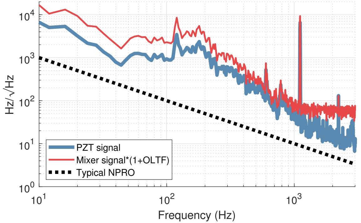
Figure 2.28: The mixer signal combined with the open-loop transfer function is shown in red. This is equivalent to the frequency noise of the system. The PZT signal should agree with this measurement below the unity gain point ( \sim 800 Hz). A signal was applied to the PZT at 1111 Hz. This is below the corner frequency of the PZT and above the unity gain point for the servo. This should match with the mixer signal. There is a factor of two between these two measurements. This can be attributed to imperfect calibration due to nominal parameters of the PMC being used. The typical noise expected from an NPRO is shown by the dashed black line. Between 100 Hz and 1000 Hz, there is a bulge in the frequency noise. This is likely due to acoustically driven noise of the PMC as the PMC is not vacuum sealed. This can be converted to length noise with a factor of \sim 10^{-14} m/Hz.
