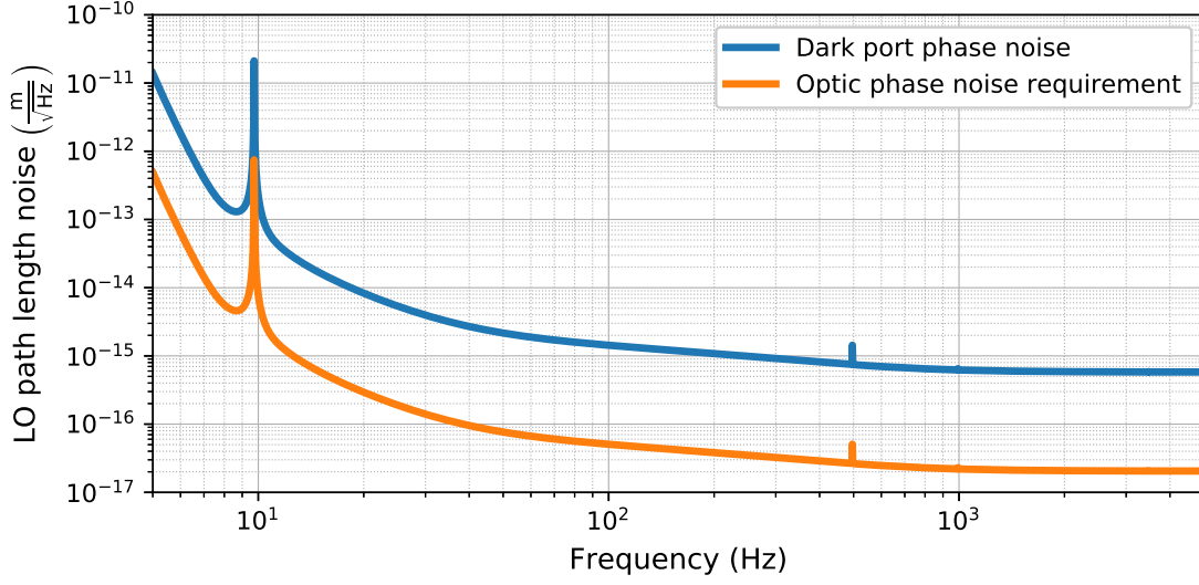
Figure 4.5: The sensitivity curve for A+ sets the limit on the amount of path length noise that is acceptable between the AS and LO beams. The blue line shows sensitivity curve in units of path length noise between the AS and LO beams, and the orange line shows the longitudinal motion requirement for the optics which combine the LO and signal beam. At 5 Hz, the longitudinal motion requirement for the optics is 4.9 \times 10^{-13} \text{ m}/\sqrt{\text{Hz}} .
