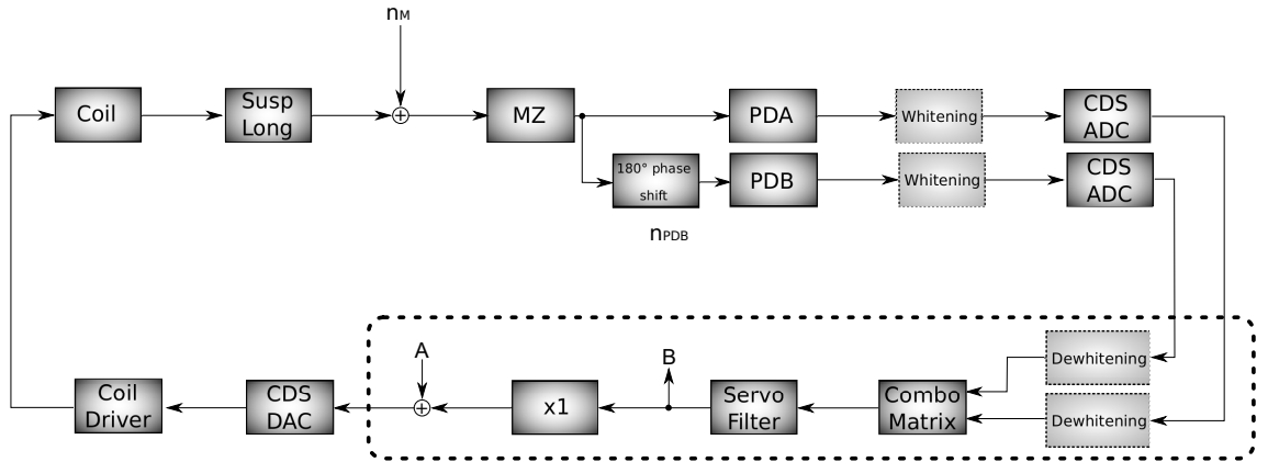
Figure 7.11: Flow diagram showing each block of the servo used to lock the in-vacuum Mach-Zehnder. The digital part of the servo is shown in the dashed area. The injection points A and B were used to calibrate the servo (see Figure 7.12) are around a times one block. The mirrors motion that the servo must correct for is represented by the signal n_M . The information about the Mach-Zehnder differential arm length is encoded by two signals that are 180^\circ out of phase. The whitening and dewhitening filters are paler as these do not affect the gain of the loop.
