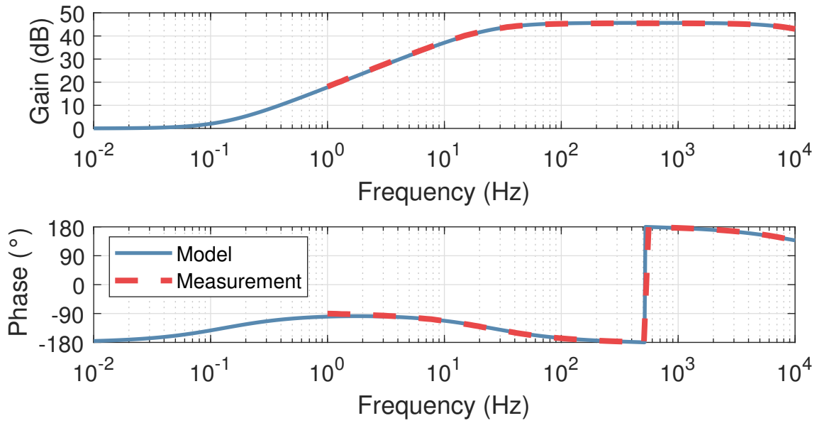
Figure 7.4: The transfer function of the electronics for sending, receiving and whitening the photodiode signal was modelled and measured. This gave the desired level of SNR to make shot noise limited measurements above \sim 200 Hz.
