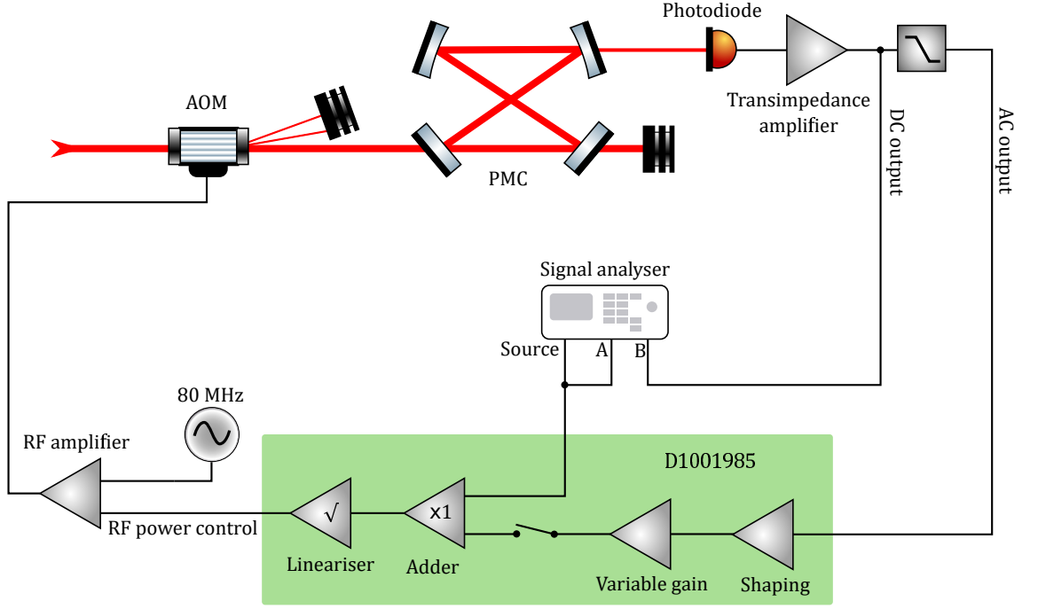
Figure 2.14: A sketch of how the AOM transfer function was measured. The components of the intensity stabilisation servo has also been shown. The PMC was locked and a signal analyser was used to perform a swept sine measurement. An IC (AD734) that performs a square root operation to an input signal was used to linearise the AOM's effect on beam power to an input signal. The transfer function was measured between the input to the lineariser and the photodiode used for the intensity stabilisation. The servo electronics are found in [120] and [121].
