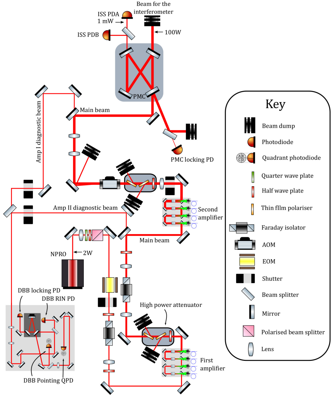
Figure 2.2: Sketch of the prototype optical layout for the PSL. The main and diagnostic beam paths are shown. This sketch shows all the optics in the main beam path as well as the pick-off points for the diagnostic beams. Within the diagnostic bread board (DBB) (grey box in the bottom left), there are several photodiodes for characterising beams.
