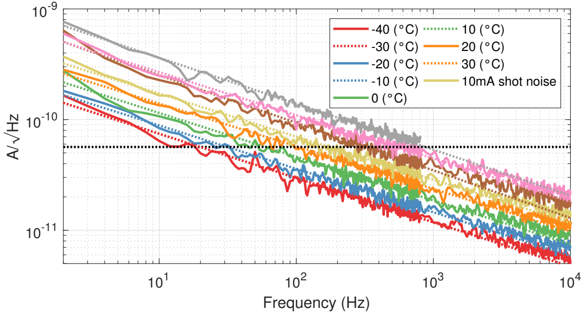
Figure A.8: The dependence of dark noise on temperature for the FD10D at 1.8V reverse bias.
