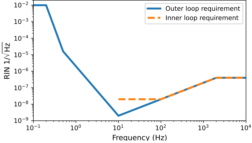
Figure 2.11: A reproduction of the intensity noise requirement from [95]. The outer-loop requirement is shown in blue and the inner-loop is shown by the dashed orange line. To lock the IMC, the inner-loop requirement must be met. Below 10 Hz, the motion of the test masses should be limited by seismic motion. An imbalance in the powers in the arm creates a coupling between laser intensity noise and differential radiation pressure noise, thus the laser's intensity needs to be stabilised such that motion induced by the laser's intensity noise is below the motion that is seismically driven. The requirement is most stringent at 10 Hz. The requirement relaxes above 10 Hz due to the PRC cavity pole. The inner-loop requirement is less extreme than the outer-loop as it is only used to stabilise the laser in the initial locking sequence.
