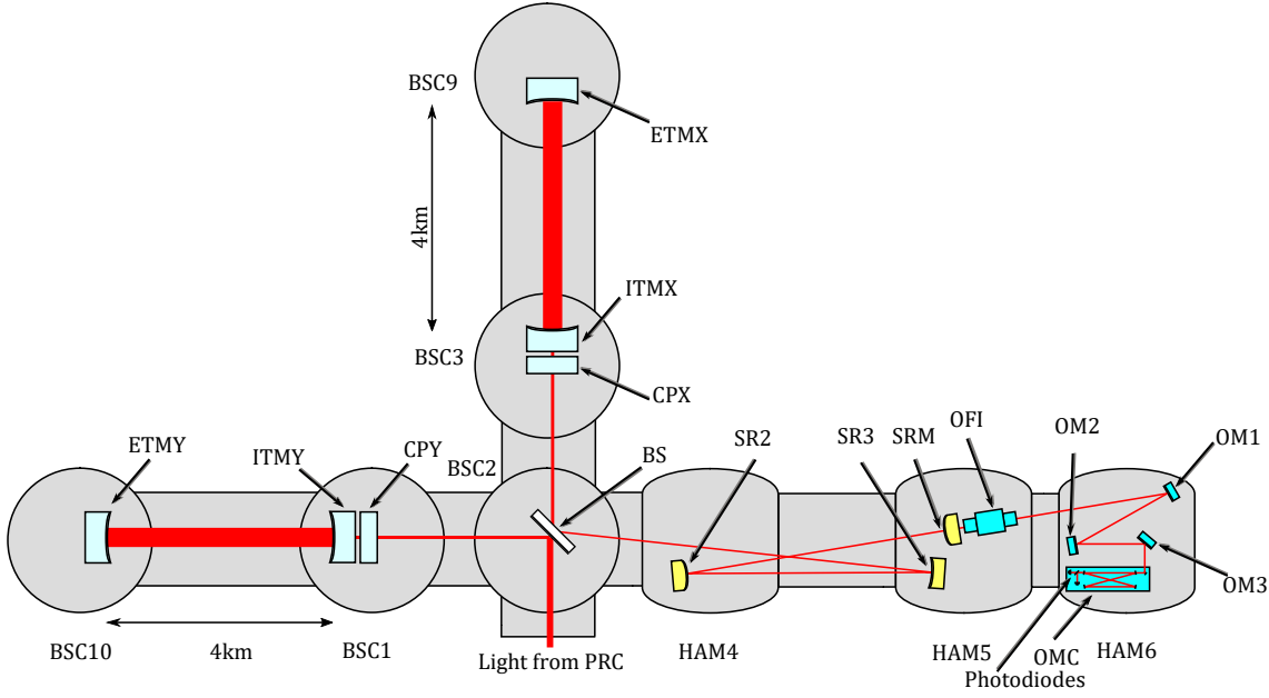
Figure 3.1: Sketch showing the parts of the aLIGO detectors discussed in this chapter. A more complete sketch is shown in Figure 1.4. The angles and lengths are exaggerated for clarity. Light from the arm cavities is incident upon the beam splitter (BS). As BS is wedged, the light going towards the SRC comes out at an angle. Differential arm length signals encoded onto this light are directed towards SR3, SR2, and then the SRM. Between the SRM and the OMC, there are optics for steering and mode matching (OM1-3). Finally, to strip away junk light, the light enters the OMC. The light emerging from the OMC is detected by photodiodes.
