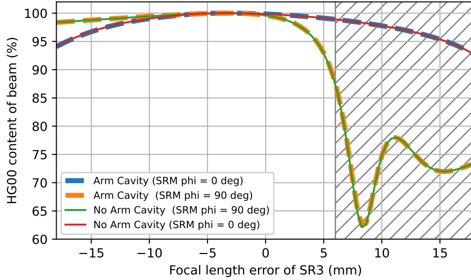
Figure 3.13: The percentage of light which is in the HG00 mode as the focal length of SR3 changes compared to the total light power does not depend on whether there are arm cavities. It is determined by the detuning of the SRM. The blue dashed line shows the behaviour of the beam with arm cavities present and with the SRC in signal recycling mode (SRM \phi = 0^\circ ). The red line shows how the beam changes with focal length error for a single-bounce measurement and with the SRC in RSE mode (SRM \phi = 90^\circ ). The orange dashed line corresponds to the interferometer having arm cavities and being in RSE mode (SRM \phi = 90^\circ ). The green line shows the behaviour of the beam when the interferometer is configured for a single-bounce measurement and is in signal recycling mode. The hatched region indicates where the SRC becomes unstable (see Figure 3.10), so the behaviour of the interferometer cannot be accurately simulated for these values of focal length.
