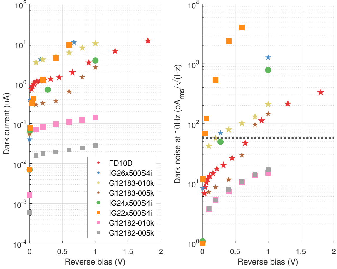
Figure 7.6: Left panel: the dark current for each photodiode was measured. Photodiodes of a similar cut-off wavelength share the same marker shape. The 1 mm photodiodes have larger markers than the 0.5 mm photodiodes. See Table 7.1 for information about the size and cut-off wavelength for each photodiode. Right panel: the dark noise at 10 Hz for each photodiode. The dashed line indicates the level of shot noise for a 10 mA current.
