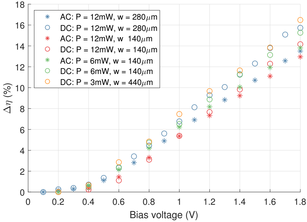
Figure 7.2: The FD10D's quantum efficiency depends on its reverse bias; the increase in quantum efficiency was 15 \pm 1\% when the bias was increased to the maximum value specified in its datasheet. Two types of measurement were used to determine the increase in quantum efficiency as the bias was increased. The first method was to measure the photocurrent with a voltmeter as the bias was increased, and the corresponding results are shown as circles ('DC'). The second method involved modulating the bias and measuring the resulting modulation in the photocurrent, i.e. an AC measurement, and these are shown by the stars. Each set of measurements was done with a different intensity by changing either the beam's width or power. Further detail on both methods is given in Section 7.4.1.
