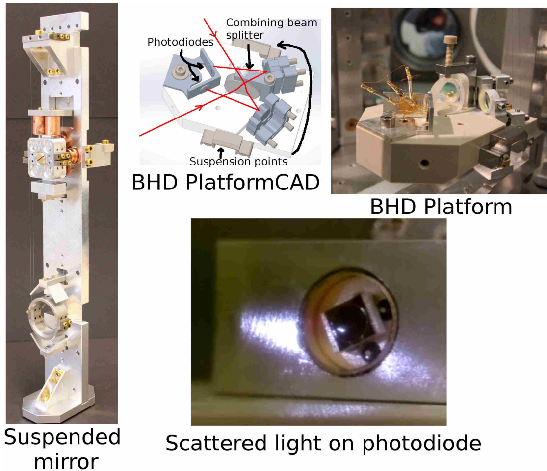
Figure 8.9: Photographs of the components used for the in-vacuum Mach-Zehnder. The scattered light originated from the uncoated back faces of the curved steering mirrors on the balanced homodyne detector platform. The design of the suspended mirrors is discussed in [207, Chapter 5]. The photograph was used by courtesy of Jan-Simon Hennig.
