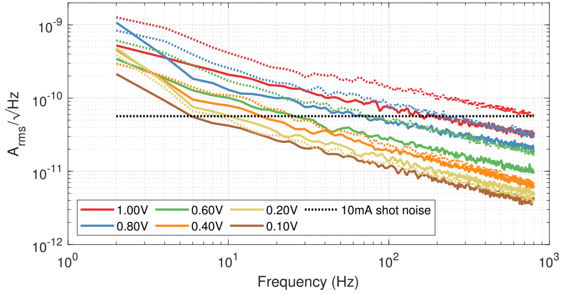
Figure A.4: G12183-010k.
