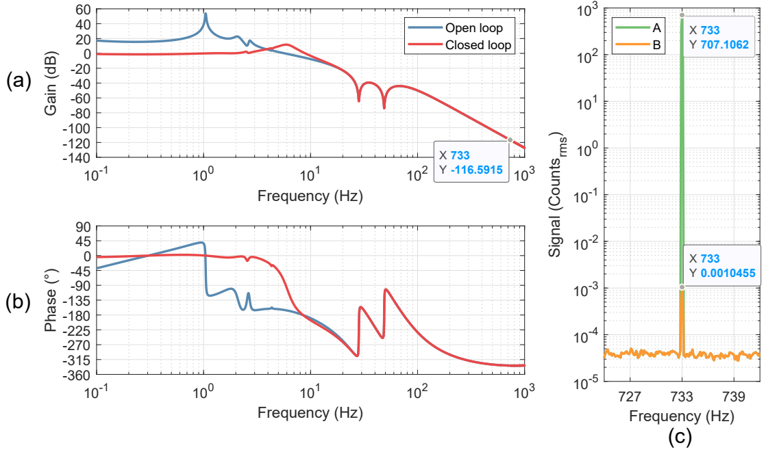
Figure 8.11: Panel (a) and Panel (b) show the Servo's open and closed-loop transfer function. This was calibrated using the factors from 8.1. Panel (c) shows a measurement where a signal was injected at point A in the servo and measured at point B (see Figure 8.10); these two points are separated by a times one block, and so the ratio of these signals represents the closed-loop transfer function of the servo. These measurements are in agreement with the model to within 0.1 dB.
