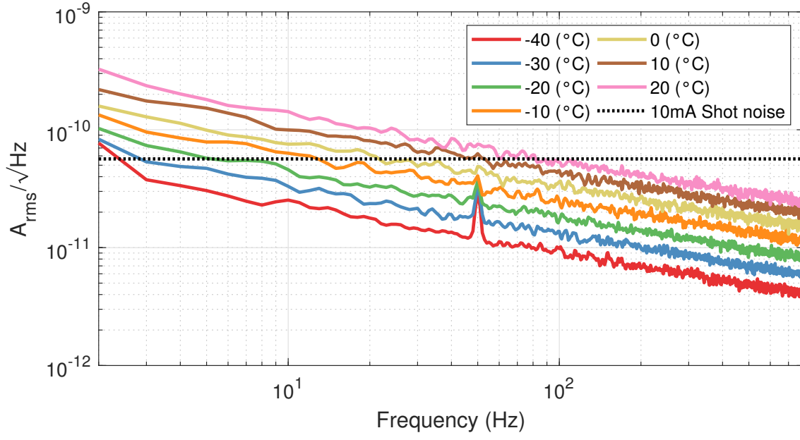
Figure A.3: G12183-005k 1.0V reverse bias
