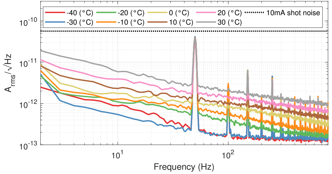
Figure A.5: G12182-005k 1.0V reverse bias
