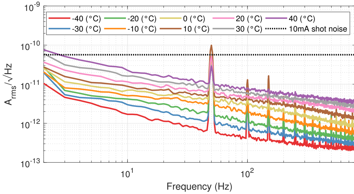
Figure A.4: G12182-010k 1.0V reverse bias
