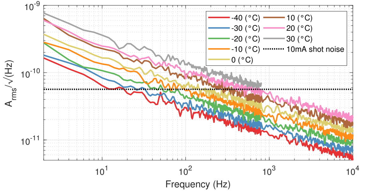
Figure A.1: FD10D 1.8V reverse bias
