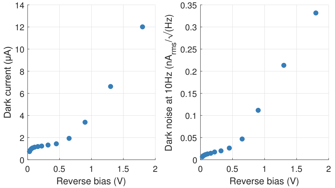
Figure 1.8: FD10D dark current and dark noise
