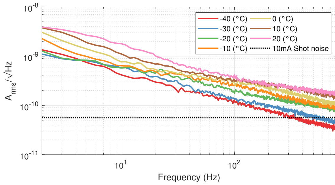
Figure A.7: IG26x500S4i 1.0V reverse bias
