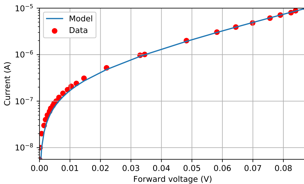
Figure 1.15: I_0 = (360 \pm 10) \text{ nA} , n = 1.02 \pm 0.01
