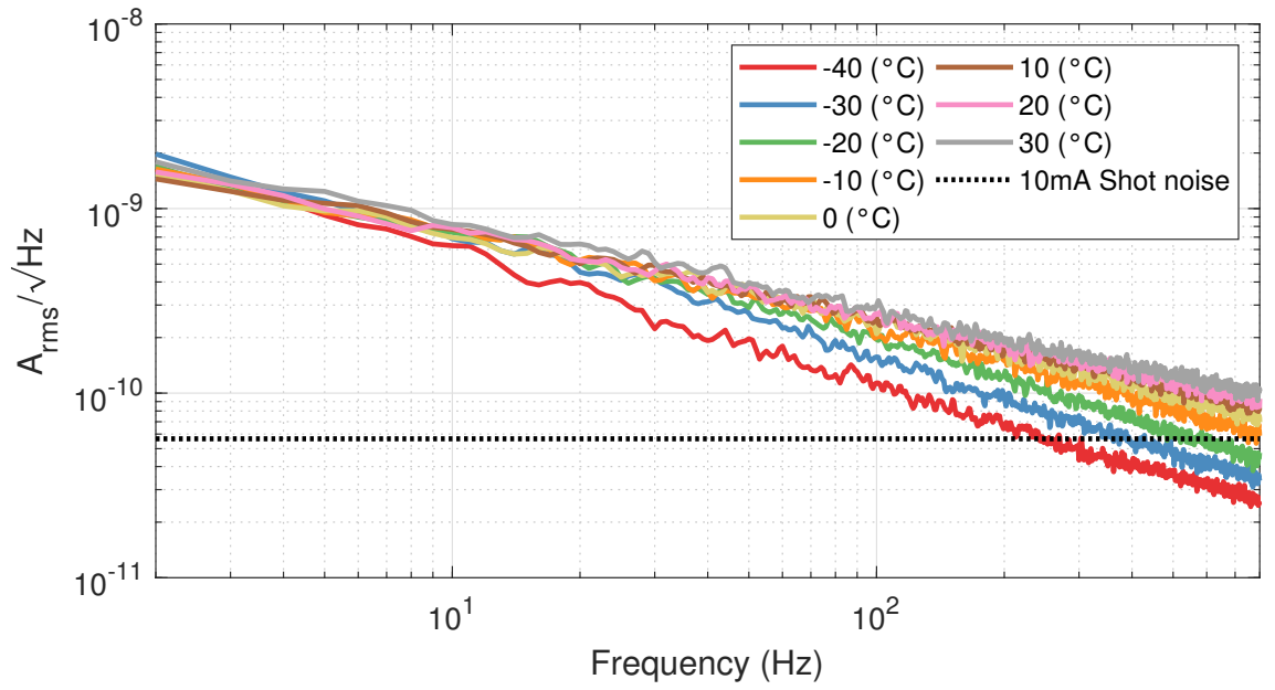
Figure A.6: IG24x500S4i 1.0V reverse bias
