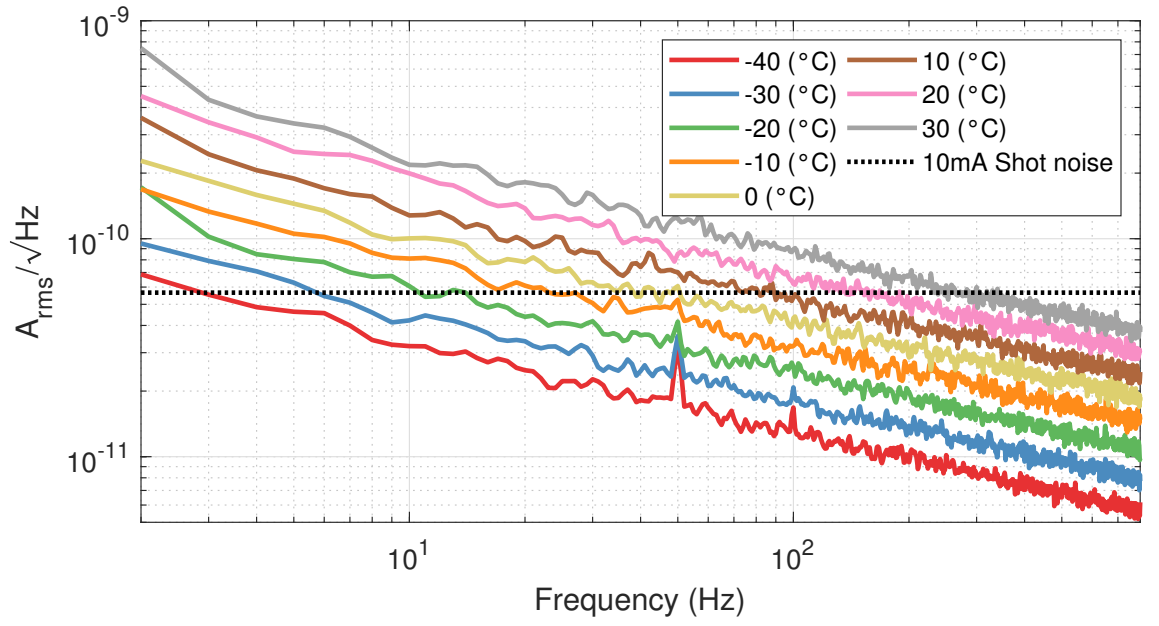
Figure A.2: G12183-010k 1.0V reverse bias
