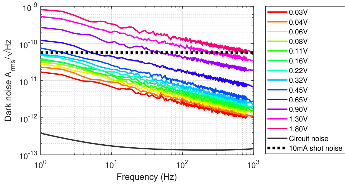
Figure 1.9: FD10D dark noise
