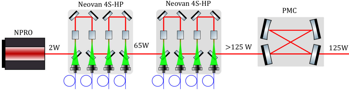
Figure 3.1: Conceptually, the PSL will be made up of four components: the NRPO, two neoVAN-4S-HP amplifiers and the PMC cavity. The NPRPO provides seed light with good noise characteristics. These noise characteristics are preserved by the amplifiers, so the resulting beam will have high power and low noise. The PMC filters junk light and RF intensity noise so a spatially pure mode can be sent to the interferometer.
