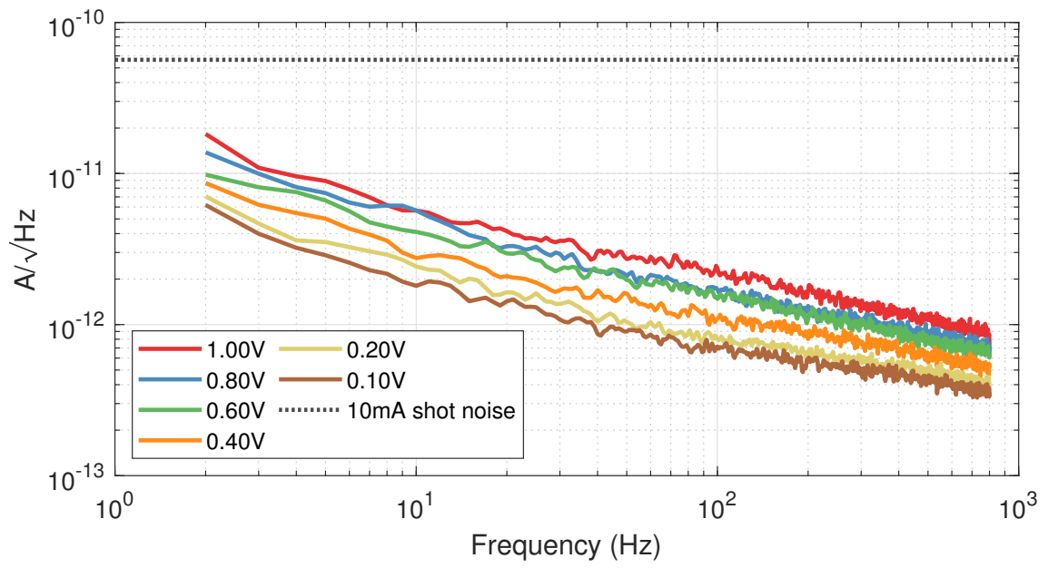
Figure A.7: Dark noise of the G12182-005k at 22°C for a series of reverse biases.
