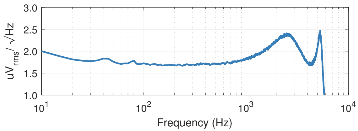
Figure C.1: Voltage noise at the input of the Glasgow CDS system
