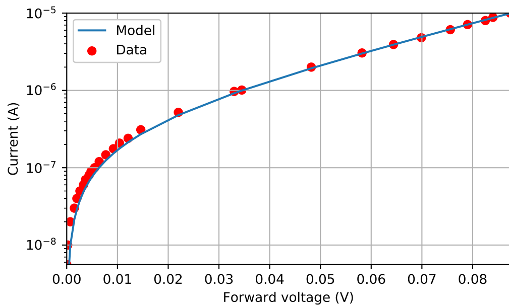
Figure 1.11: I_0 = (360 \pm 10) \text{ nA} , n = 1.02 \pm 0.01
