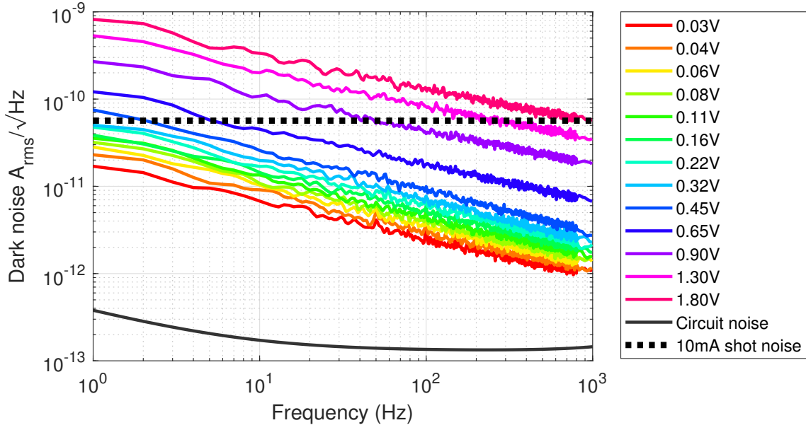
Figure 1.6: FD10D dark noise
