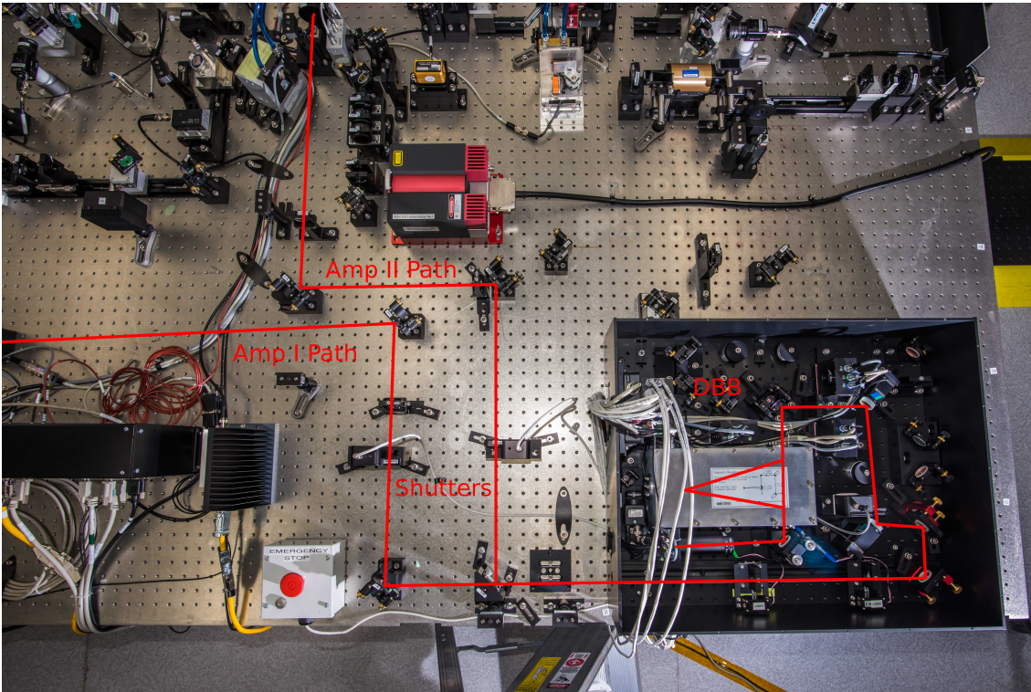
Figure 2.6: Photograph of the DBB and beam paths towards it.
