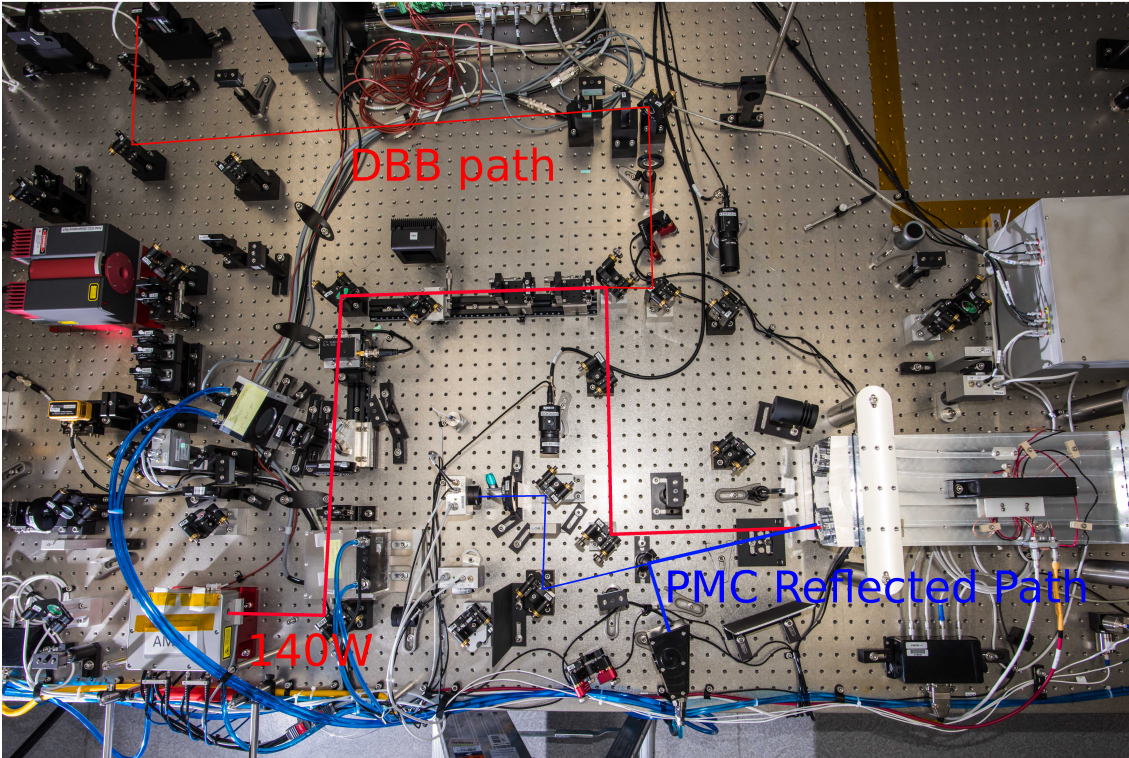
Figure 2.4: Photograph of the PSL prototype showing the beam path from the second amplifier (Amp I) to the input of the PMC. The path taken by reflected light from PMC used to lock the PMC can also be seen.
