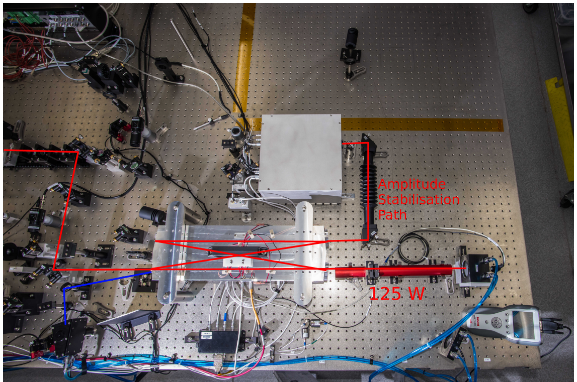
Figure 2.5: Photograph of the PMC and the inner ISS photodiode box.
