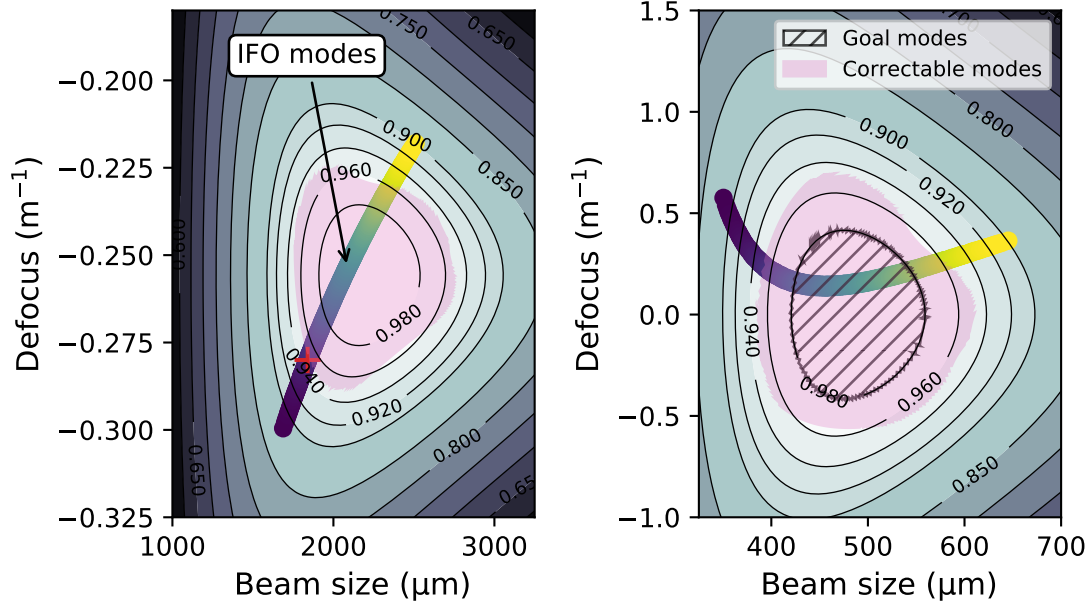
Figure 5.7: The region of WS space covered by the AWC in HAM6 if OMx1 and OMx2 for the layout discussed in Section 5.1. Left panel: the set of modes that is expected to be present at the SRM, as described in Chapter 3, is shown by the purple-blue-green-yellow curve. The pink region shows which modes that can be corrected for so that 98% mode-matching is achieved. The contours indicate the mode-matching between a mode (W, S) and the OMC mode. The red cross indicates the mode size that can be inferred from measurements of the SRC's Gouy phase at LLO. Right panel: this shows the same modes as the left panel, except they have been transformed by the optical layout to the plane of the OMC waist. Modes within the pink region can be actuated on so they move to the goal region, which is indicated with a hatched area.
