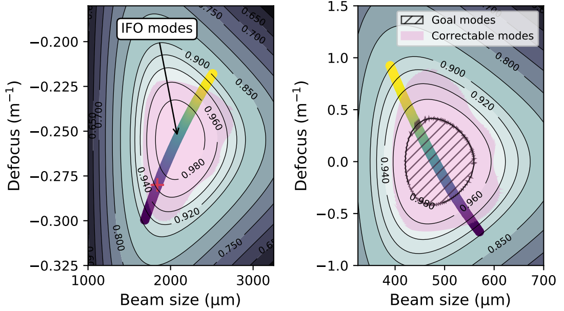
Figure 5.8: At the expense of orthogonality, the region of WS space covered by the AWC in HAM6 can be optimised by changing the Gouy phase separation between OMx1 and OMx2. Left panel: the set of modes that could be emerge from at the SRM, as described in Chapter 3, is shown by the purple-blue-green-yellow curve. The pink region shows which modes can reach 98% mode-matching by using the AWC in HAM6. The contours indicate the mode-matching between a mode ( W, S ) and the OMC mode. Right panel: this shows the same modes as the left panel; however, they have been transformed by the optical layout to the plane of the OMC waist. Modes within the pink region can be actuated on so they move to the goal region (hatched area).
