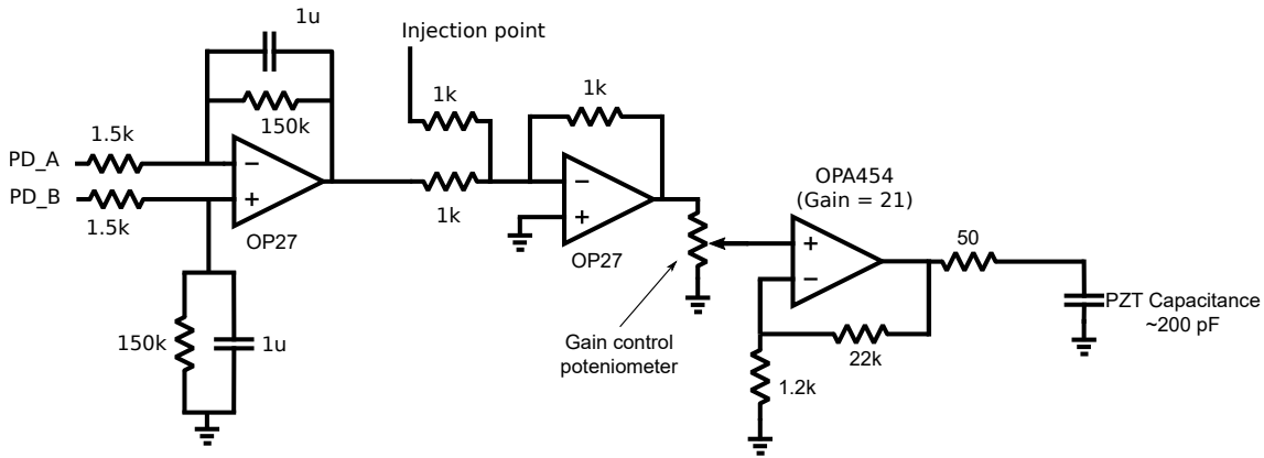
Figure 7.5: Circuit diagram for the electronics used to keep the in-air Mach-Zehnder locked to the middle of a fringe. The first stage subtracts the signals from the photodiodes and provides a 1 Hz roll-off. The second stage allowed for a signal to be applied to the PZT. The final stage boosted the signal to around 100V. The final resistor was used to prevent the OPA454 oscillating.
