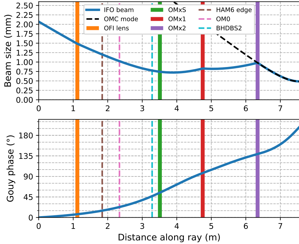
Figure 5.3: The top panel shows the radius of the beam as it travels from the SRM ( z = 0 ) to the waist of the OMC. Significant points along the axis are marked with vertical lines. Less significant, but useful, reference points are marked by dashed vertical lines. The bottom panel shows the Gouy phase shift accumulated by the beam as it propagates along the optical axis.
