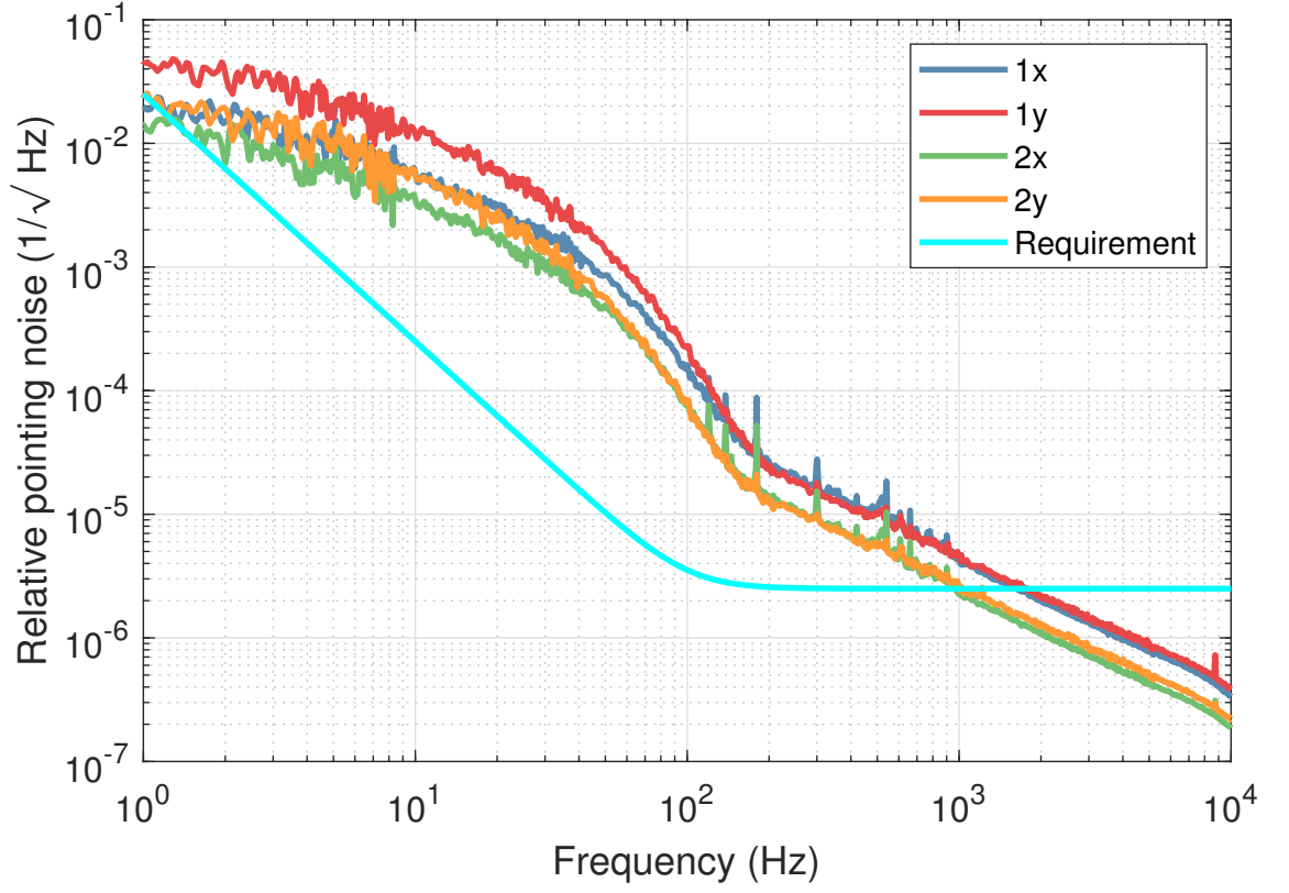
Figure 2.21: The four relative pointing degrees of freedom for the beam into the PMC was measured with the DBB. The requirement [123] is shown in light blue. The pointing noise is above the requirement, however the TnT lab has a higher amount of environmental noise than the PSL. Measurements below 200 Hz were be affected by scattering.
