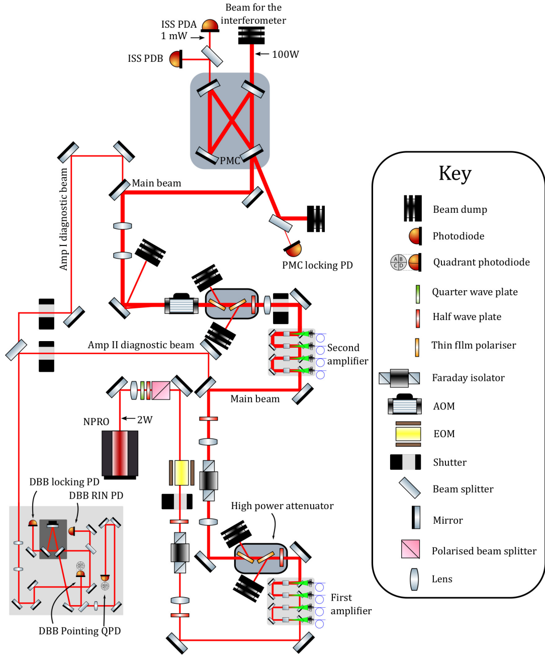
Figure 2.2: Sketch of the prototype optical layout for the PSL. The main and diagnostic beam paths are shown. This sketch shows all the optics in the main beam path as well as the pick-off points for the diagnostic beams.
