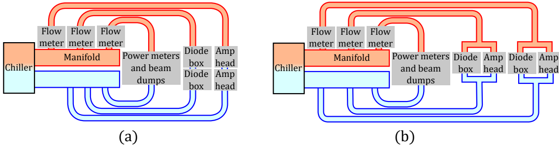
Figure 2.8: Cartoons of water cooling layout for the prototype laser. Panel (a): The laser will be run with the amplifier heads cooled in series with each other to reduce pointing noise. Panel (b): To perform the amplifier head temperature experiment, the water cooling was arranged so that the amplifiers temperature could be independently controlled.
