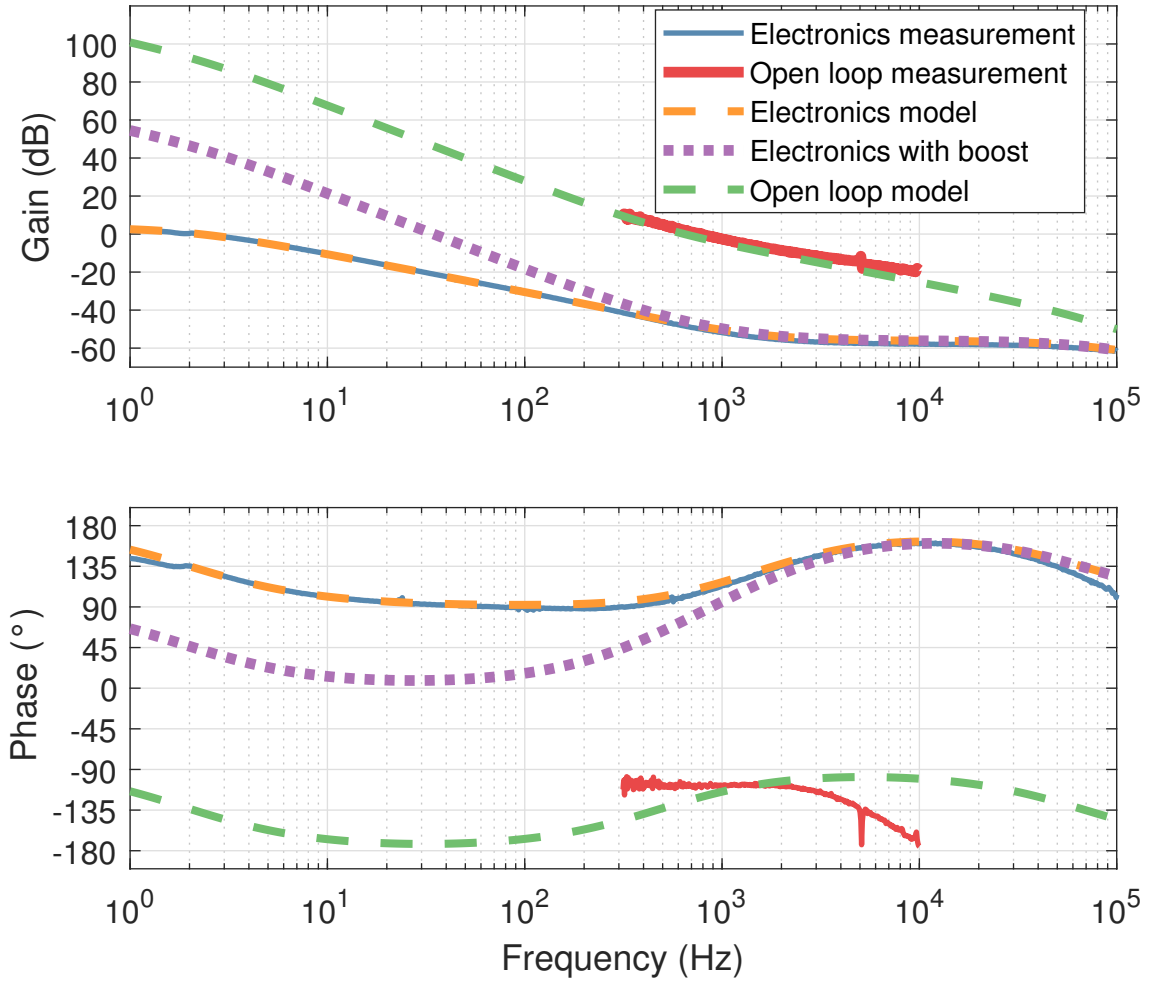
Figure 2.26: The open loop transfer function was measured using the layout shown in Figure 2.22. This is shown in red. The transfer function of the electronics without the ‘boost’ provided by an extra integrator stage was measured and is shown in blue. The model of this is shown in orange. The boosted electronics model is shown in purple. The green line shows the expected servo gain based on the boosted electronics model and the measurements shown in Figures 2.24 and 2.25. This model is within 2 dB of the measurement. The unity gain point was measured to be at \sim 800 Hz.
