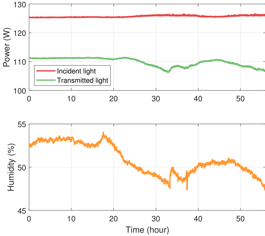
Figure 2.7: The top panel shows the power that was incident on the PMC and the power emerging from the PMC over a 55 hour trail run. The light produced by the amplifiers did not change significantly for the duration of this measurement, however the transmitted light through the PMC dropped from 111 W to, at its lowest, 107 W. This is likely due to the environmental conditions in the lab changing. The bottom panel shows the humidity of the lab. Changes in the humidity, which can be caused by a temperature change, coincide with changes in the power emerging from the PMC.
