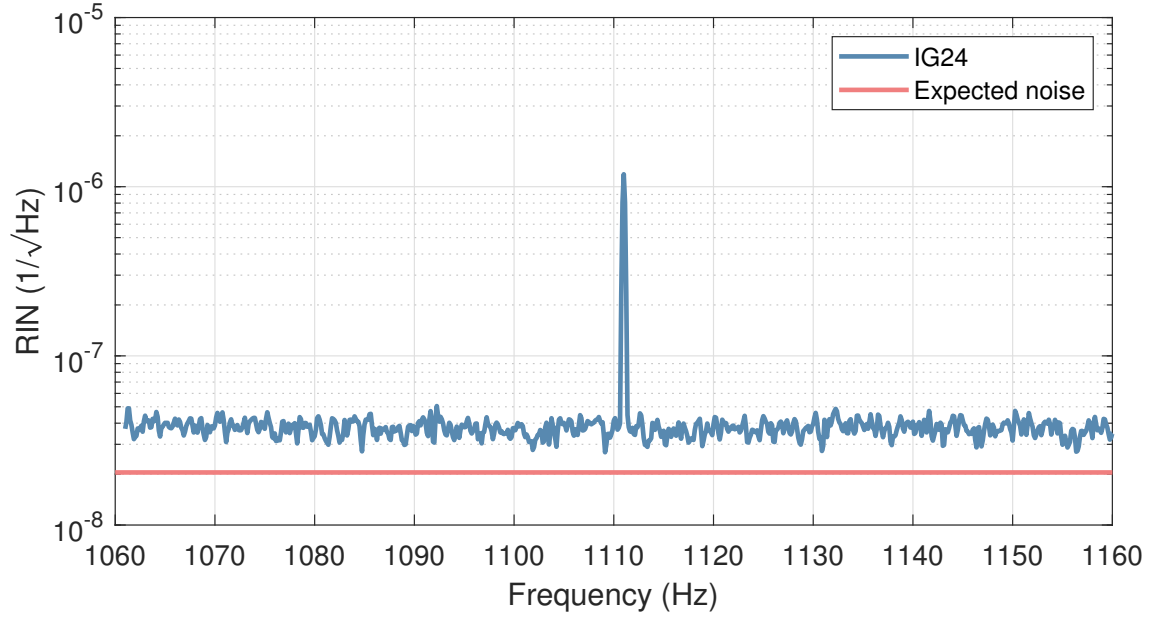
Figure 6.11: The noise of a 1.3 mA photocurrent made by the IG24x500S4i (blue) exceeded the expected amount (red) based on Equation 6.3 by a factor of 1.84. Note that the height of the 1111 Hz peak cannot be expressed in terms of amplitude spectral density units; however, this peak was measured to be the right level, so this beam was not saturating the photodiode.
