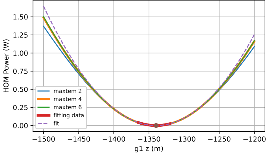
Figure D.1: Optimisation of parameters used in the gauss command to mode match the laser to the arms in the simulations described in chapter 3 and section D.3. The blue, green and orange lines show how the mode matching changes as the beam waist location is changed. As the mode matching becomes larger, more HOM are required, as the blue and green/orange lines diverge. A quadratic was fitted to the data highlighted in red, and the minimum value was used as the waist location parameter for the gauss command.
