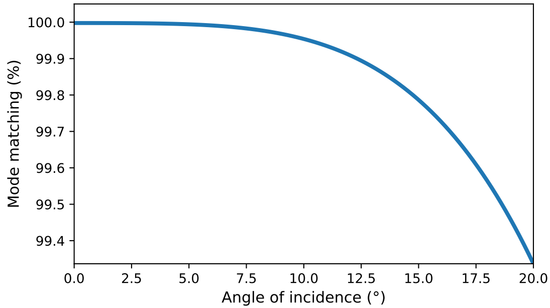
Figure 5.2: Astigmatism is a source of loss. When designing the layout shown in Figure 5.1, the AOI for the curved mirrors was altered to explore how sensitive it was to astigmatism. Using Equation (5.2), the loss was computed. This effect is negligible up to 10^\circ after which it starts to become significant compared to the losses summarised in Table 5.2.
