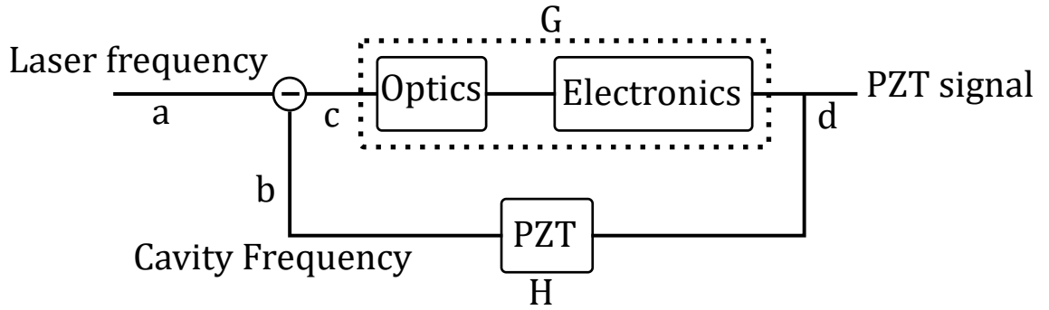
Figure 2.23: The servo can be considered as being made of three parts: the optics, the shaping electronics and the PZT. The transfer function of the optics represents how a difference in frequency between the laser and the cavity transforms into a signal after the demodulator. When at resonance and below the cavity pole, this is a flat transfer function that is proportional to the difference in frequency. Since this cavity pole is in the MHz region and this measurement will only go to the kHz region, the cavity pole can be ignored. The transfer function of the electronics includes everything after the demodulator up to and including the final high power OP amp. The PZT transfer function converts a voltage to a cavity frequency. The PZT acts as a low pass filter due to it having capacitance.
