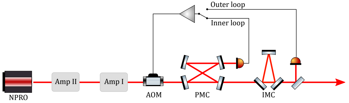
Figure 2.12: The intensity stabilisation concept involves two loops. The inner loop is responsible for stabilising the laser so that the IMC can lock. The outer loop is used to stabilise the laser for observation mode. The two loops sense the laser intensity noise at different points. The inner loop uses a low power beam, \sim 1 mW, transmitted by the PMC. The outer loop uses a higher power, \sim 350 mW, pick-off from the main beam. An AOM is used to actuate on the laser's power.
