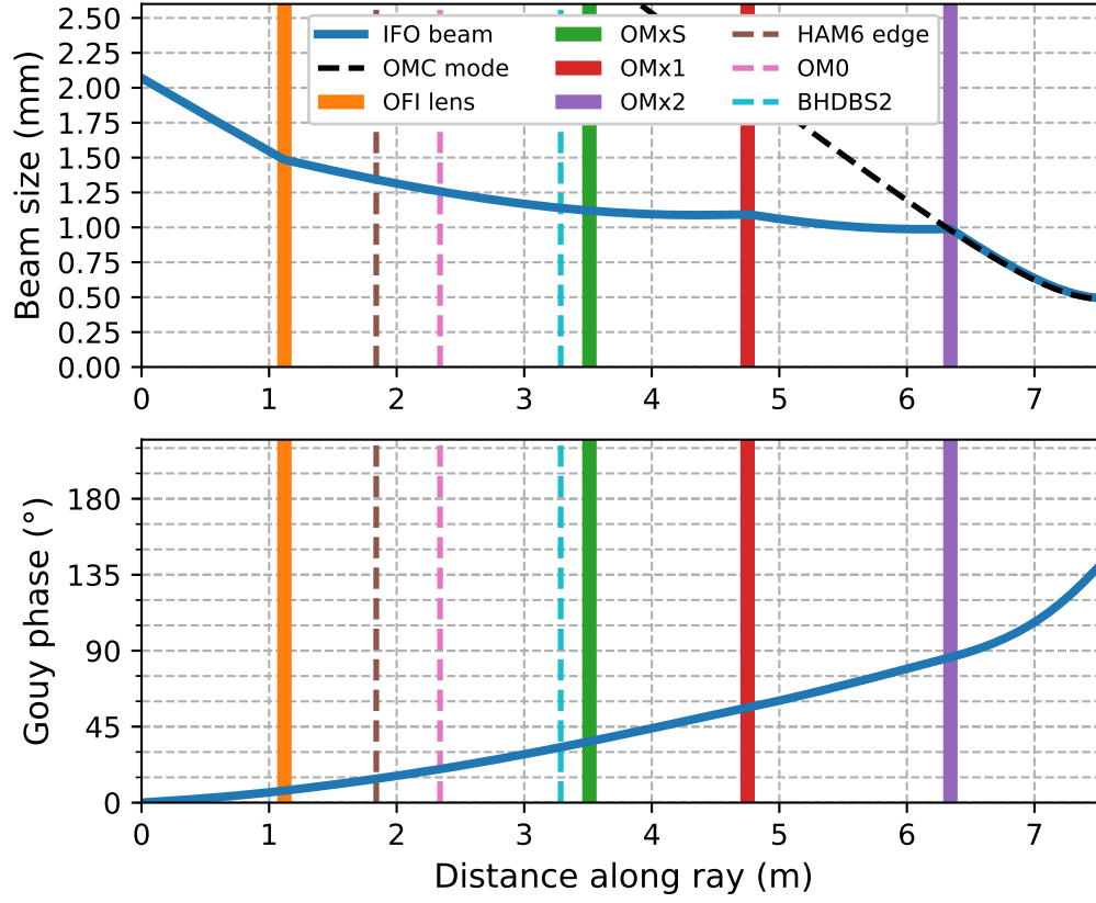
Figure 5.9: Top panel: the beam profile for the alternative layout of HAM6 suggested in Section 5.3.5. Bottom panel: The Gouy phase accumulated along the optical axis for the alternative layout. While alignment Gouy phase is degraded, the mode-matching Gouy phase was changed to bias the optical layout for correcting errors in the RoC of SR3.
