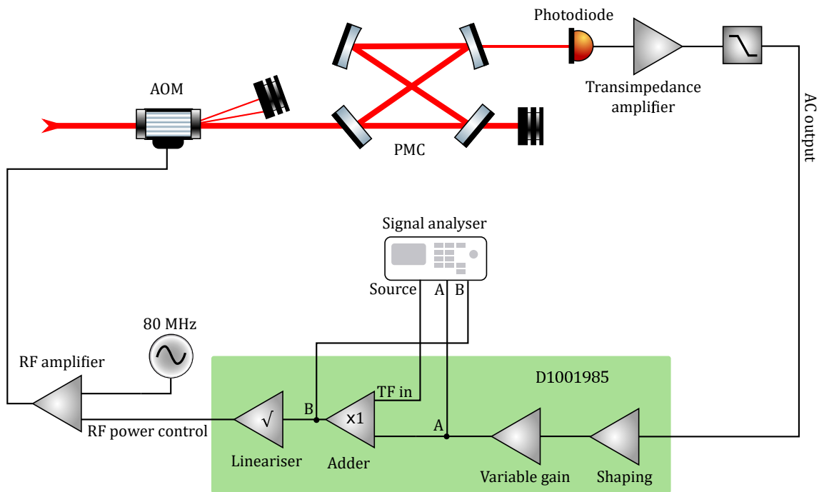
Figure 2.18: Sketch of the amplitude stabilisation servo. The open loop transfer function was measured by injecting a signal into a \times 1 adding stage and measuring the ratio of the signal immediately after and just before this stage.
