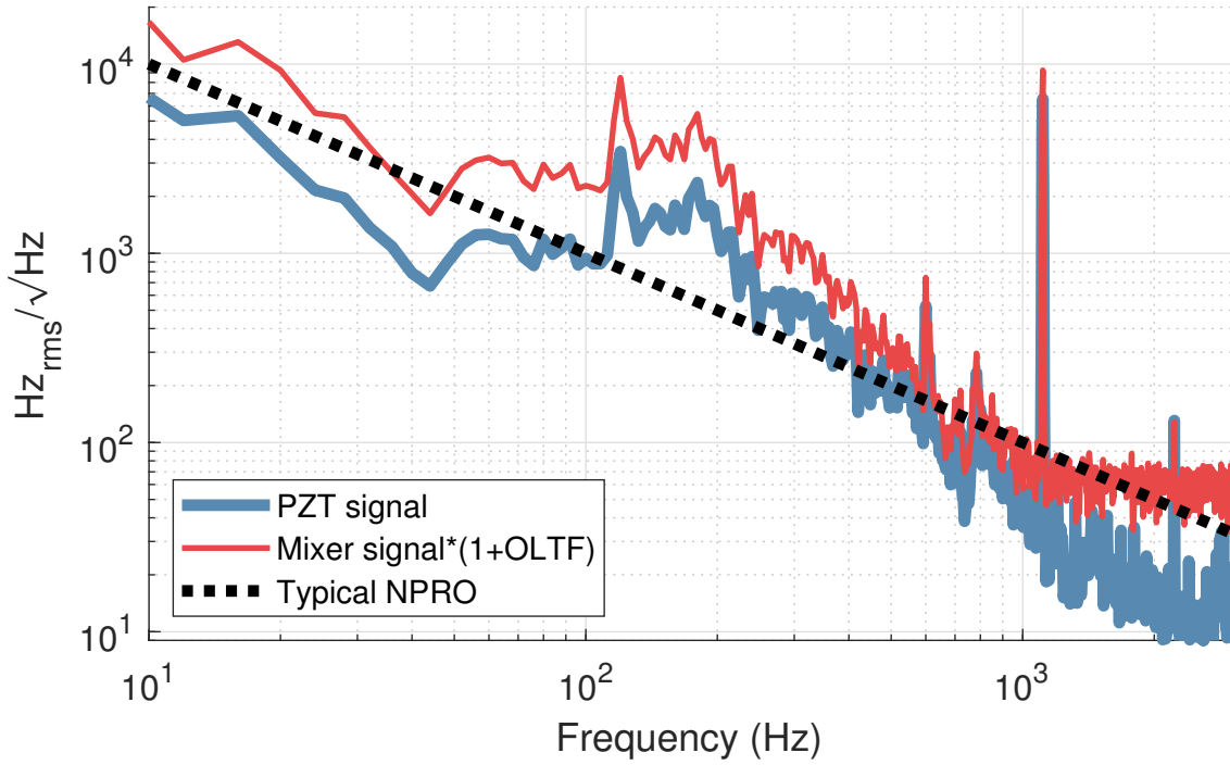
Figure 2.27: The mixer signal combined with the open loop transfer function is shown in red. This is equivalent to the frequency noise of the system. The PZT signal should agree with this measurement below the unity gain point ( \sim 800 Hz). A signal was applied to the PZT at 1111 Hz. This is below the corner frequency of the PZT and above the unity gain point for the servo. This should match with the mixer signal. There is a factor of two between these two measurements. This can be attributed to imperfect calibration due to nominal parameters of the PMC being used. The typical noise expected from an NPRO is shown by the dashed black line. Between 100 Hz and 1000 Hz, there is a bulge in the frequency noise. This is likely due to acoustically driven length noise of the PMC as the PMC is not vacuum sealed.
