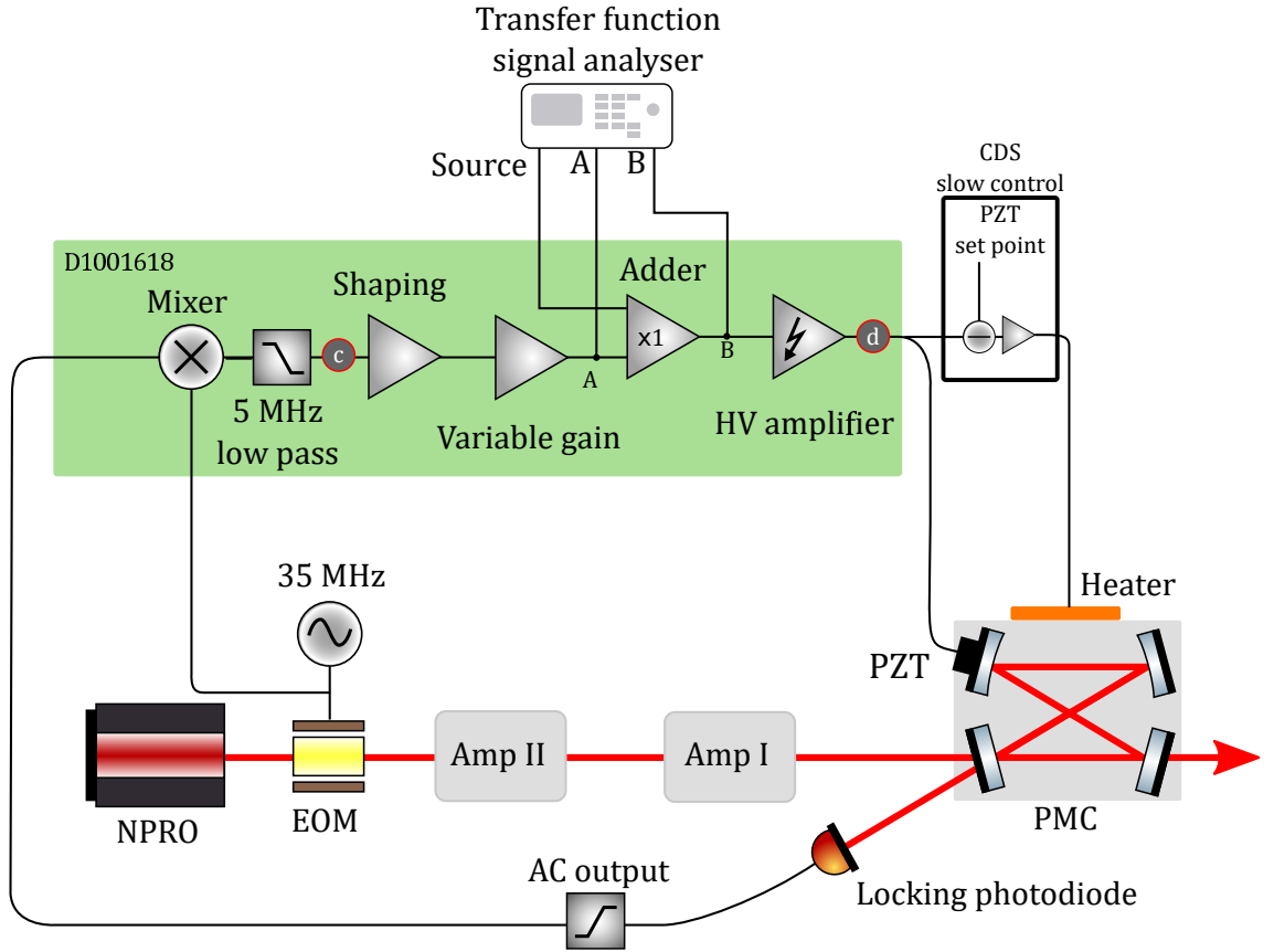
Figure 2.22: A sketch of the frequency stabilisation servo. An EOM creates 35 MHz sidebands which are used to produce a PDH locking signal. A PZT controls the length of the cavity at high frequencies. A heater and a digital loop is used to provide slow control that corrects for frequency drifts associated with change in the NPRO temperature and the room temperature. This is required as otherwise the PZT would run out of range. The open loop transfer function was measured using signals at A and B. The frequency noise was measured using the error point and control signals marked by c and d , with this notation corresponding with the notation in Figure 2.23 and Equation (2.1).
