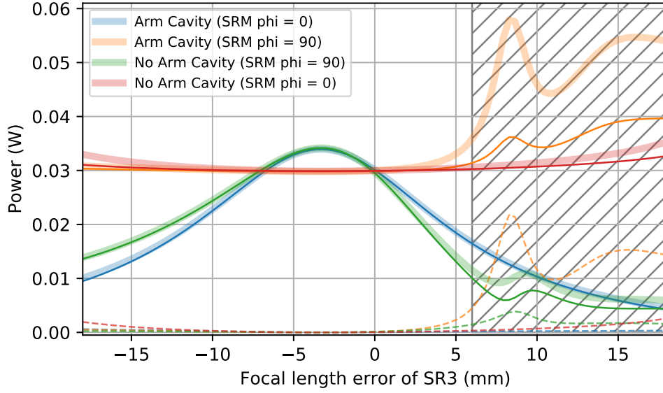
Figure 3.14: The total power transmitted through the SRM for each simulation is shown by the thick pale lines. The thin solid lines correspond to the power in the HG00 mode, and the thin dashed lines correspond to the power in the higher order modes. Blue lines show the behaviour when the interferometer has arm cavities and is in signal recycling mode, and the orange lines shows when it is in RSE mode. Green lines show how the power changes when the interferometer is configured for a single-bounce measurement and is in signal recycling mode, and the red line shows when its in RSE mode. The hatched region indicates where the SRC is becomes unstable, and so the behaviour of the interferometer cannot be accurately simulated for these values of focal length.
