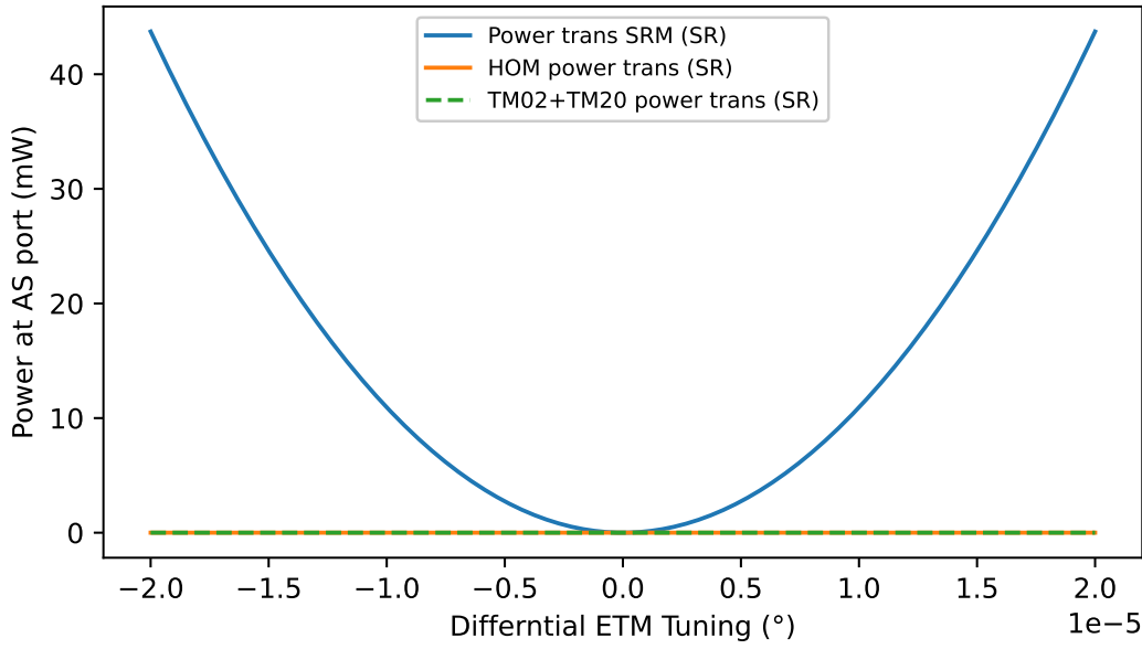
Figure 3.4: The minimum of the dark fringe is at 0^\circ differential ETM detuning, as shown by the blue line. A slight offset causes light to be at the AS port. This result was used to determine tunings for simulating what effect focal length errors in SR3 and SR2 have on the beam transmitted through the SRM. The orange line and dashed green line show the HOM content of the beam.
