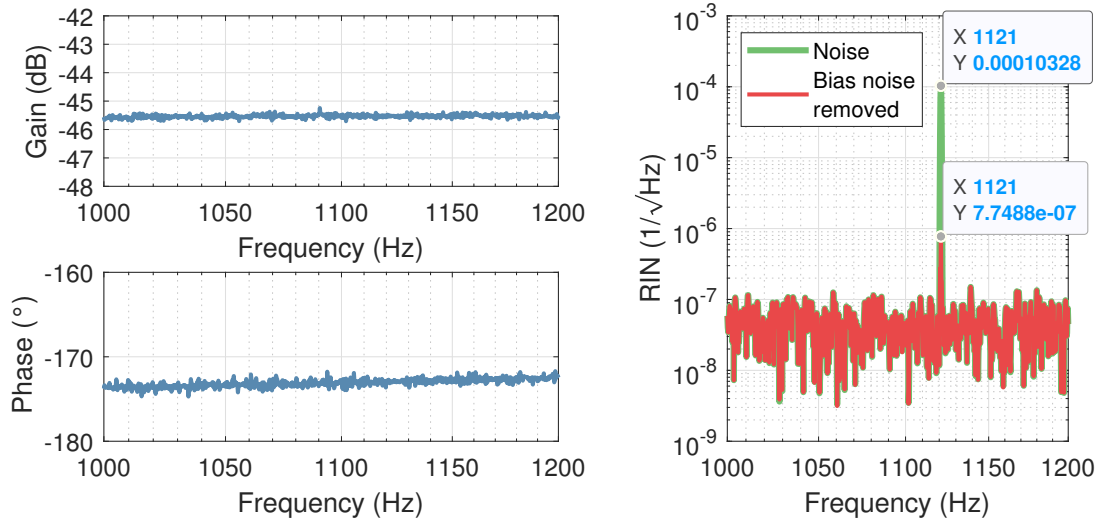
Figure 6.12: A noise projection measurement was performed to determine if the excess noise in the photocurrent produced by the IG24x500S4i (see Figure 6.11) was due to bias noise. The left hand panels show the Bode plot of the transfer function between the photodiode's cathode and the output of the transimpedance amplifier when the photodiode was producing 1.3 mA of photocurrent. The right hand panel shows the effect of subtracting bias noise from the signal at the output of the transimpedance amplifier. The peak at 1121 Hz was a modulation applied to the photodiode's cathode; 42.5 dB of this signal was removed by using the noise projection technique, and this is approximately the amount expected from the measured transfer function (45.5 dB at 1121 Hz). However, the level of the broadband noise remained unchanged thus indicating that the excess noise witnessed in the photocurrent produced by the IG24x500S4i was not due to bias noise.
