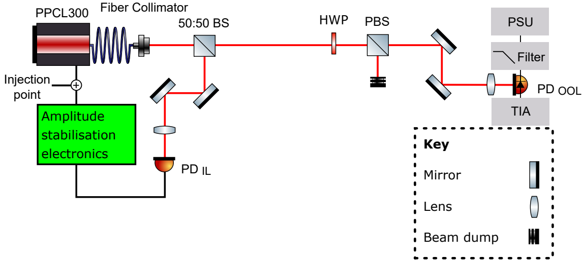
Figure 6.1: Optical layout used for measuring the effect that increasing the reverse bias of a photodiode had on its quantum efficiency and saturation limit. The out-of-loop photodiode, PD_{OOL} , was the photodiode under test (FD10D). A 1.55\ \mu\text{m} laser was used to assess the optical properties of the photodiode. A combination of half wave plate (HWP) and polarised beam splitter (PBS) allowed for the power of the beam to be set, and a lens was used to set the size of the beam on the photodiode under test. Amplitude stabilised light was needed to ensure the increase in photocurrent seen when the bias was increased was due to an improvement in quantum efficiency. The photodiode circuit (TIA) (see Appendix B.2) allowed for shot noise limited measurements of current around 10 mA and for the bias to be selected. The calibration signal was added onto the amplitude stabilisation error signal.
