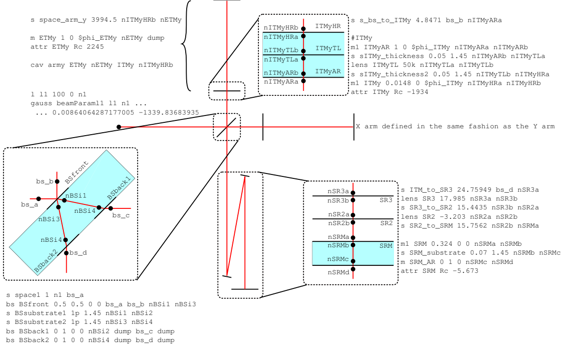
Figure 3.3: Schematic of the simulation. The dimensions of the schematic are not to scale. The laser light is shown as a red line. Black lines with red beams interacting with them corresponds to components such as mirrors and lenses. Important nodes are highlighted with black dots and the associated FINESSE commands are shown nearby. Zoom-ins provide more detail for the main beam splitter, ITMy and the SRC. The elongated curled bracket highlights the arm cavity, and the text with it shows how it is implemented in FINESSE.
