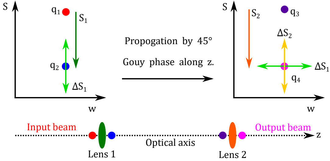
Figure 5.5: Sketches of the WS representation for a Gaussian beam interacting with different parts of a simple optical layout consisting of two active lenses with powers S_{1,2} \pm \Delta S_{1,2} . The left hand axes shows the WS plane at Lens 1. The input beam, q_1 , is indicated by a red dot, and the effect of the lens on q_1 is shown by the dark green arrow S_1 . This results in a new mode q_2 which is shown as a blue dot. A light green arrow indicates the actuation of Lens 1. The right hand axes shows the WS plane at Lens 2. The input mode at Lens 2, q_3 , is shown as a purple dot, and the output mode, q_4 , is shown as a pink dot. The static and dynamic power of Lens 2 is indicated by the orange and yellow lines. As Lens 1 and Lens 2 are separated by 45^\circ of Gouy phase, the actuation provided by Lens 1 results in a change in the beam parameter which is orthogonal to the actuation provided by Lens 2, provided that the actuations are small enough. Beneath the two WS space diagrams is a sketch of the optical axis and the location of the modes.
