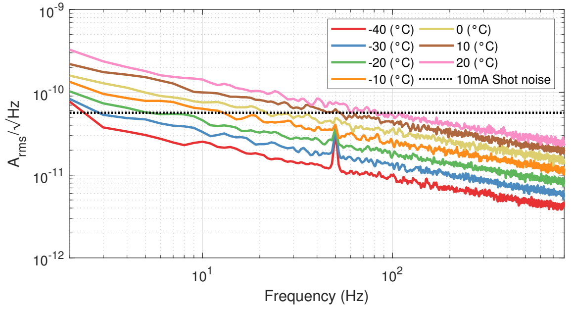
Figure A.10: G12183-005k at 1.0V reverse bias.
