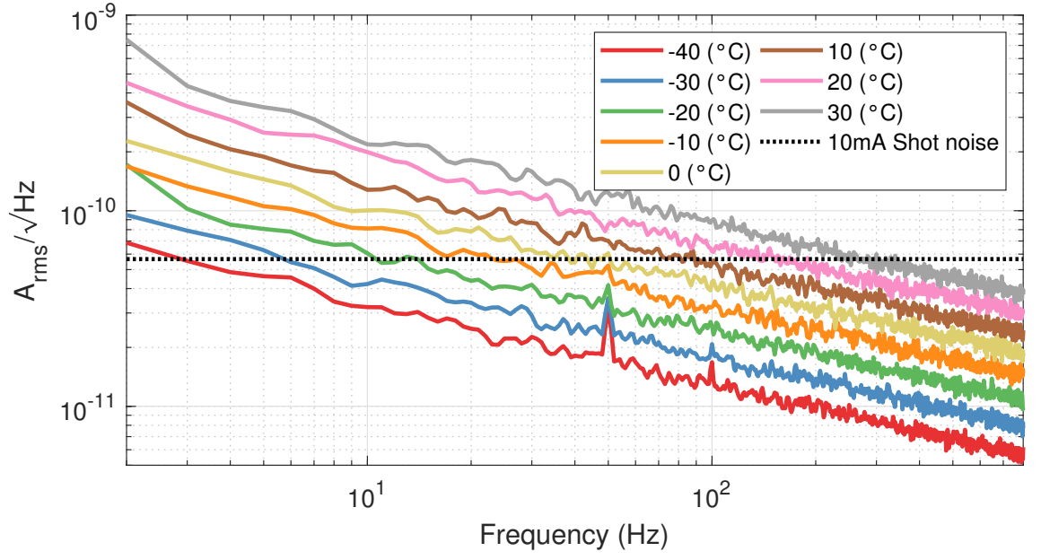
Figure A.9: G12183-010k at 1.0V reverse bias.
