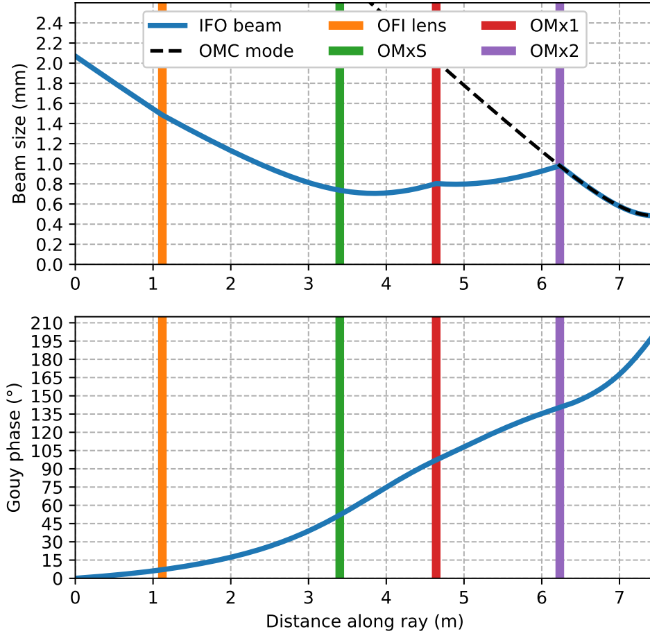
Figure 1.7: The radius of the beam as it travels from the SRM ( z = 0 ) to the waist of the OMC.
