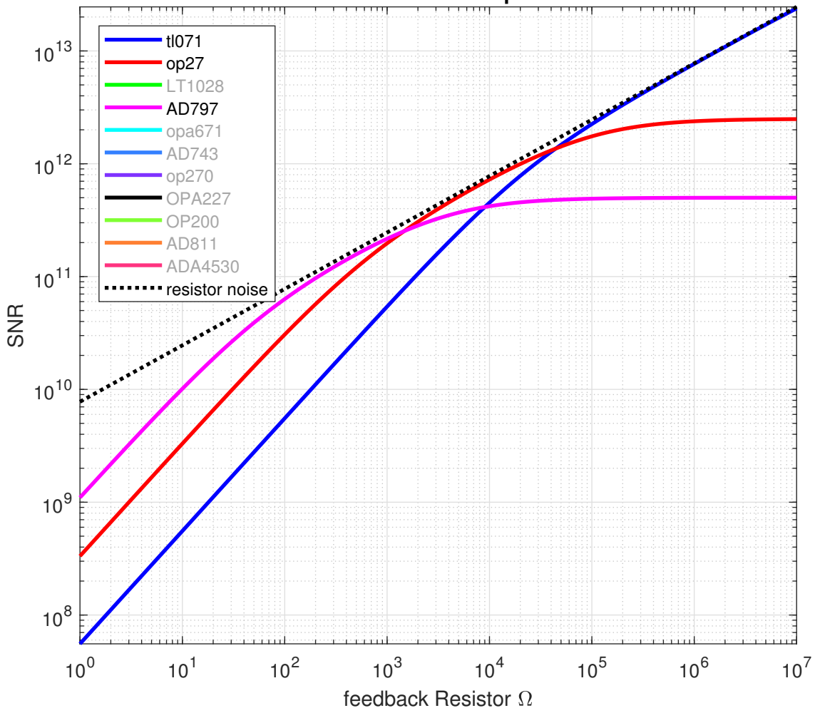
Noise of various OP amps at 1kHz
