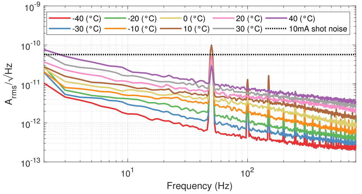
Figure A.4: G12182-010k 1.0V reverse bias
