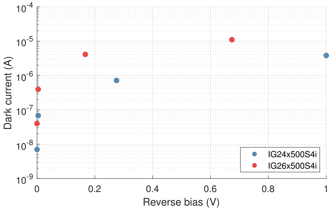
Figure 1.8: The IG26x500S4i has an order of magnitude more dark current in compared to the IG24x500S4i at similar reverse biases. The measurement at 1V reverse bias for the IG26 saturated the transimpedance amplifier.
