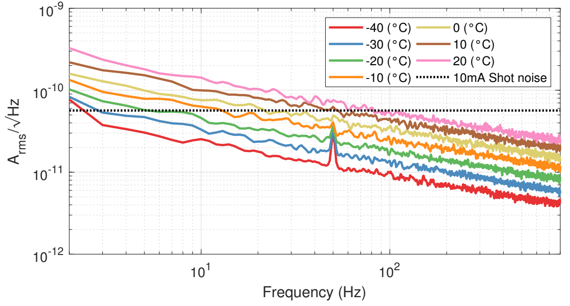
Figure A.3: G12183-005k 1.0V reverse bias
