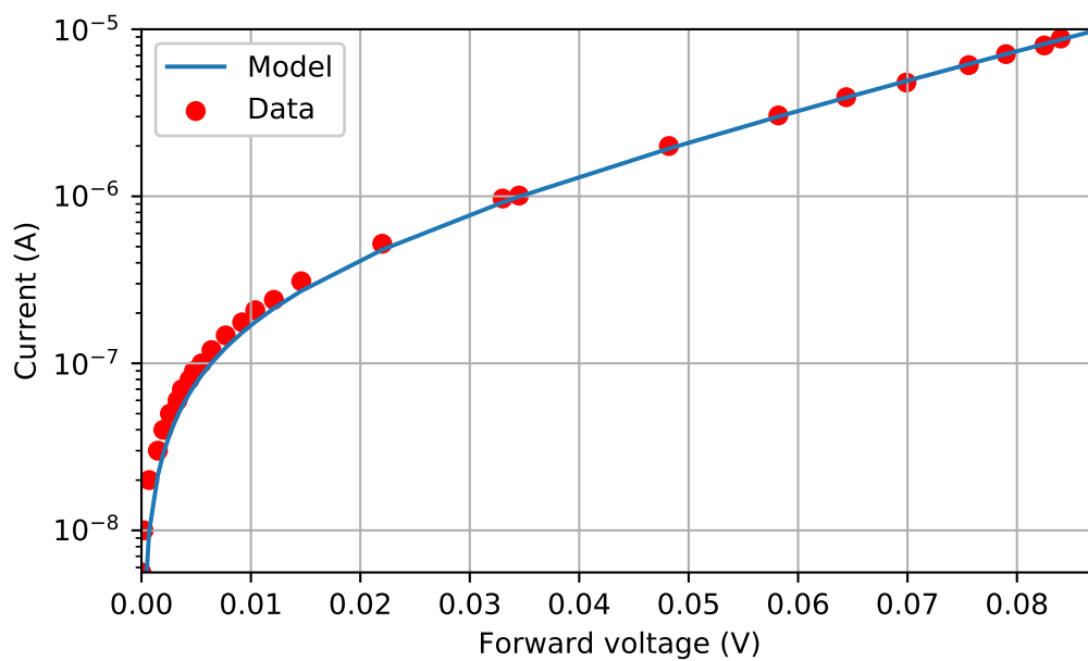
Figure 1.13: I_0 = (360 \pm 10) \text{ nA} , n = 1.02 \pm 0.01
