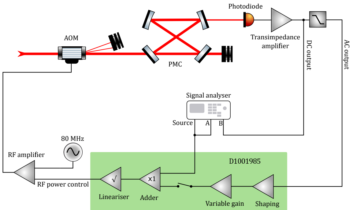
Figure 2.14: A sketch of how the AOM transfer function was measured. The components of the intensity stabilisation servo have also been shown. The PMC was locked and a signal analyser was used to perform a swept sine measurement. An IC (AD734) that performs a square root operation to an input signal was used to linearise the AOM's effect on beam power to an input signal. The transfer function was measured between the input to the lineariser and the photodiode used for the intensity stabilisation. The servo electronics are found in [127] and [128].
