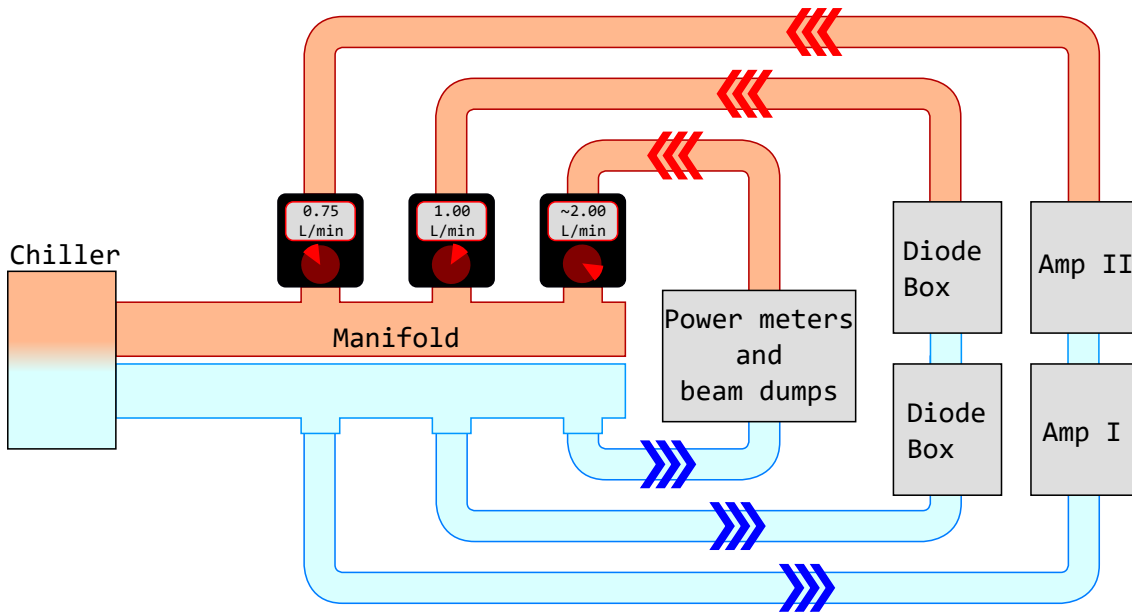
Figure 2.8: Cartoon of the cooling layout for the PSL. The amplifiers are on a separate loop to the diode boxes so that the flow rates for these can be reduced as much as possible. By placing the flow rate sensors on the return side of the the cooling system, leaks can be detected.
