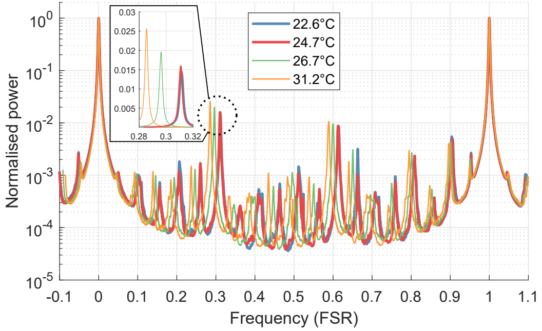
Figure 2.10: Mode scans were performed with the DBB for each amplifier head temperature. The second order mode for this cavity is located at \sim 0.3 FSR. As the temperature of the amplifier head changes, the second order mode content of the beam changes on the percent level. This second order mode height is shown in the inset. The second order mode can change due changes in the thermal lens focal length or because the beams astigmatism changes.
