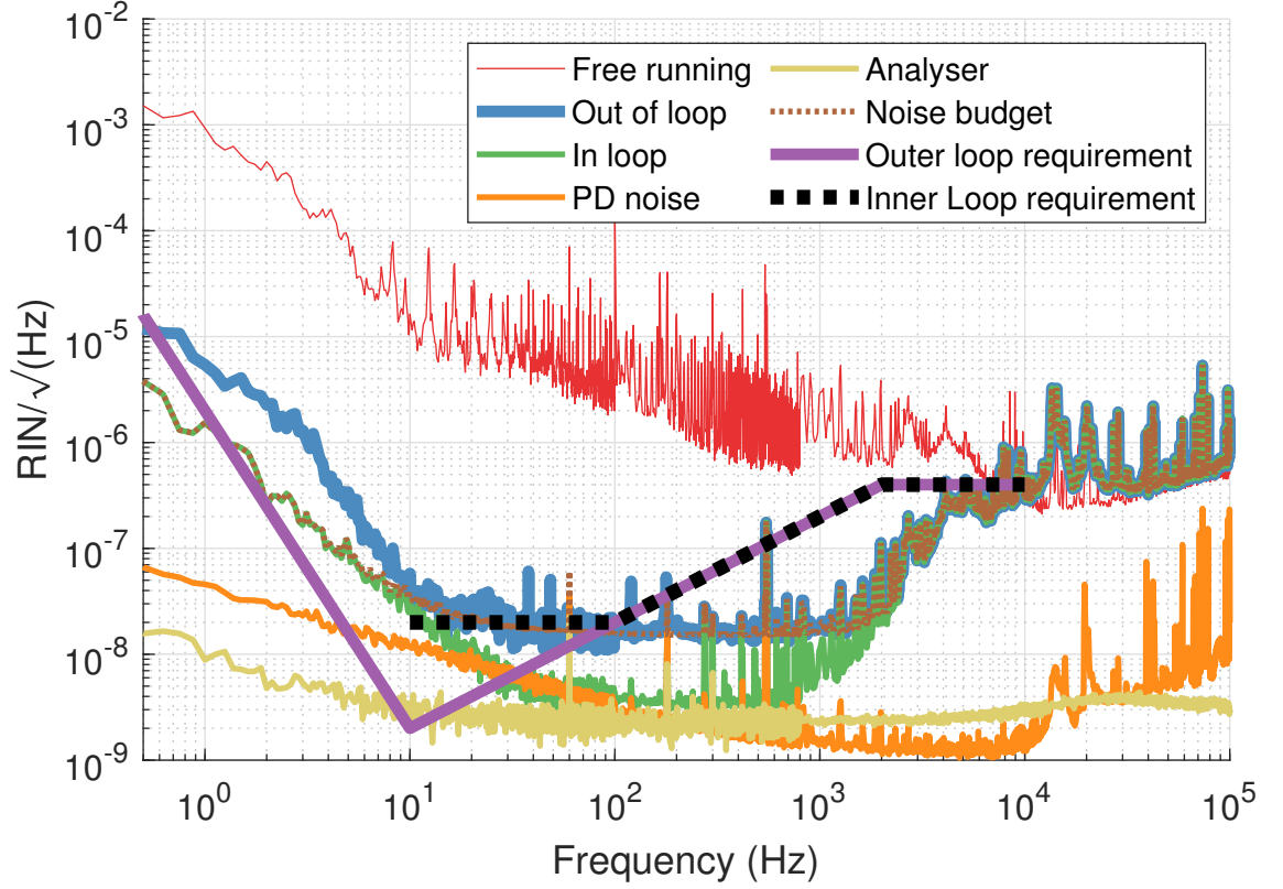
Figure 2.20: The Free running noise of the laser is shown in red. The noise of the light transmitted by the PMC is shown in blue; this meets the requirement that is shown by the dashed black line. The noise level is determined by the in loop noise, shown in green, the shot noise and other technical noise sources. The sum of these is shown by the dotted brown line. Below 100 H the noise is shot noise limited. There is a discrepancy between the noise budget and the measured noise. This is likely due to dust falling through the beam or scattered light. Near the unity gain point of the servo, the noise is enhanced by the servo due to gain peaking.
