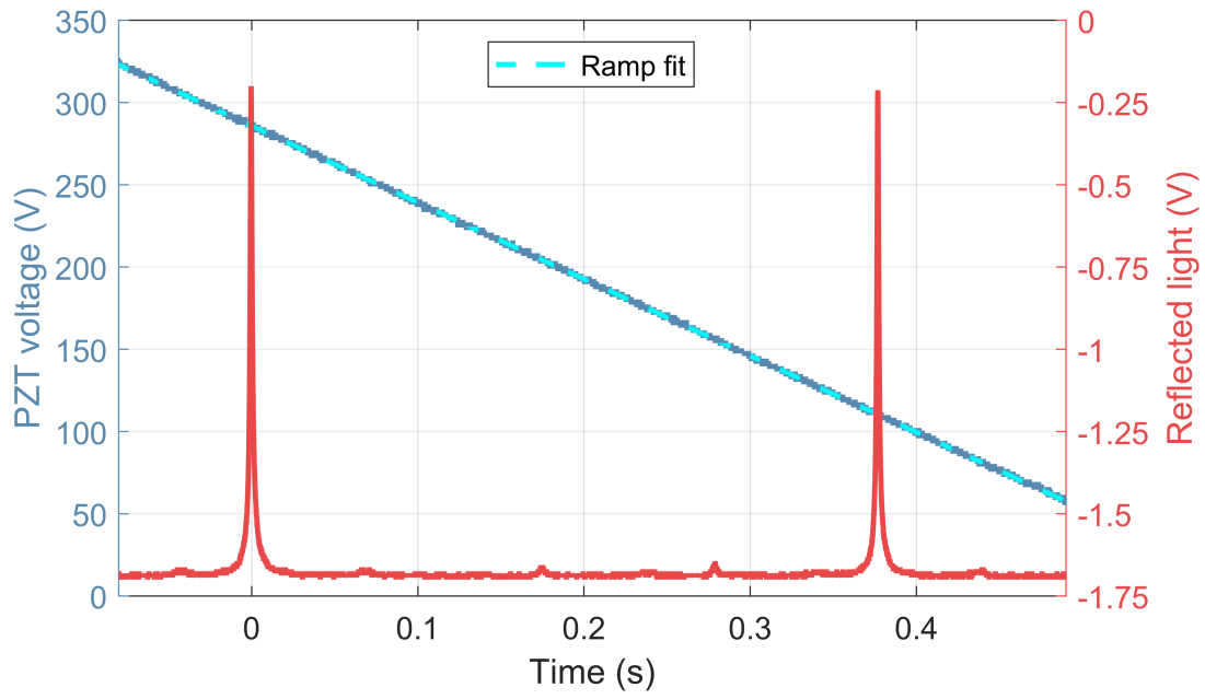
Figure 2.25: A ramp was applied to the PZT and the reflected light from the cavity was measured. The FSR of the cavity is known, so the time in this measurement can be converted to frequency giving the PZT transfer function at low frequencies. The ramp signal is shown in blue and the reflected light is shown in red.
