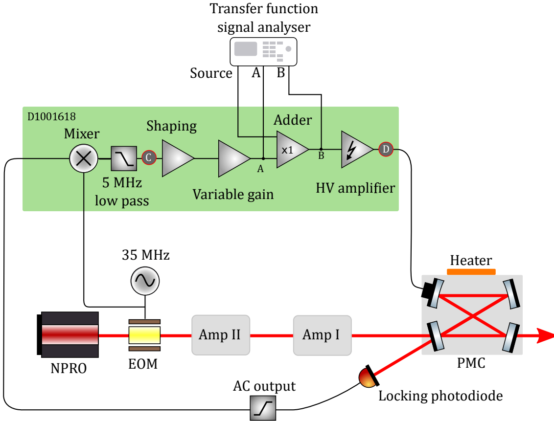
Figure 2.22: A sketch of the frequency stabilisation servo. An EOM produces 35 MHz sidebands which are used to produce a PDH locking signal. A PZT controls the length of the cavity at high frequencies. A heater and a digital loop is used to provide slow control so that the PZT can operate around its mid point. The open loop transfer function was measured using signals at A and B, and the frequency noise was measured using the error point and control signals marked by C and D.
