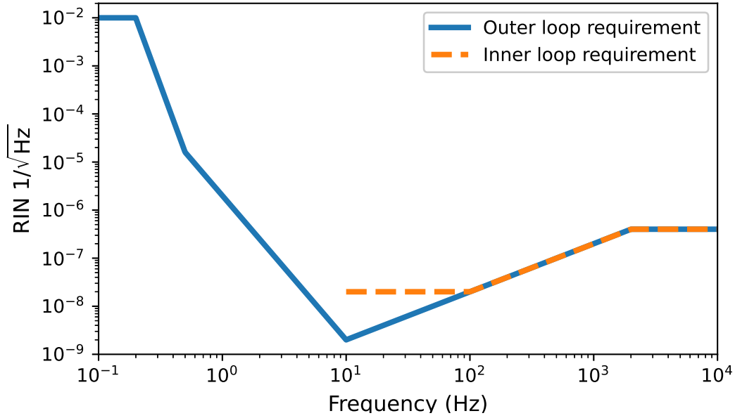
Figure 2.12: A reproduction of the intensity noise requirement from [12]. The outer loop requirement is shown in blue and the inner loop is shown by the orange dashed line. At frequencies below 10 Hz, the outer loop requirement is determined by the radiation pressure noise that is expected to arise due to imbalances in the arm power. The requirement is most stringent at 10 Hz. Due to the PRC cavity pole, the requirement relaxes above 10 Hz. The inner loop requirement is less extreme than the outer loop as it is only needed to stabilise the laser in the initial locking sequence and not for during an observation run.
