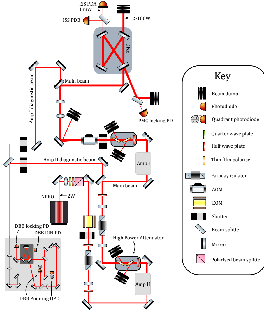
Figure 2.2: Sketch of the prototype optical layout that was constructed in the TnT lab. The main beam path and diagnostic beam paths are shown. Key photodiodes are also shown. A to-scale version of this layout is found in [20]. This layout does not include the frequency stabilisation optics that will feature in the PSL.
