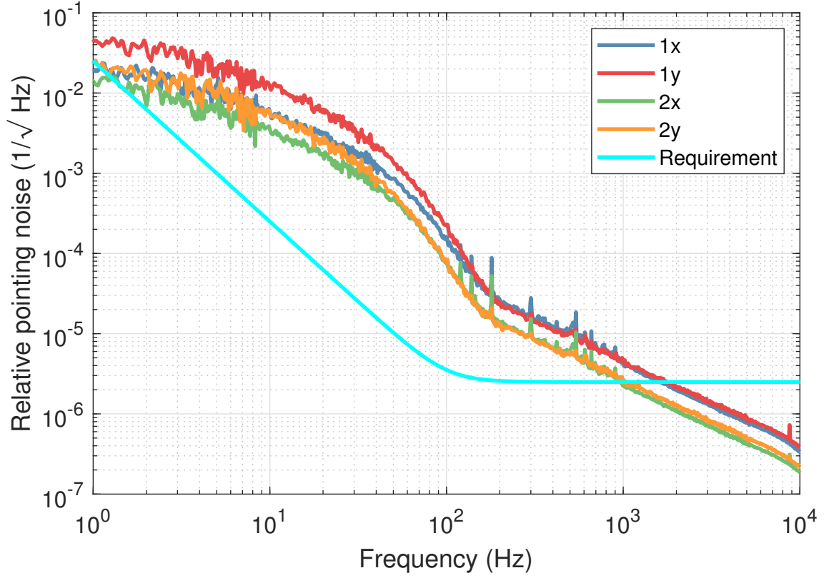
Figure 2.21: The four relative pointing noise degrees of freedom for the the beam into the PMC was measured with the DBB. The requirement [28] is shown in light blue. The pointing noise is above the requirement, however the TnT lab has a higher amount of environmental noise, this pointing noise will be less in the PSL. Measurements below 100 Hz may be affected by scattering.
