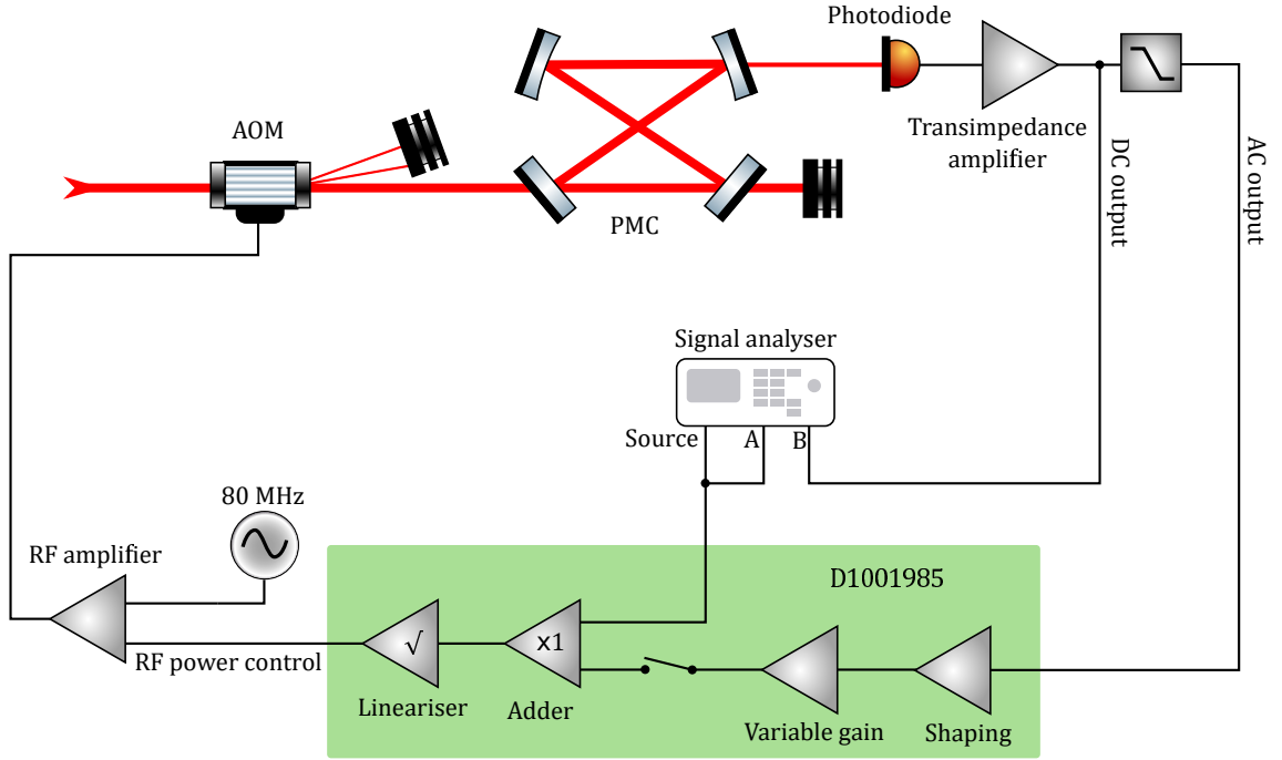
Figure 2.14: A sketch of how the AOM transfer function was measured. The components of the intensity stabilisation servo has also been shown. The PMC was locked and a signal analyser was used to perform a swept sine measurement. A chip that performs a square root operation to an input signal was used to linearise the AOM. The transfer function was measured between the input to this chip and the photodiode used for the intensity stabilisation. The servo electronics are detailed in D1001985 and D1001998.
