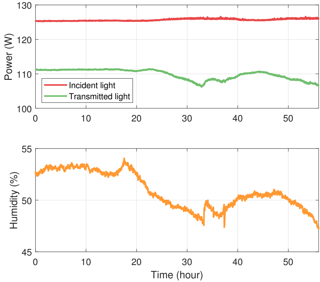
Figure 2.7: The top panel shows the power that was incident to the PMC and the power transmitted by the PMC over a 55 hour run. The light produced by the amplifiers did not change significantly for the duration of this measurement, however the transmitted light through the PMC dropped from 111 W to, at its lowest, 107 W. This is likely due to the environmental conditions in the lab changing. The bottom panel shows the humidity of the lab, and changes in the humidity, which can be caused by a temperature change, coincides with changes in the power level of the amplifier.
