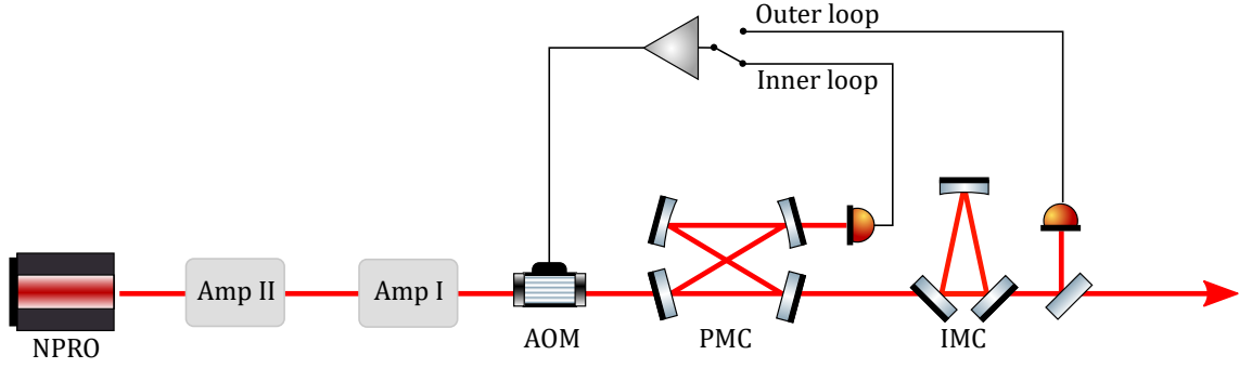
Figure 2.11: The intensity stabilisation concept involves two loops. The inner loop is responsible for stabilising the laser so that the IMC can lock. The outer loop is used to stabilise the laser for observation mode. The two loops sense the laser intensity noise at different points. The inner loop uses a low power beam transmitted by the PMC. The outer loop uses a pick-off from the main beam. An AOM is used to actuate on the laser's power.
