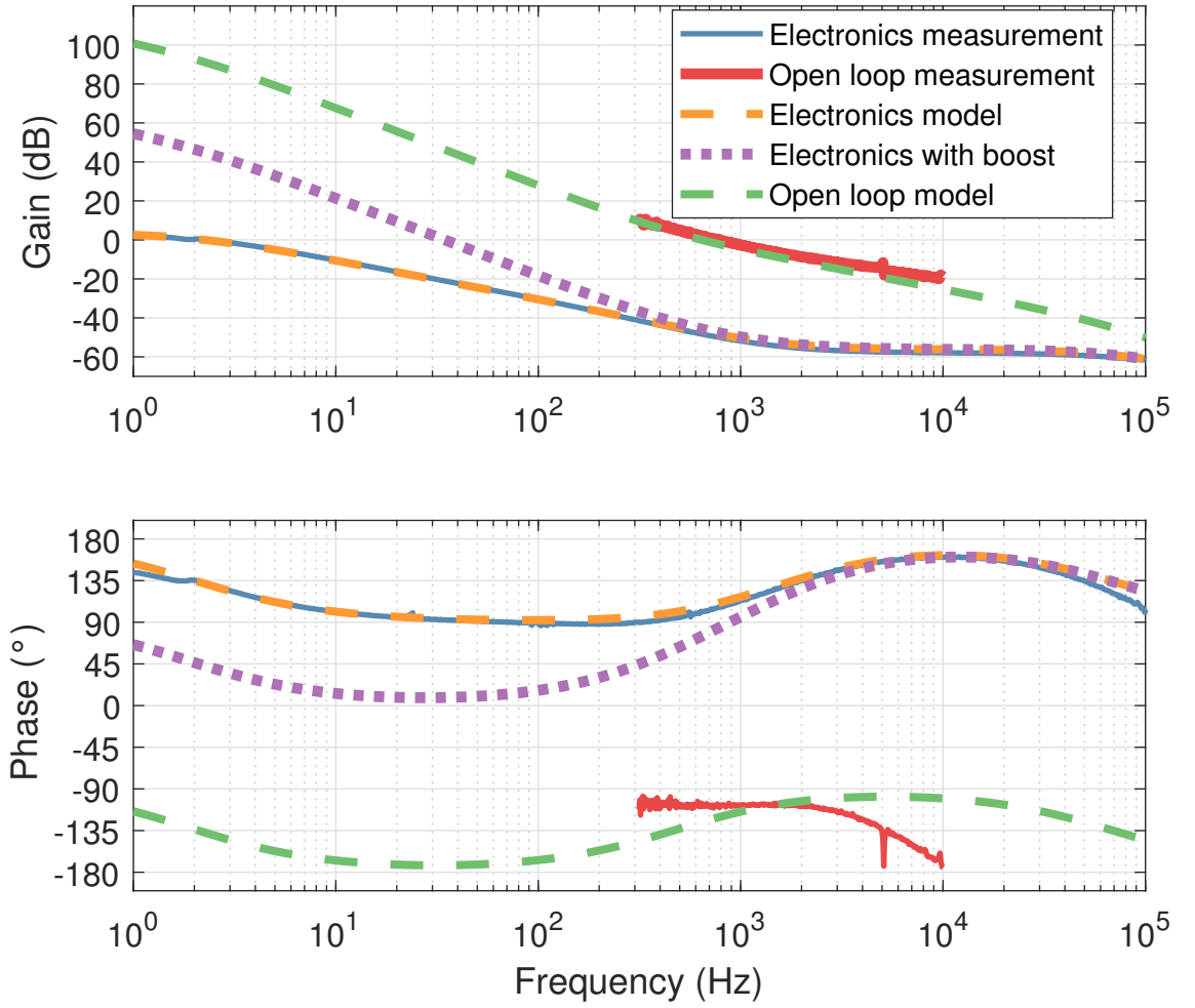
Figure 2.26: The open loop transfer function was measured using the layout shown in figure 2.22. This is shown in red. The electronics transfer function, without the ‘boost’ provided by an extra integrator stage, was measured and is shown in blue. The model of this is shown in orange. The boosted electronics model is shown in purple. The green line shows the expected servo gain based on the boosted electronics model and the measurements shown in Figures 2.24 and 2.25. This model is within 2 dB of the measurement. The unity gain point was measured to be at \sim 800 Hz.
