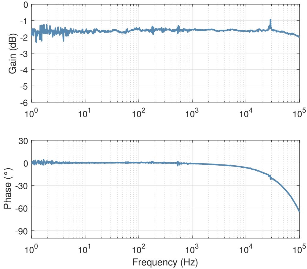
Figure 2.15: Using the layout shown in figure 2.14, the transfer function of the input to the linearisation stage before the AOM to light power change on the ISS photodiode was measured. The response was normalised by dividing by the DC power on the photodiode. The transfer function is flat over the region where there open loop gain needs to be greater than one ( \sim 10 kHz), There is a small amount of phase lag at higher frequencies.
