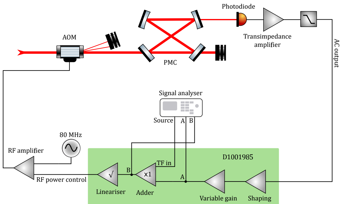
Figure 2.18: The open loop transfer function of the servo was measured by injecting a signal at a times one adding stage. The points immediately before and after this stage were measured, and the ratio of these two stages gives the open loop transfer function of the servo.
