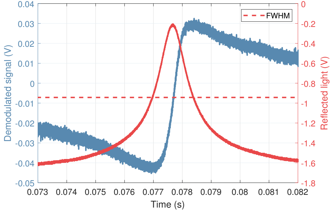
Figure 2.24: A ramp was applied to the PZT and photodiode signal was measured before and after demodulation. The demodulated photodiode signal is shown in blue. The photodiode signal is shown in red. Around the peak of the photodiode signal the slope of the demodulated signal gives the gain of the ‘optics’ transfer function. This can be expressed in units of MHz/V by converting the time axis to a frequency axis. This is done by using the full-width-half-maximum of the photodiode signal as a reference frequency.
