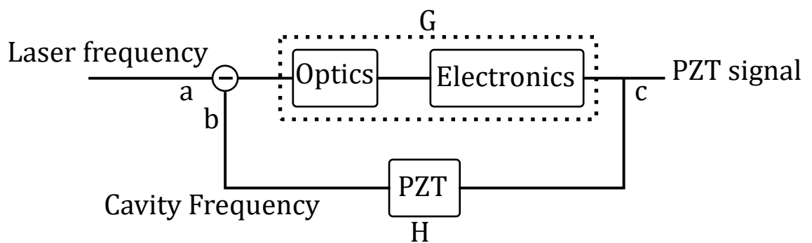
Figure 2.23: The servo can be considered as being made of three parts: the optics, the shaping electronics and the PZT. The optics block waht is obtained after the photodiode signal is demodulated. When at resonance, this is a flat transfer function that is proportional to the difference in frequency, although at MHz frequencies the cavity pole will affect this. The electronics transfer function includes everything after the mixer up to and including the final high power OP amp. The PZT tranfer function converts a voltage to a cavity frequency. The PZT acts as a low pass filter due to it having capacitance.
