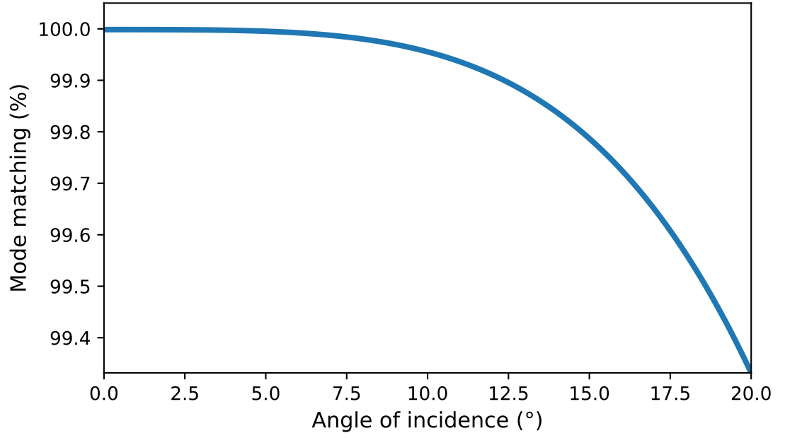
Figure 2.4: Astigmatism is a source of loss. When designing this layout, to explore how sensitive it was to astigmatism, the AOI for the curved mirrors was altered. Using equation (2.1), the loss was computed. This effect is negligible up to 10^\circ after which it starts to become significant compared to the losses summarised in Table 2.1.
