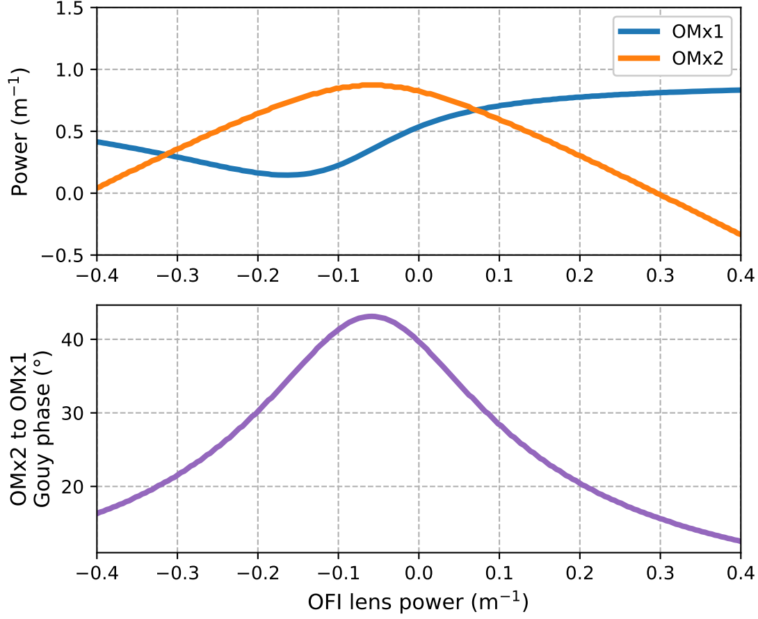
Figure 2.3: Top panel: The choice of OFI lens power affects the combination of OMx1 and OMx2 power required for 100% mode matching. Bottom panel: The best choice of OFI lens corresponds to where the Gouy phase separation between the pair of OMx1 and OMx2 mirrors that give 100% mode matching is closest to 45^\circ . The optimal Gouy phase separation between OMx1 and OMx2 achievable by this layout is 43^\circ .
