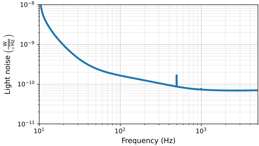
Figure 1.4: The intensity noise of the light at the AS port for the A+ detector. This was obtained by deconvolving the detectors sensitivity curve with the function shown in Figure 1.3. At frequencies above 1 kHz the noise is flat as it is dominated by shot noise. At lower frequencies the noise is increased relative to shot noise due to radiation pressure, coating thermal noise and other noise sources. The spike in the spectrum at 500Hz represents the presence of suspension modes (actually find out what this is).
