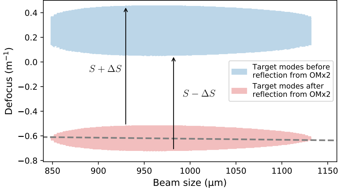
Figure 2.6: This is the WS space at the OMx2 plane. The affect of OMx2 in the plane of OMx2 is to move a mode vertically in WS space. After reflection from OMx2, a mode must be at least 98% mode matched to the OMC as there are no further active mode matching elements in the layout of HAM6. Modes with at least 98% are shown by the red region. The blue region represents which modes can be reached from the red region by either S_{\text{OMx2}} \pm \Delta S , and was constructed by applying transformations to the modes in the red region. The red region was split into two parts, ‘upper’ and ‘lower’, indicated by the dashed line that connects the two extremes in width of the region. To create the lower edge of the blue region, modes in the lower edge of the red region had the transformation corresponding to a mirror power of S_{\text{OMx2}} - \Delta S applied to them. To construct the upper edge of the blue region, upper edge of the red region had the transformation corresponding to a mirror power of S_{\text{OMx2}} + \Delta S applied to them.
