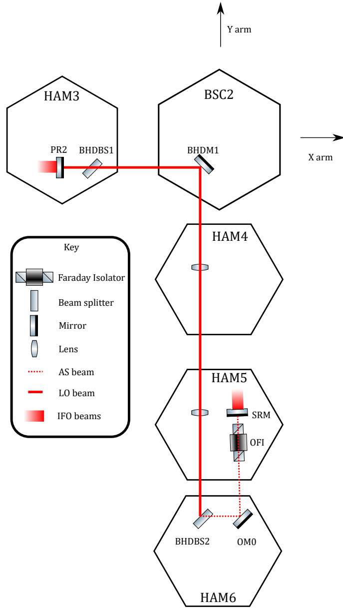
Figure 1.2: Sketch of the LO and signal beam paths. The HAM tables are shown by the hexagons. Most of the interferometer has not been shown for clarity. The main interferometer beam is indicated by a thick, gradated red line. The thinner red line indicates the LO beam, and the signal beam is shown with a dashed red line.
