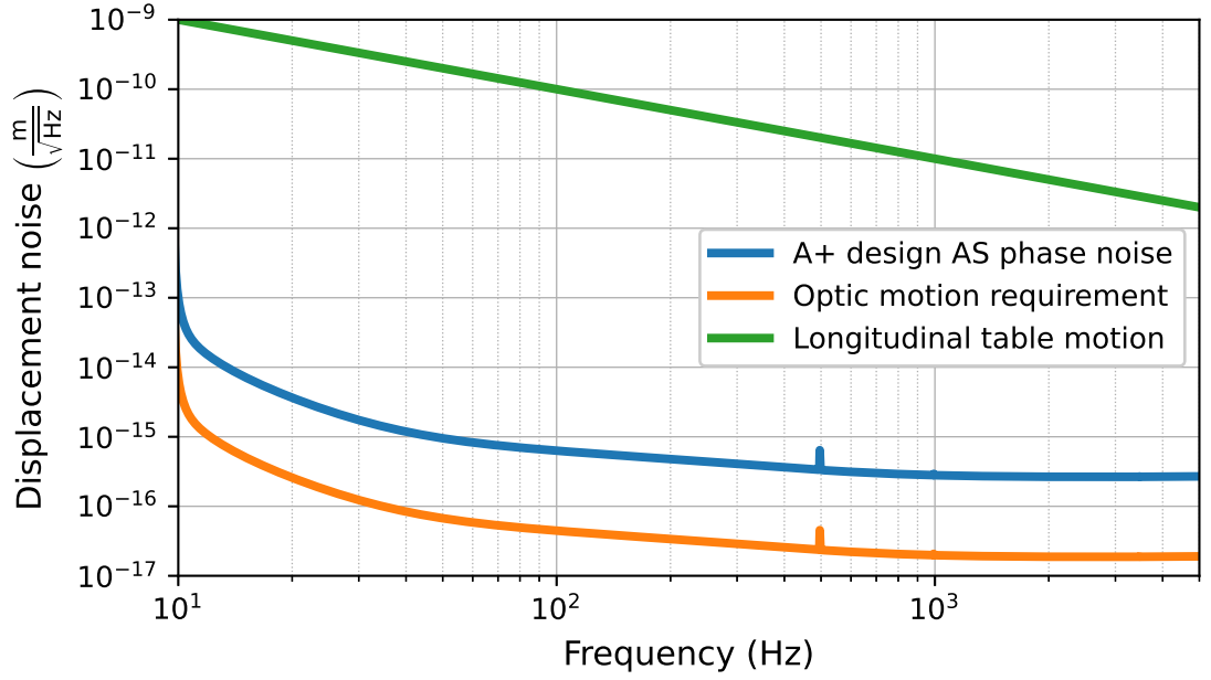
Figure 1.6: The phase noise between the LO and the signal beams causes noise. The sensitivity curve for A+ sets the limit on how much path length noise is acceptable between the AS and LO beams. The blue line shows sensitivity curve is shown in units of path length noise between the AS and LO beams, and the orange line shows the requirement of HRTS mirror motion. The table motion was modelled as 1/f noise.
