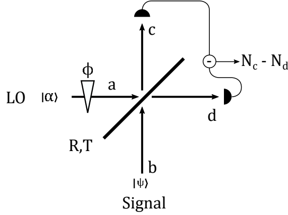
Figure 1.1: A coherent state |\alpha\rangle , enters port a of a beam splitter. A signal |\Psi\rangle enters port b . These two beams interfere, resulting in photons being detected at the c and d ports. The two photo-currents are subtracted, and the signal that is produced is proportional to an arbitrary quadrature of the state |\Psi\rangle . The quadrature that is measured is determined by the homodyne angle, \phi . This is expressed mathematically by equation (??).
