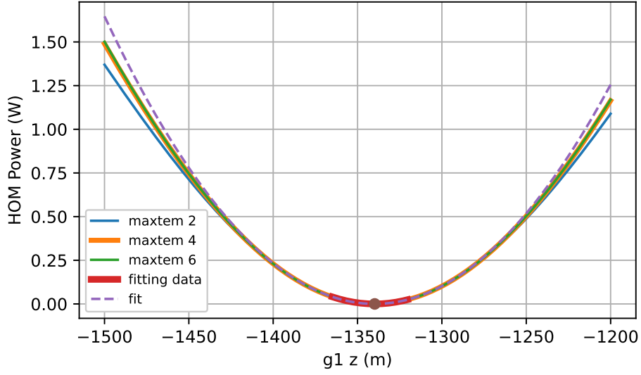
Figure D.1: Optimisation of parameters used in the gauss command to mode match the laser to the arms in the simulations described in chapter 4 and section D.3. The blue, green and orange lines show how the mode matching changes as the beam waist location is changed. As the mode matching becomes larger, more HOM are required, as the blue and green/orange lines diverge. A quadratic was fitted to the data highlighted in red, and the minimum value was used as the waist location parameter for the gauss command.
