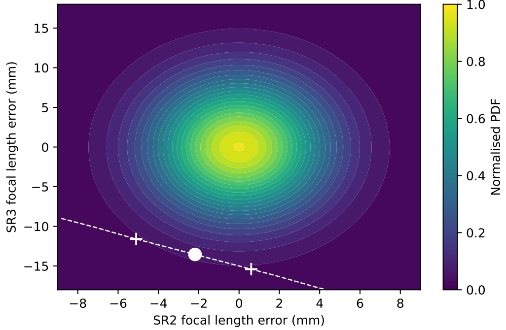
Figure 4.11: The measurement error of SR3 and SR2 follows a normal distribution. These were combined to make a 2-D normal distribution. Dark blue corresponds to the least likely combinations of SR3 and SR2, and bright yellow corresponds to the most likely. The measured Gouy phase was 21.3^\circ [146]; this is indicated by the white dashed line. The white circle marks the most likely combination of SR3 and SR2 which gives 21.3^\circ of Gouy phase, and the white crosses show one standard deviation from this. The white circle and crosses indicate that the focal length of SR2 is -3.205 \pm 0.003 m and the focal length of SR3 is 17.971 \pm 0.002 m.
