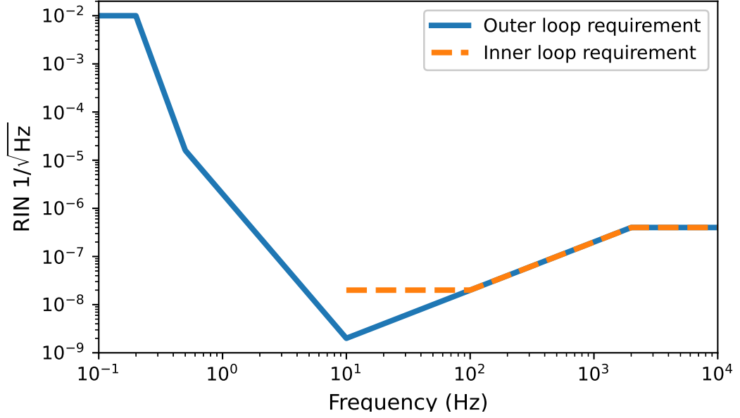
Figure 3.12: A reproduction of the intensity noise requirement from [12]. The outer loop requirement is shown in blue and the inner loop is shown by the orange dashed line. At frequencies below 10 Hz, the outer loop requirement is determined by the radiation pressure noise that is expected to arise due to imbalances in the arm power. The requirement is most stringent at 10 Hz. Due to the PRC cavity pole, the requirement relaxes above 10 Hz. The inner loop requirement is less extreme than the outer loop as it is only used to stabilise the laser in the initial locking sequence and not during an observation run.
