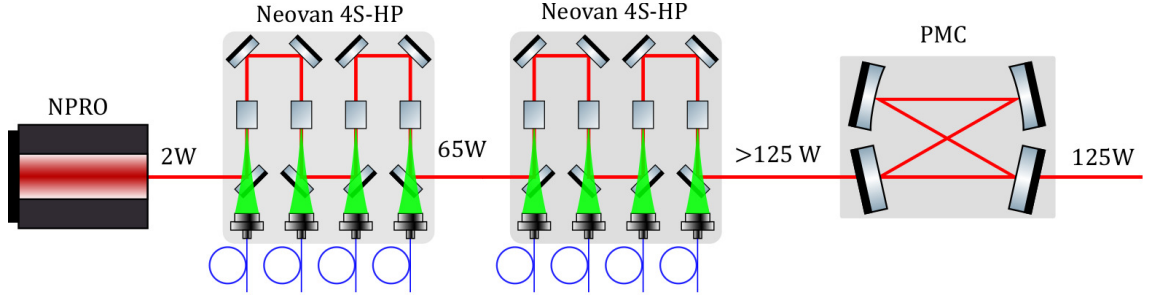
Figure 3.1: Conceptually, the PSL will be made up of four components: the NRPO, two Neovan 4S-HP amplifiers and the PMC cavity. The NPR0 provides seed light with good noise characteristics. These noise characteristics are preserved by the amplifiers, so the resulting beam will have high power and low noise. The PMC filters junk light and RF intensity noise so a spatially pure mode can be set to the interferometer.
