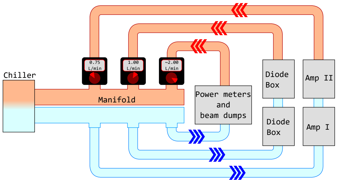
Figure 2.2: Cartoon of the cooling layout for the PSL. The amplifiers are on a separate loop to the diode boxes so that the flow rates for these can be reduced as much as possible.
