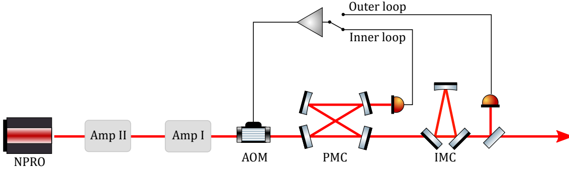
Figure 2.5: ISS concept
