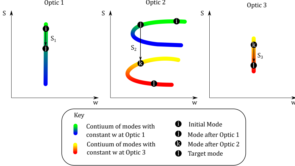
Figure E.2: Sketch of the WS phase space representations of the Gaussian beams at the three positions along the optical axis where a mirror or a lens could be. Examples of such layouts are shown in Figure E.1. The optical power of the first optic is given by the difference in the defocus between the initial mode (i) and the second mode (j). The power of the second optic is found by finding the difference in defocus from the blue-green continuum to the red-yellow continuum. There are 2 optical powers that will move the mode j to the red-yellow continuum, and two possible modes in the blue-green continuum from which k can be reached, giving 4 possible similar solutions. The algorithm can be set up so that it is only one way of moving between the blue-green and red-yellow continua by limiting their extent. The power of the third optic is found from the difference between the mode k and mode l at optic 3.
