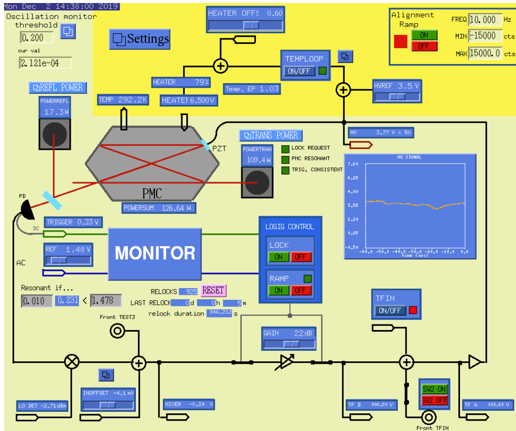
Figure C.1: The MEDM screen for locking the PMC.
