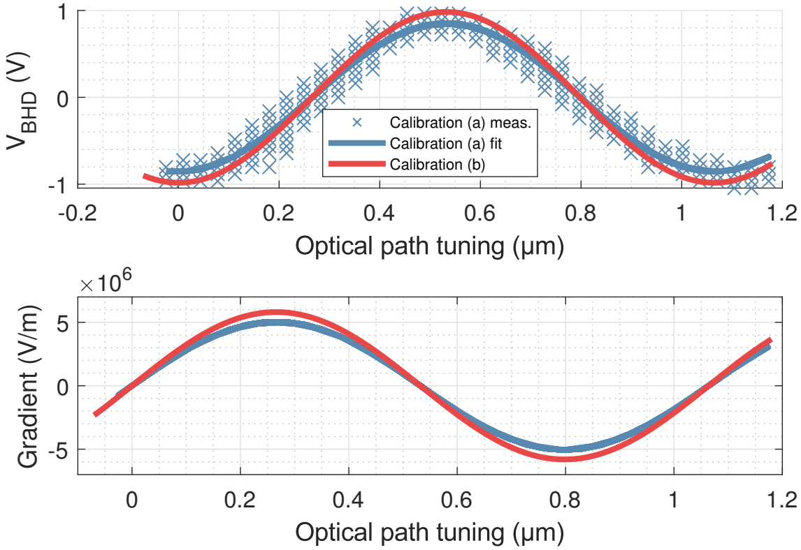
Figure 8.6: There are two ways of calibrating the differential photodiode signal that will be generated by a change in optical path length between the two paths in the Mach-Zehnder. Method (a) is to measure a ramp signal that is applied to the PZT while simultaneously measuring the photodiode signals. The measurement of this is shown by the blue crosses, and the fit to this data is shown by the blue line. Method (b) is to measure the power in the local oscillator and signal beams when they are not interfering. From this, Equation (5.14) can be used to find the response of the Mach-Zehnder. This is shown by the red line. Thus, the blue and red data are independent of each other. The two calibrations agree to within 10%. The gradient of V_{BHD} is used to get the conversion factor for a change in beam power to a change in differential path length.
