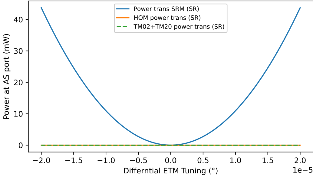
Figure 4.4: The minimum of the dark fringe is at 0° differential ETM detuning, as shown by the blue line. A slight offset causes light to be at the AS port. This result was used to determine tunings for simulating what effect focal length errors in SR3 and SR2 have on the beam transmitted through the SRM. The orange line and dashed green line show the HOM content of the beam.
