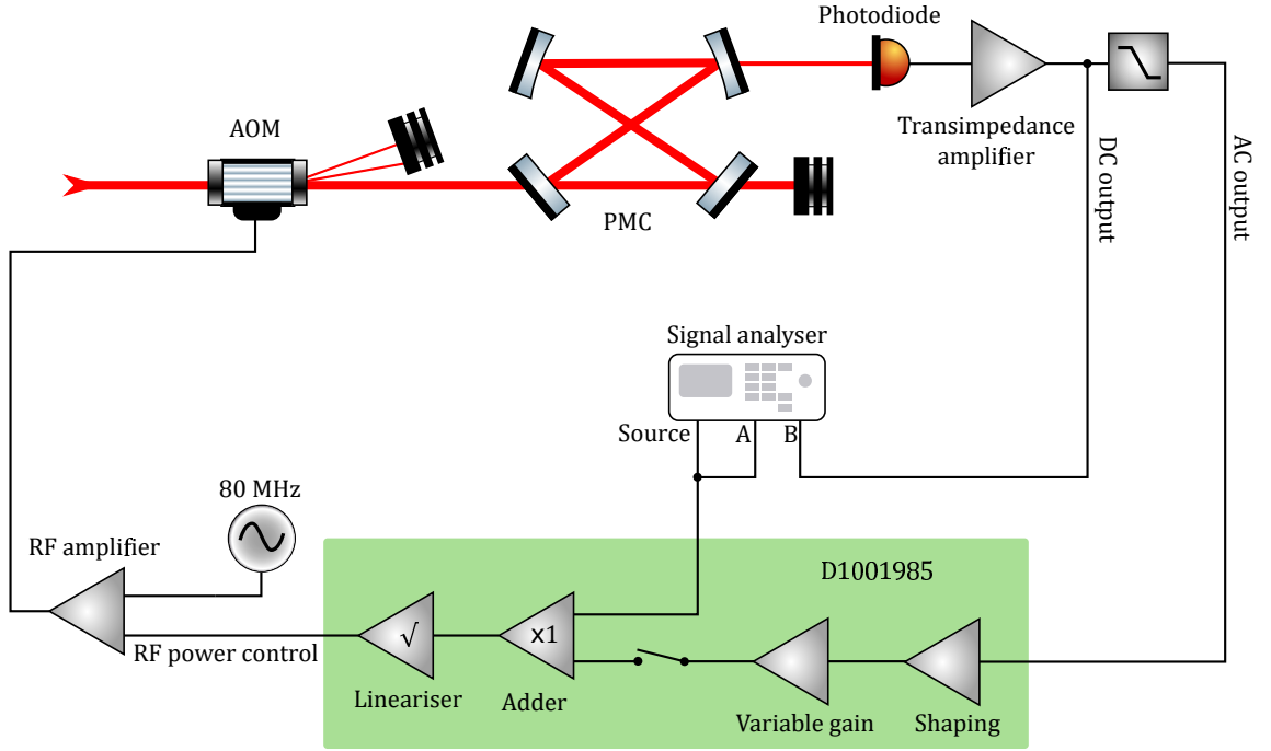
Figure 3.14: A sketch of how the AOM transfer function was measured. The components of the intensity stabilisation servo has also been shown. The PMC was locked and a signal analyser was used to perform a swept sine measurement. An IC (AD734) that performs a square root operation to an input signal was used to linearise the AOM's effect on beam power to an input signal. The transfer function was measured between the input to the lineariser and the photodiode used for the intensity stabilisation. The servo electronics are found in [115] and [116].
