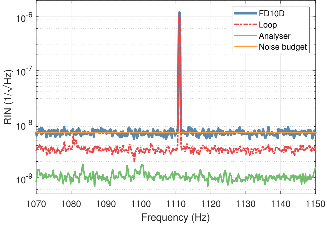
Figure 7.3: The bias of the FD10D was set to 0.6 V, and it was exposed to 15 mW of 1.55 \mu m light. 15 mA of photocurrent was generated. The noise of the photocurrent produced by the FD10D (blue line) corresponds to the level predicted by Equation 7.3 (orange line) meaning that the increase in photocurrent can only be explained by an increase in quantum efficiency. The 1111 Hz signal was used to calibrate the measurement as this modulation also could be measured on the high-performance in-loop photodiode.
