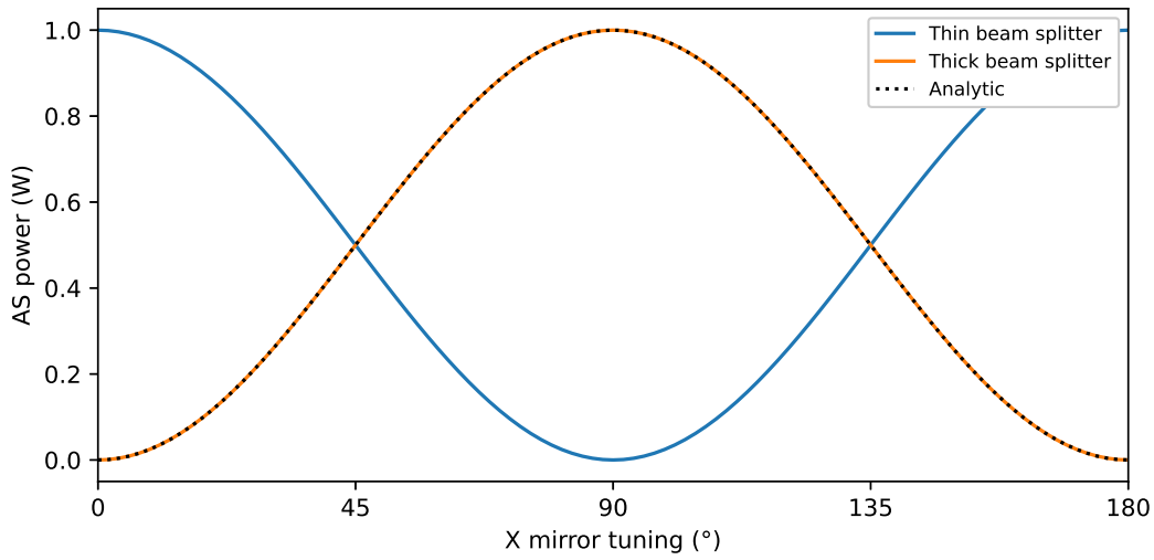
Figure 4.2: The simulation of a Michelson interferometer with thin a beam splitter is shown in blue. The same simulation was done with a thick beam splitter, this is shown in orange. The analytic behaviour of a Michelson interferometer (Equation (4.1)) is shown by the dashed black line. The tuning of one of the arm mirrors was changed and the power at the AS port was simulated. Comparing the outputs of the simulation to Equation (4.1) shows that thick beam splitters should be used.
