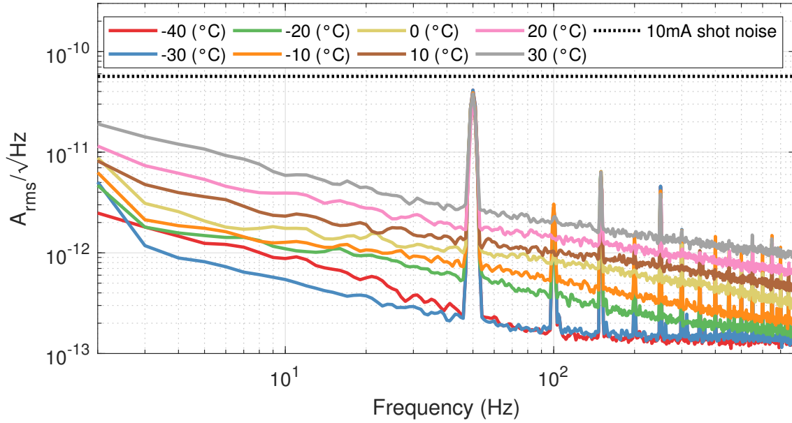
Figure A.12: G12182-005k at 1.0V reverse bias.
