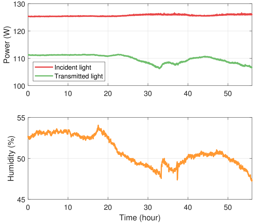
Figure 3.7: The top panel shows the power that was incident on the PMC and the power emerging from the PMC over a 55 hour trail run. The light produced by the amplifiers did not change significantly for the duration of this measurement, however the transmitted light through the PMC dropped from 111 W to, at its lowest, 107 W. This is likely due to the environmental conditions in the lab changing. The bottom panel shows the humidity of the lab. Changes in the humidity, which can be caused by a temperature change, coincide with changes in the power emerging from the PMC.
