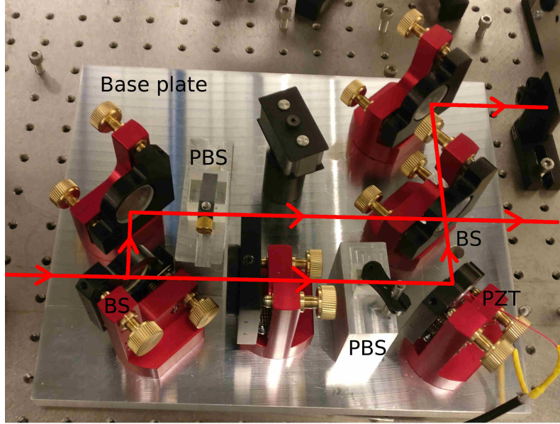
Figure 8.2: Photograph of the Mach-Zehnder base plate. The polarising beam splitters were part of an earlier design; they were removed when the measurements with this apparatus were made.
