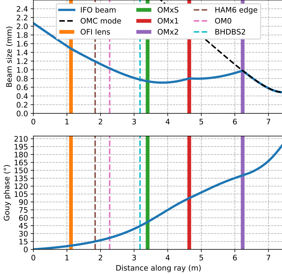
Figure 1.7: Top panel: the radius of the beam as it travels from the SRM ( z = 0 ) to the waist of the OMC. Significant points along the axis are marked with vertical lines. Bottom panel: The gouy phase shift accumulated by the beam as it propagates along the optical axis.
