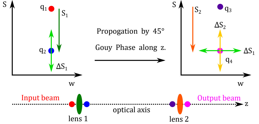
Figure 1.10: Sketches of the WS representation for a Gaussian beam interacting with different parts of a simple optical layout consisting of two active lenses with powers S_{1,2} + \Delta S_{1,2} . The left hand axis shows the WS plane at lens 1. The input beam q_1 is indicated by a red dot, and the effect of the lens on q_1 is shown by the dark green arrow S_1 . This results in a new mode q_2 , which is shown as a blue dot. A light green arrow indicates the actuation of lens 1. The right hand axis shows the WS plane at lens 2. The input mode at lens 2, q_3 , is shown as a purple dot, and the output mode q_4 is shown as a pink dot. The static and dynamic power of lens 2 is indicated by the orange and yellow lines. As lens 1 and lens 2 are separated by 45^\circ of Gouy Phase, the actuation provided by lens 1 results in a change in the beam parameter which is orthogonal to the actuation provided by lens 2, provided that the actuations are small enough.
