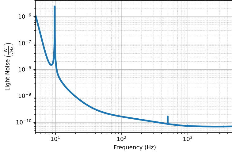
Figure 1.3: The intensity noise of the light at the AS port for the A+ detector. This was obtained by deconvolving the detectors sensitivity curve[10] with the function shown in figure 1.2.
