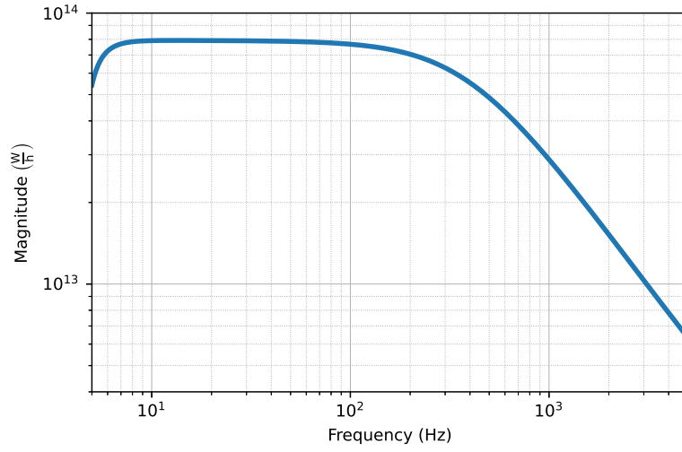
Figure 1.2: The linear response function between strain and light power at the AS port was obtained from a FINESSE simulation of the LLO detector[9]. The corner frequency at \approx 300 Hz comes from the pole of the coupled SRC-arm cavity. The behaviour below 6 Hz is due to optical spring effects.
