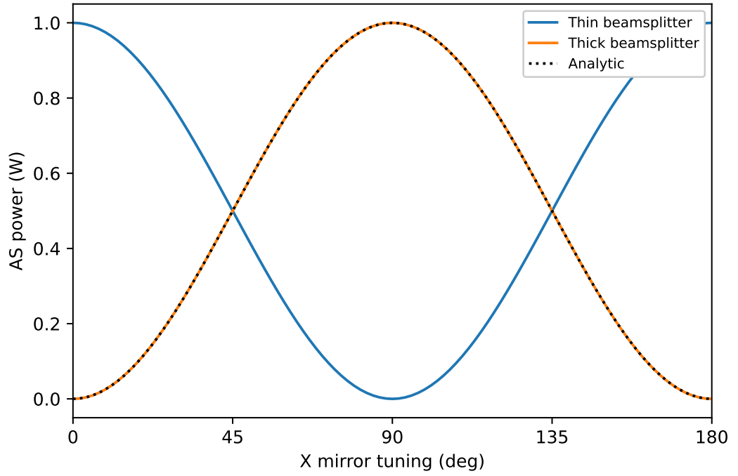
Figure 7.1: The simulation of a Michelson interferometer with thin a beamsplitter is shown in blue. The same simulation was done with a thick beam splitter, this is shown in orange. The analytic behaviour of a Michelson interferometer (equation 7.1) is shown by dashed black line. The tuning of one of the arm mirrors was changed and the power at the AS port was measured. Comparing the outputs of the simulation to equation 7.1 shows that thick beamsplitters should be used.
