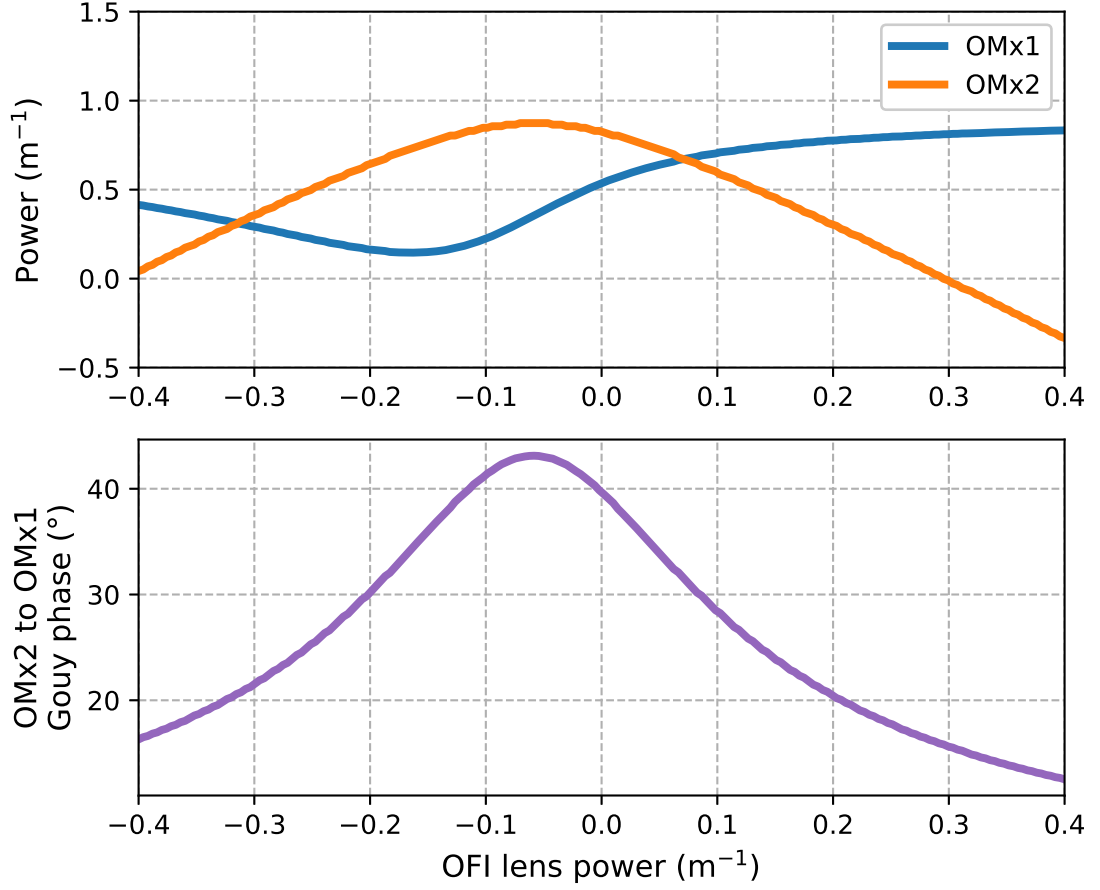
Figure 9.3: Top panel: The choice of OFI lens power affects the combination of OMx1 and OMx2 power that is required for 100% mode-matching. Bottom panel: The best choice of OFI lens corresponds to where the Gouy phase separation between the pair of OMx1 and OMx2 is closest to 45^\circ . The most Gouy phase separation between OMx1 and OMx2 achievable by this layout is 43^\circ .
