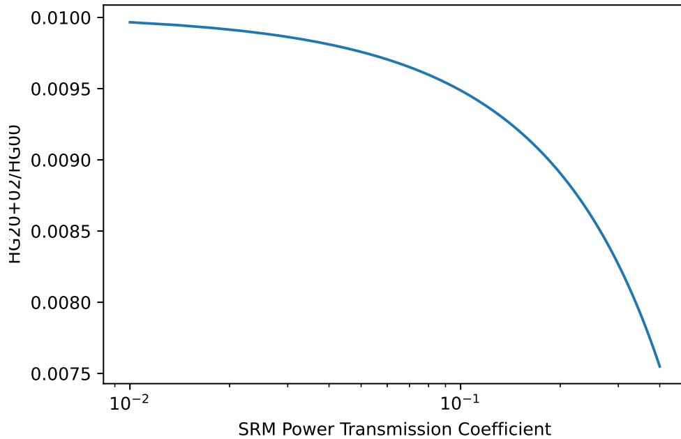
Figure 7.14: Ratio of HG20+02 to HG00 as the transmission of the SRM is increased for a mode mismatch between the arm cavity and the SRC. The interferometer is in RSE mode. A mode mismatch was introduced by setting the focal length of SR3 to be 12 mm shorter than the nominal amount.
