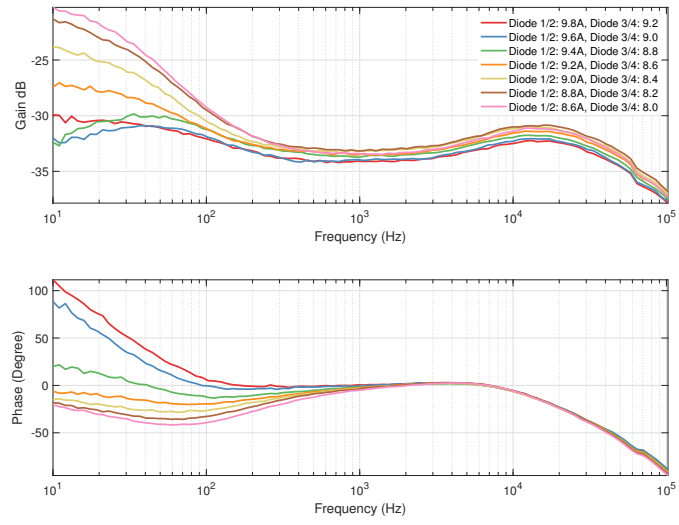
Figure 6.3: current shunt input to light power transfer function for different diode currents
