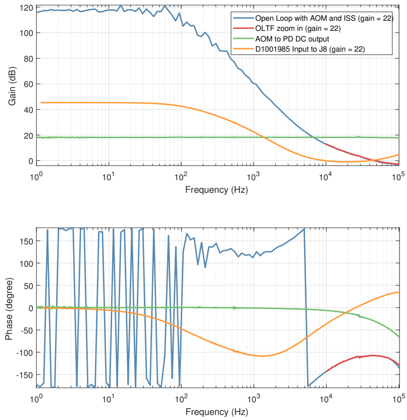
Figure 6.2: Transfer functions for parts of the AOM servo
