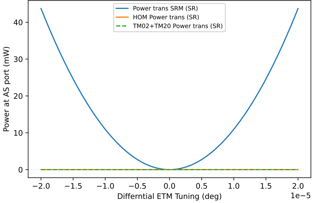
Figure 7.3: The minimum of the dark fringe is at 0^\circ differential ETM detuning, as shown by the blue line. A slight offset causes light to be as the AS port. This result was used to determine tunings for simulating what effect focal length errors in SR3 and SR2 have on the beam transmitted through the SRM. The orange and green dashed line show the HOM content of the beam.
