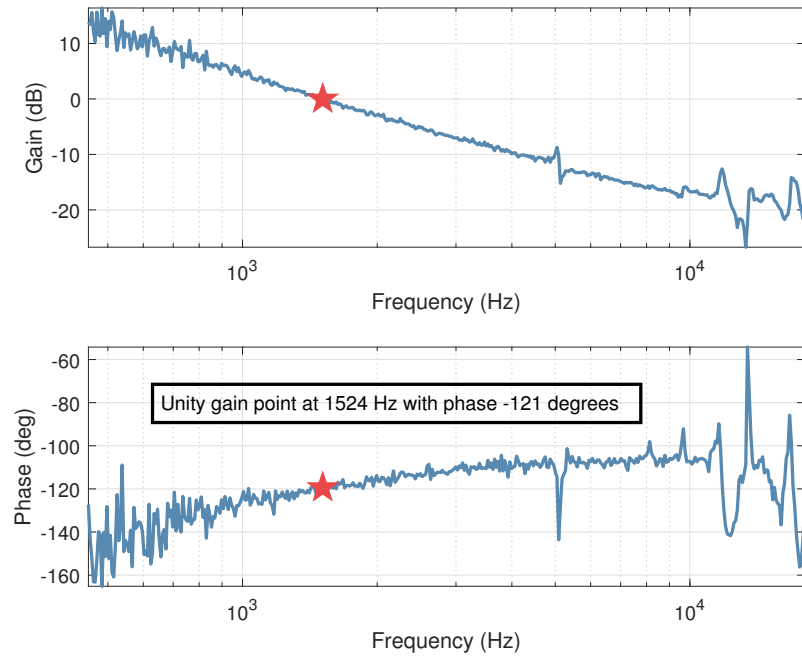
Figure 5.2: Open loop gain of frequency stabilisation loop
