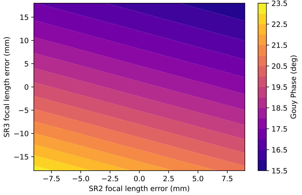
Figure 7.7: Gouy phase between the ITMs and the SRM as a function of the error ( \pm 3\sigma ) in SR3 and SR2. When the SR3 focal length error > 6 mm and SR2 error is zero the SRC cavity is unstable (see figure 7.9), so this area of the parameter space is unlikely to correspond to the beam at the SRM at LLO.
