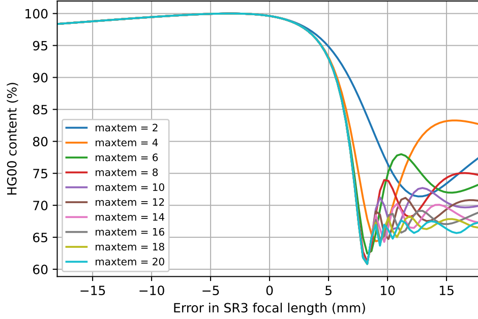
Figure 7.9: The percentage of HG00 light transmitted through the SRM as a function of SR3 focal length for the Michelson interferometer with Fabry-Perot cavities in its arms was simulated. Each simulation used a different maxtem command. The focal length of SR3 was changed. For focal lengths with a positive error greater than 7.5 mm, the cavity becomes unstable and FINESSE does not produce reliable results. For a stable SRC, the minimum number of TEM modes for sub 1% accuracy is six.
