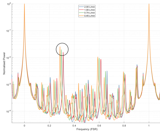
Figure 5.3: Flow rates affecting the thermal lensing, resulting in increased ellipticity
