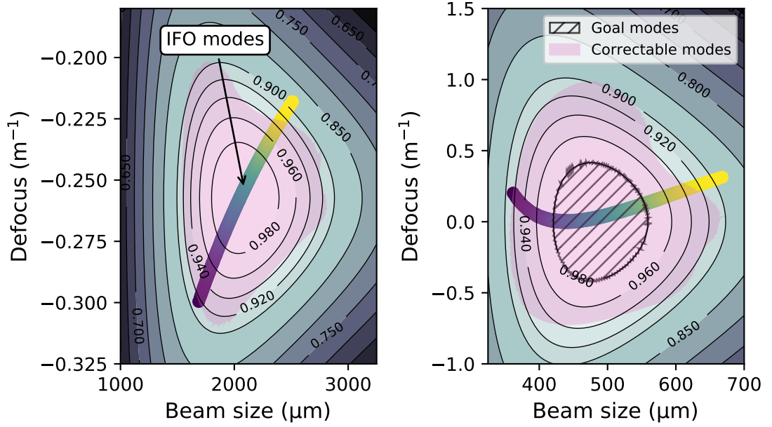
Figure 9.7: Left panel: the set of modes that could be present at the SRM, as described in Chapter 7, is shown by the purple-blue-green-yellow curve. The pink region shows which modes can reach 98% mode-matching by using the AWC in HAM6. The contours indicate the mode-matching between a mode (W, S) and the OMC mode. Right panel: this shows the same modes as the left panel, except they have been transformed by the optical layout to the plane of the OMC waist. Modes within the pink region can be actuated on so they move to the goal region, which is indicated with a hatched area.
