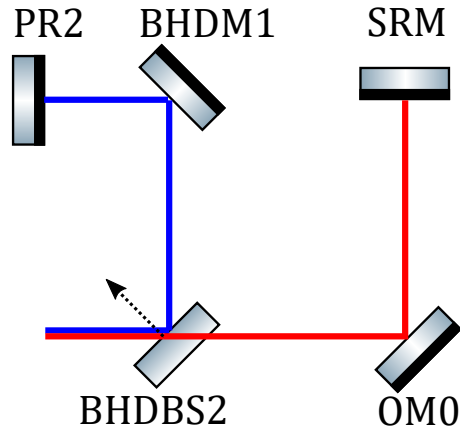
Figure 8.5: A sketch of the LO and signal beam paths. The LO beam path is shown in blue, and the signal beam is shown in red. A dashed arrow indicates the direction that the recombining beam splitter, BHDBS2, may move in. If BHDBS2 moves in this way, the phase of the signal beam has increased while the phase of the LO beam has decreased at the point where the signal and LO beams combine. This means that the recombination beam splitter motion needs to be counted twice in calculations of the phase noise requirement.
