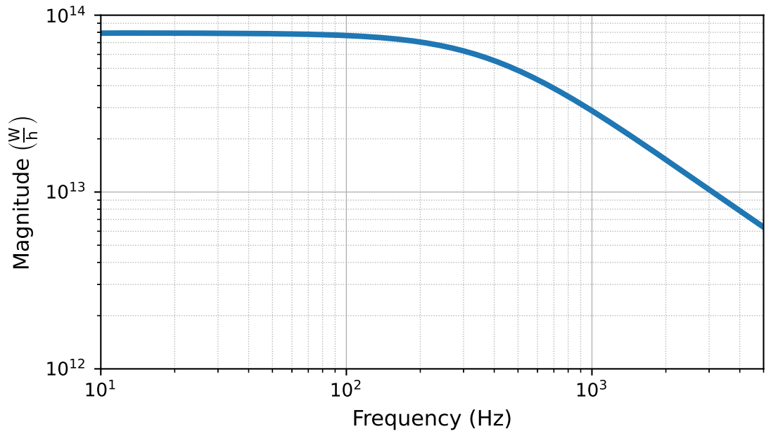
Figure 8.3: The linear response function between strain and light power, expressed in units of Light Power/gravitational wave strain, at the AS port was obtained from a FINESSE simulation of the LLO detector. The corner frequency at \approx 300 Hz comes from the pole of the coupled SRC-arm cavity.
