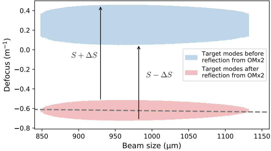
Figure 9.6: This is the WS space at the OMx2 plane. The effect of OMx2 in the plane of OMx2 is to move a mode vertically in WS space. After reflection from OMx2, a mode must be at least 98% mode-matched to the OMC as there are no further active mode-matching elements in the layout of HAM6. Modes with at least 98% are shown by the red region. The blue region represents which modes can be reached from the red region by either S_{\text{OMx2}} \pm \Delta S , and was constructed by applying transformations to the modes in the red region. The red region was split into two parts, ‘upper’ and ‘lower’, indicated by the dashed line that connects the two extremes in width of the region. To create the lower edge of the blue region, modes in the lower edge of the red region had the transformation corresponding to a mirror power of S_{\text{OMx2}} - \Delta S applied to them. To construct the upper edge of the blue region, the upper edge of the red region had the transformation corresponding to a mirror power of S_{\text{OMx2}} + \Delta S applied to them.
