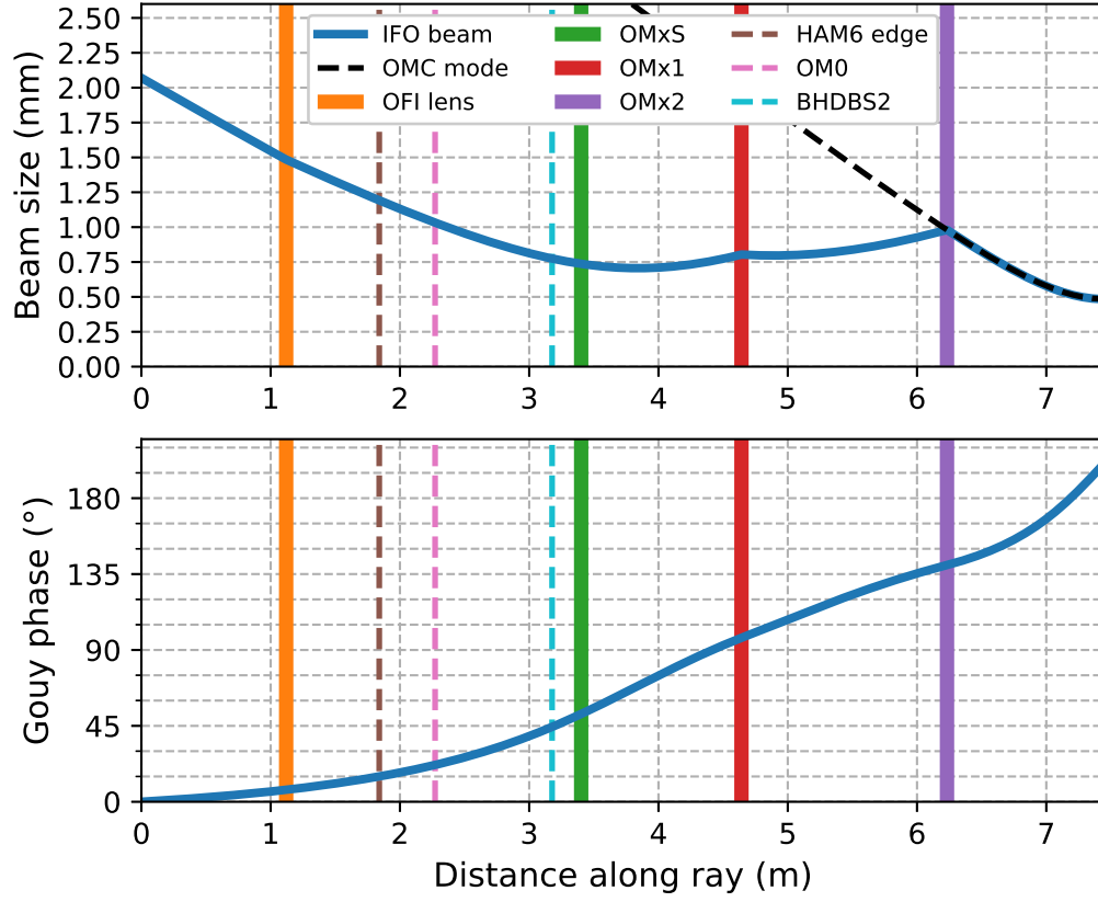
Figure 9.2: Top panel: the radius of the beam as it travels from the SRM ( z = 0 ) to the waist of the OMC. Significant points along the axis are marked with vertical lines. Less significant, but useful, reference points are marked by dashed vertical lines. Bottom panel: The Gouy phase shift accumulated by the beam as it propagates along the optical axis.
