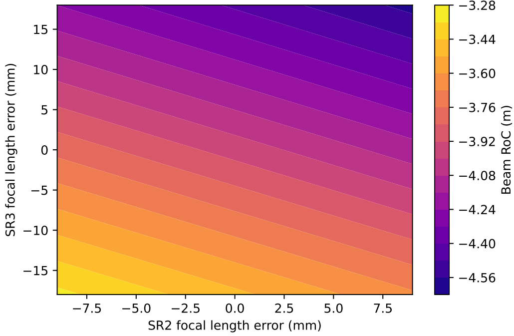
Figure 7.6: The RoC of the beam that is transmitted through the SRM as a function of the error ( \pm 3\sigma ) in focal length of SR3 and SR2. If the arm cavities and the SRC are well mode matched, then the RoC of the beam transmitted through the SRM would be \frac{5.67\text{m}}{1.45} = 3.91\text{m} . When the SR3 focal length error > 6 mm and SR2 error is zero the SRC cavity is unstable (see figure 7.9), so this area of the parameter space is unlikely to correspond to the beam at the SRM at LLO.
