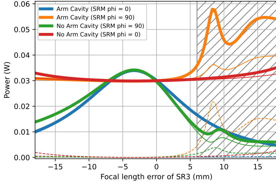
Figure 7.13: The total power transmitted through the SRM for each simulation, is shown in the thick pale lines. The thin solid lines corresponds to the power in the HG00 mode, and the thin dashed lines correspond to the power in the higher order modes. Blue lines show the behaviour when the interferometer has arm cavities and is in signal recycling mode, and the orange lines shows when it is in RSE mode. Green lines show how the power changes when the interferometer is configured for a single bounce measurement and is in signal recycling mode, and the red line shows when its in RSE mode. The hatched region indicates where the SRC is becomes unstable, and so the behaviour of the interferometer cannot be accurately simulated for these values of focal length.
