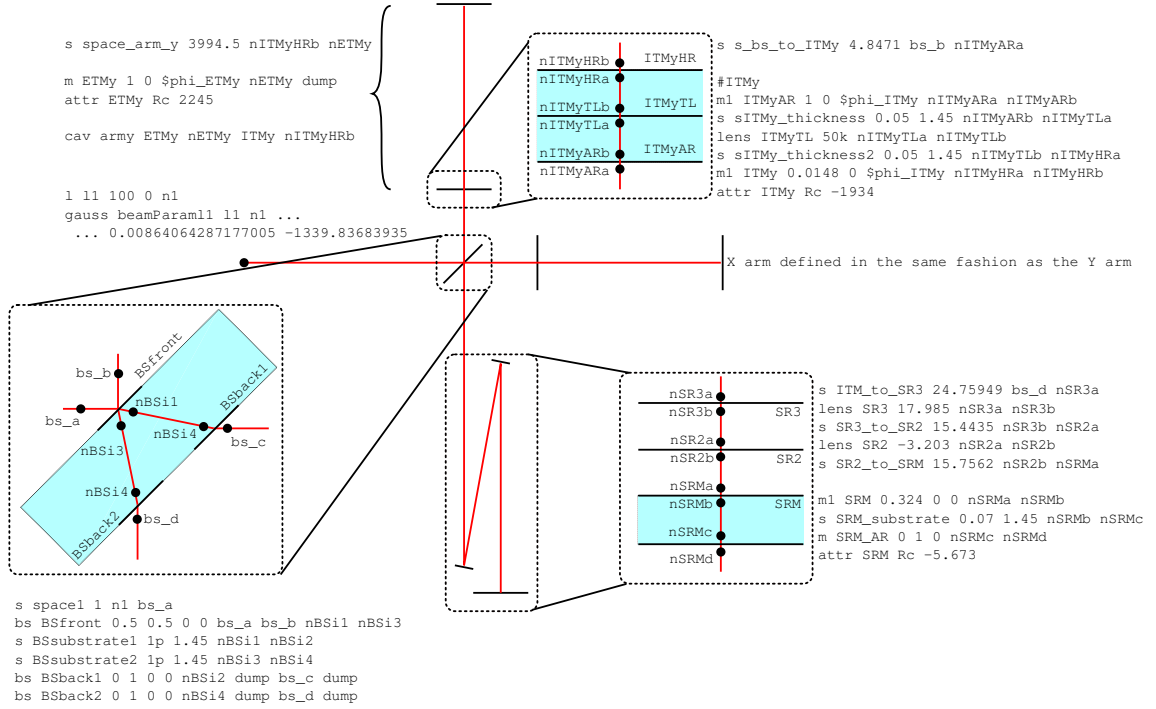
Figure 7.2: Schematic of the simulation. The dimensions of the schematic are not to scale. The laser light is shown as a red line. Black lines with red beams interacting with them corresponds to components such as mirrors and lenses. Important nodes are highlighted with black dots and the associated FINESSE commands are shown nearby. Zoom-ins provide more detail for the main beam splitter, ITMy and the SRC. The elongated curled bracket highlights the arm cavity, and the text with it shows how it is implemented in FINESSE.
