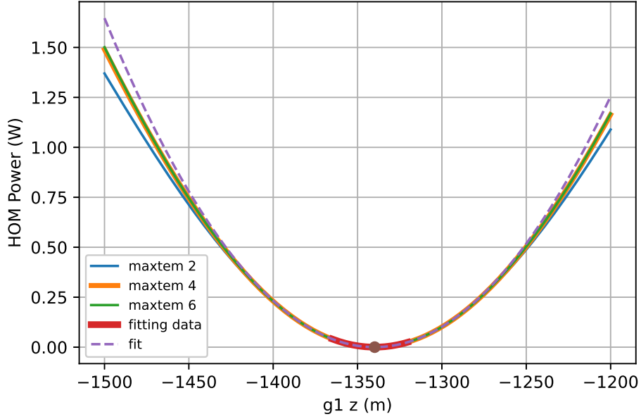
Figure A.1: Optimisation of parameters used in the gauss command to mode match the laser to the arms in the simulations described in chapter 7 and section A.3. The blue, green and orange lines show how the mode matching changes as the beam waist location is changed. As the mode matching becomes larger, more HOM are required, as the blue and green/orange lines diverge. A quadratic was fitted to the data highlighted in red, and the minimum value was used as the waist location parameter for the gauss command.
