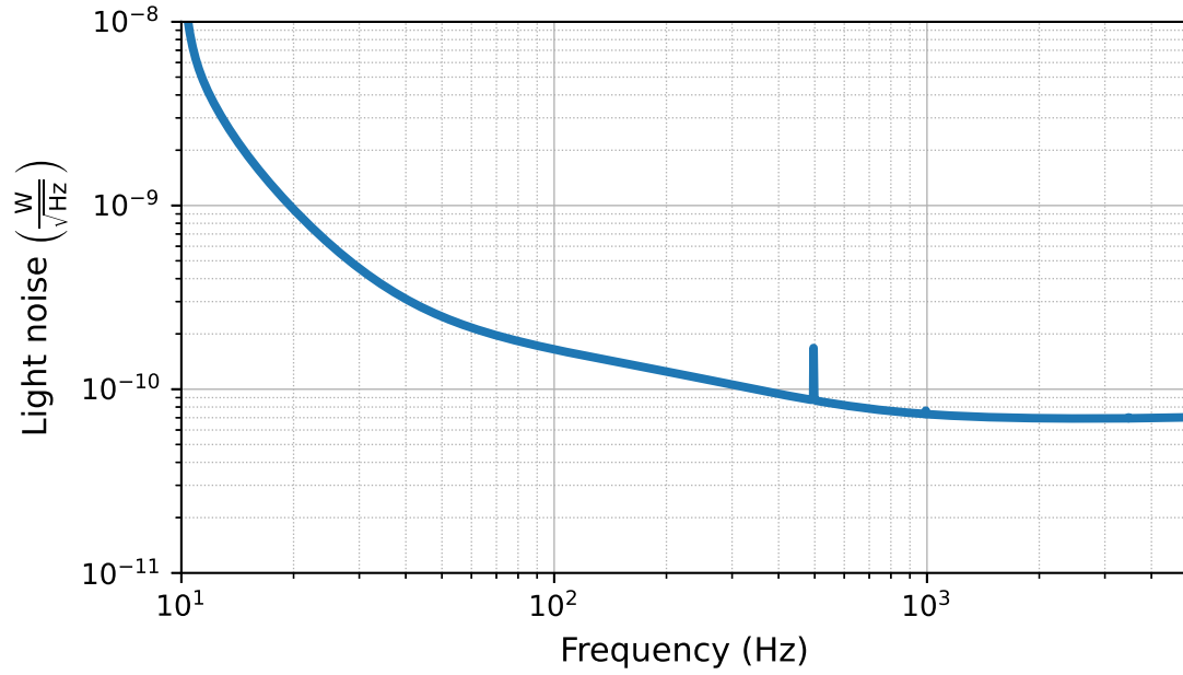
Figure 8.4: The intensity noise of the light at the AS port for the A+ detector. This was obtained by deconvolving the detectors sensitivity curve with the function shown in Figure 8.3. At frequencies above 1 kHz the noise is flat as it is dominated by shot noise. At lower frequencies the noise is increased relative to shot noise due to radiation pressure, coating thermal noise and other noise sources. The spike in the spectrum at 500Hz represents the presence of suspension modes ( actually find out what this is ).
