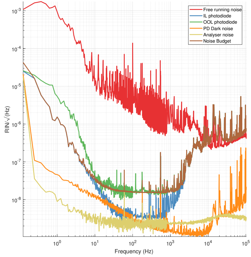
Figure 6.1: Free running and stabilised noise of laser
