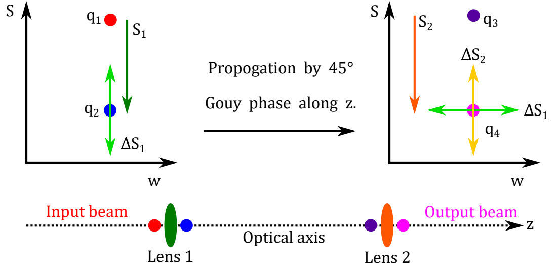
Figure 9.5: Sketches of the WS representation for a Gaussian beam interacting with different parts of a simple optical layout consisting of two active lenses with powers S_{1,2} \pm \Delta S_{1,2} . The left hand axis shows the WS plane at Lens 1. The input beam q_1 is indicated by a red dot, and the effect of the lens on q_1 is shown by the dark green arrow S_1 . This results in a new mode q_2 which is shown as a blue dot. A light green arrow indicates the actuation of Lens 1. The right hand axis shows the WS plane at Lens 2. The input mode at Lens 2, q_3 , is shown as a purple dot, and the output mode, q_4 , is shown as a pink dot. The static and dynamic power of Lens 2 is indicated by the orange and yellow lines. As Lens 1 and Lens 2 are separated by 45^\circ of Gouy Phase, the actuation provided by Lens 1 results in a change in the beam parameter which is orthogonal to the actuation provided by Lens 2, provided that the actuations are small enough. Beneath the two WS space diagrams is a sketch of the optical axis and where the modes are along it.
