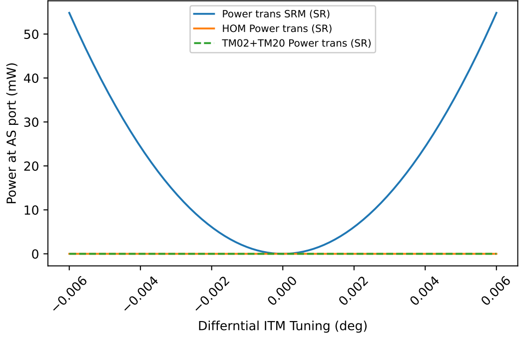
Figure 7.4: The minimum of the dark fringe is at 0^\circ differential ITM detuning, as shown by the blue line. A slight offset causes light to be as the AS port. This result was used to determine tunings for simulating what effect focal length errors in SR3 and SR2 have on the beam transmitted through the SRM. The orange and green dashed line show the HOM content of the beam.
