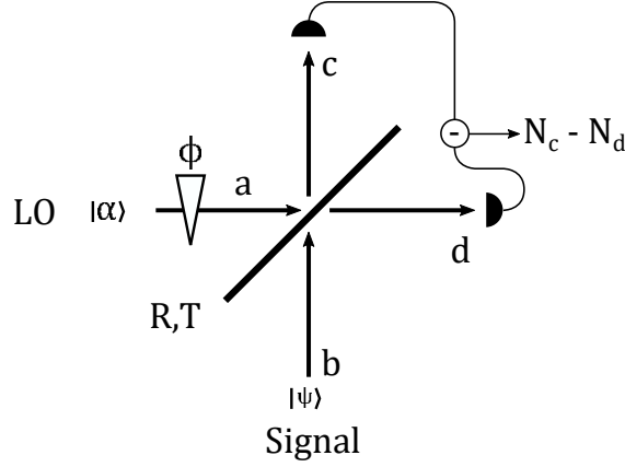
Figure 8.1: A coherent state |\alpha\rangle , enters port a of a beam splitter. A signal |\Psi\rangle enters port b . These two beams interfere, resulting in photons being detected at the c and d ports. The two photo-currents are subtracted, and the signal that is produced is proportional to an arbitrary quadrature of the state |\Psi\rangle . The quadrature that is measured is determined by the homodyne angle, \phi . This is expressed mathematically by equation (??).
