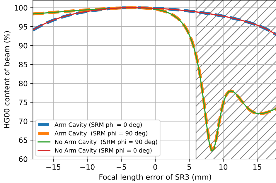
Figure 7.12: The percentage of light which is in the HG00 mode as the focal length of SR3 changes compared to the total light power does not depend on whether there are arm cavities. It is determined by the detuning of the SRM. The blue dashed line shows the behaviour of the beam with arm cavities present and with the SRC in signal recycling mode (SRM \phi = 0^\circ ). The red line shows how the beam changes with focal length error for a single bounce measurement and with the SRC in RSE mode (SRM \phi = 90^\circ ). The orange dashed line corresponds to the interferometer having arm cavities and being in RSE mode (SRM \phi = 90^\circ ). The green line shows behaviour of the beam when the interferometer is configured for a single bounce measurement and is in signal recycling mode. The hatched region indicates where the SRC becomes unstable (see figure 7.9), so the behaviour of the interferometer cannot be accurately simulated for these values of focal length.
