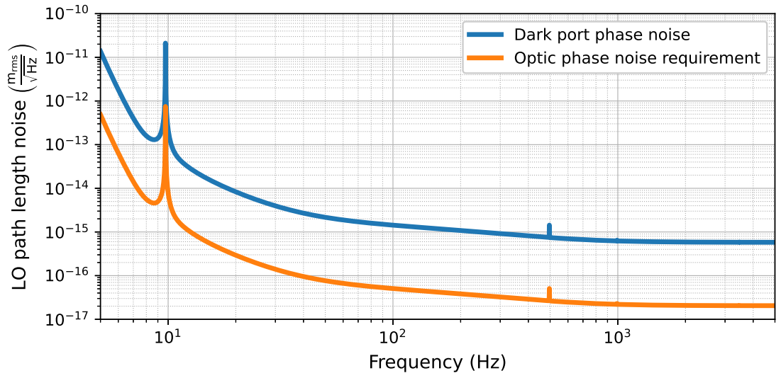
Figure 5.5: The sensitivity curve for A+ sets the limit on the amount of path length noise that is acceptable between the AS and LO beams. The blue line shows sensitivity curve in units of path length noise between the AS and LO beams, and the orange line shows the longitudinal motion requirement for the optics which combine the LO and signal beam. At 5 Hz, the longitudinal motion requirement for the optics is 4.9 \times 10^{-13} \text{ m}_{rms}/\sqrt{\text{Hz}} .
