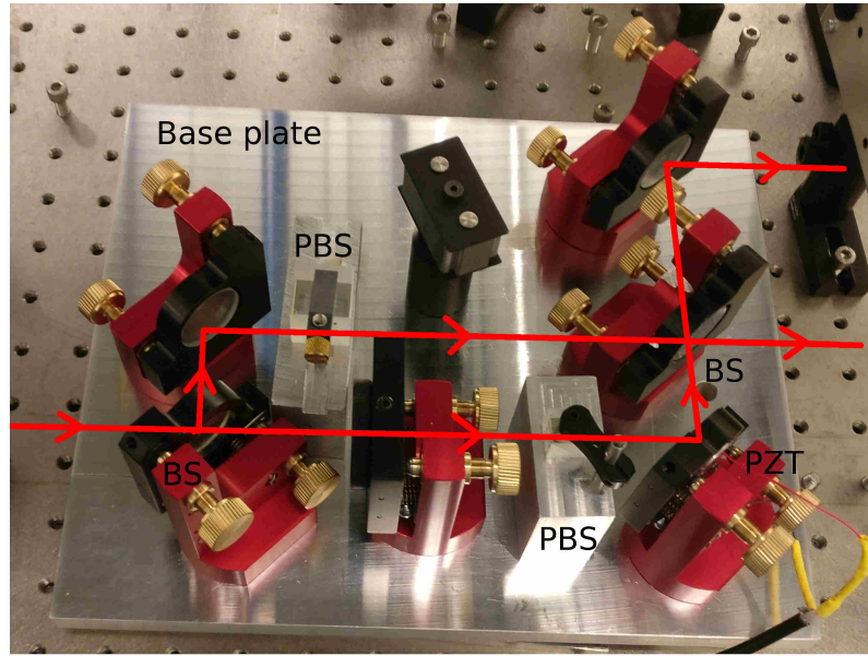
Figure 7.2: Photograph of the Mach-Zehnder base plate. The polarising beam splitters were part of an earlier design; they were removed when the measurements with this apparatus were made.
