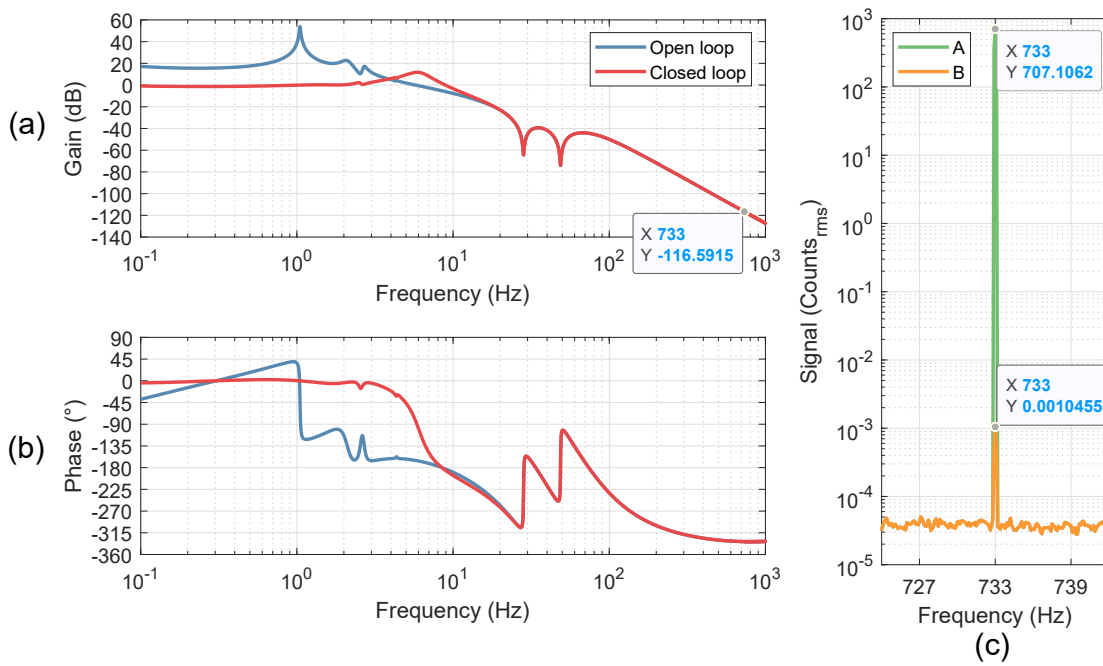
Figure 7.11: Panel (a) and Panel (b) show the Servo's open and closed-loop transfer function. This was calibrated using the factors from 7.1. Panel (c) shows a measurement where a signal was injected at point A in the servo and measured at point B (see Figure 7.10); these two points are separated by a times one block, and so the ratio of these signals represents the closed-loop transfer function of the servo. These measurements are in agreement with the model to within 0.1 dB.
