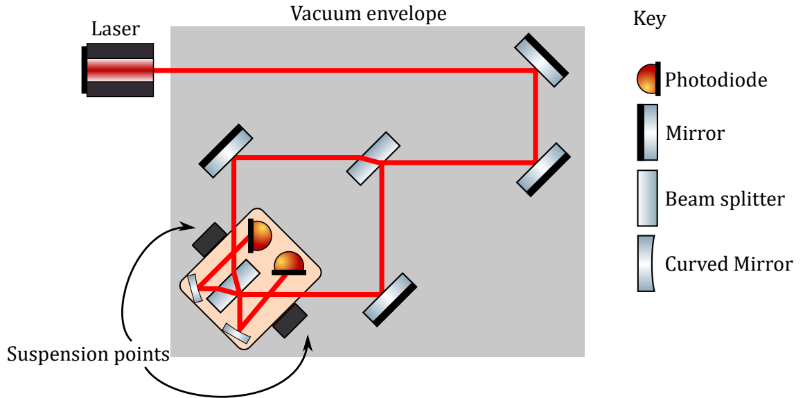
Figure 7.8: Sketch of the in-vacuum Mach-Zehnder. Laser light entered the vacuum system and was steered by suspended optics into a Mach-Zehnder interferometer. The first beam splitter and the two corner mirrors were in identical suspensions. The suspensions are described in Section 7.2.1. The beam splitter for recombining the beam was part of a larger suspended assembly which also included steering mirrors and the photodiodes. Photographs of the components are shown in Figure 7.9. The mirrors and the beam splitter were suspended with identical suspensions, and the recombining beam splitter was part of a larger assembly.
