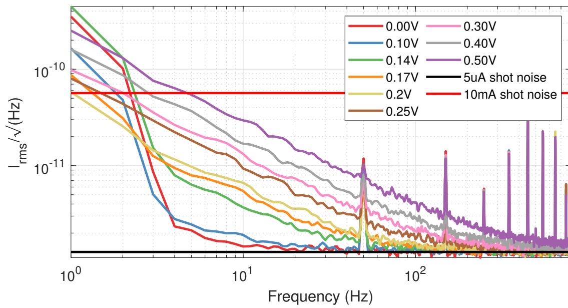
Figure A.15: The noise of the photocurrent produced by the P5968 as a function of bias.
