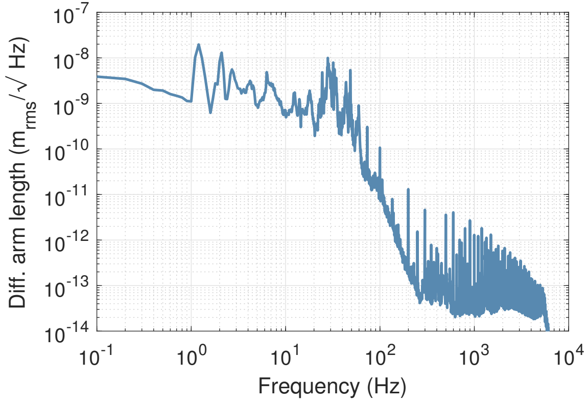
Figure 7.12: Scattering caused there to be a high level of noise in the differential arm length signal. Many peaks related to the balanced homodyne detector suspension can be seen around 30 Hz, and this motion generated phase modulations in the scattered light. The noise was caused by the interference between the scattered light and the signal-carrying light on the photodiodes. For this measurement, shot noise would have been at \sim 10^{-15} \text{ m}/\sqrt{\text{Hz}} .
