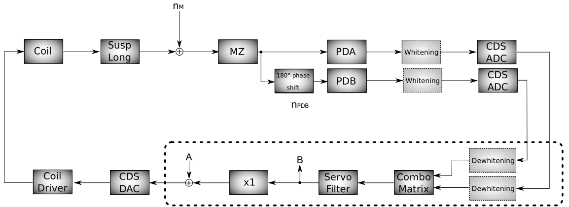
Figure 7.10: Flow diagram showing each block of the servo used to lock the in-vacuum Mach-Zehnder. The digital part of the servo is shown in the dashed area. The injection points A and B were used to calibrate the servo (see Figure 7.11) are around a times one block. The mirrors motion that the servo must correct for is represented by the signal n_M . The information about the Mach-Zehnder differential arm length is encoded by two signals that are 180^\circ out of phase. The whitening and dewhitening filters are paler as these do not affect the gain of the loop.
