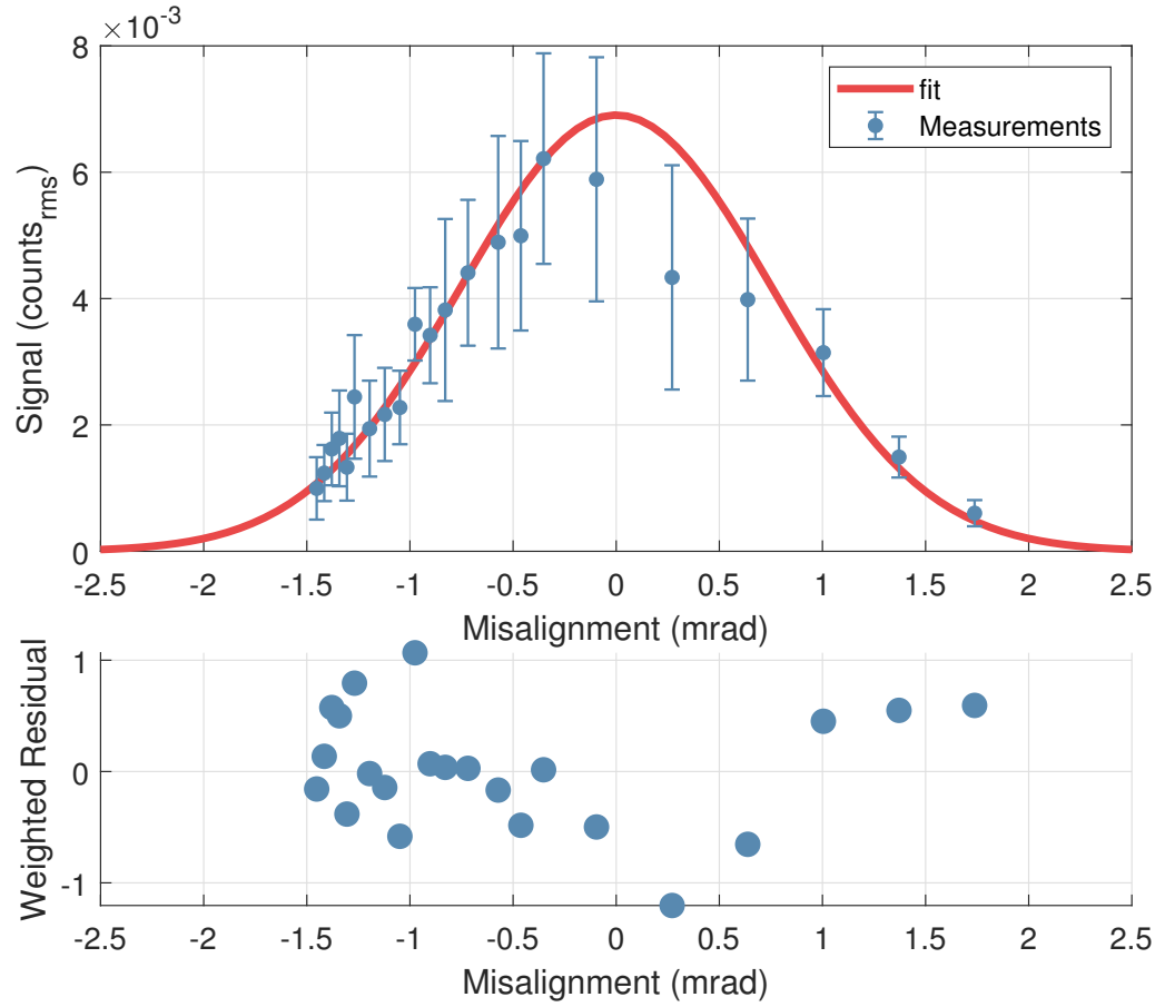
Figure 7.13: Top panel: As the Mach-Zehnder was misaligned, the signal due to the differential arm length modulation decreased. The blue points show the measured signal as a function of misalignment. The data was fit to Equation (7.2), and this is shown in red. Bottom panel: the weighted residuals of the measurements to the fit show no pattern, indicating that the model used was appropriate.
