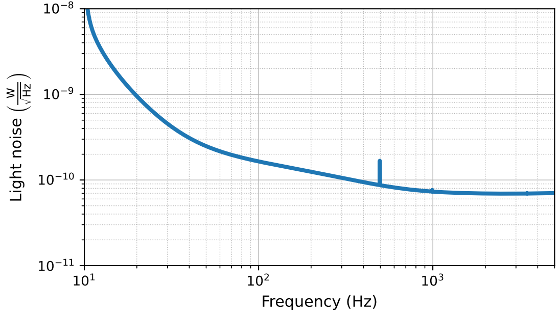
Figure 1.4: The intensity noise of the light at the AS port for the A+ detector. This was obtained by deconvolving the detectors sensitivity curve[23] with the function shown in Figure 1.3. At frequencies above 1 kHz the noise is flat as it is dominated by shot noise. At lower frequencies the noise is increased relative to shot noise due to radiation pressure, coating thermal noise and other noise sources. The spike in the spectrum at 500Hz represents the presence of suspension thermal noise (?).
