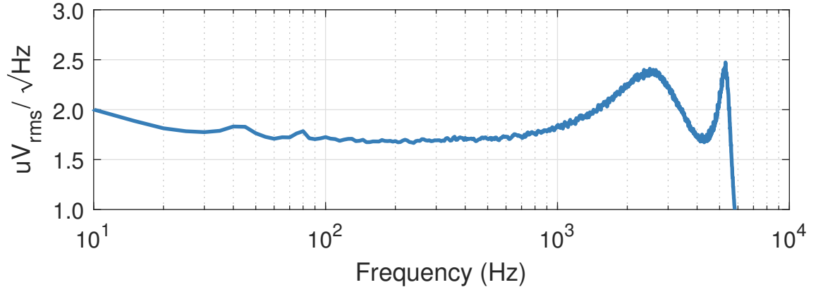
Figure C.2: Voltage noise at the input of the Glasgow CDS system
