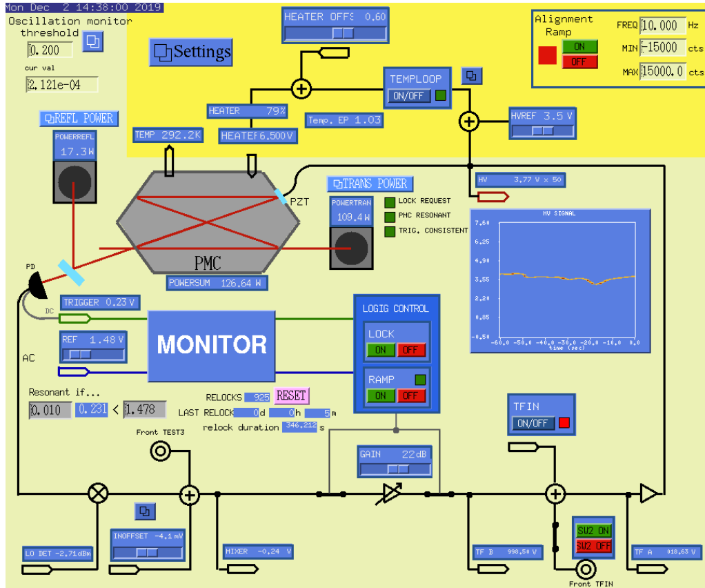
Figure C.1: The MEDM screen used to lock the PMC.
