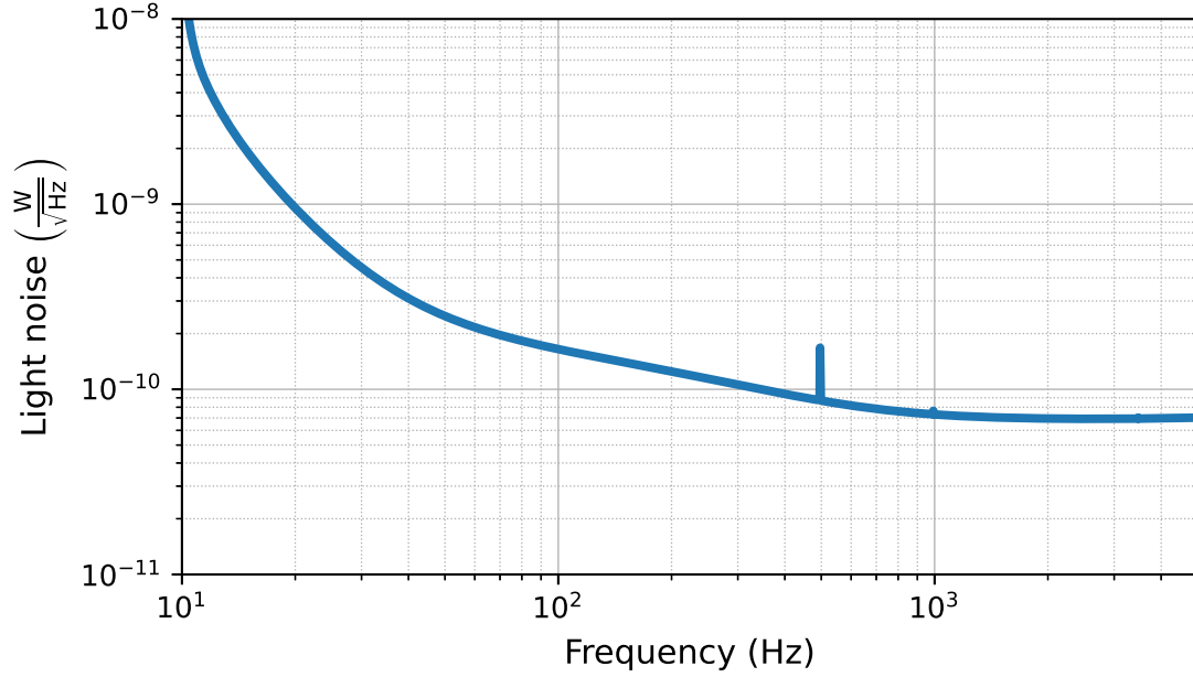
Figure 1.4: The intensity noise of the light at the AS port for the A+ detector. This was obtained by deconvolving the detectors sensitivity curve[11] with the function shown in figure 1.3. At frequencies above 1 kHz, the noise is flat as it is dominated by shot noise. At lower frequencies, the noise is increased relative to shot noise due to radiation pressure, coating thermal noise. The spike in the spectrum at 500Hz represents the presence of suspension thermal noise (?).
