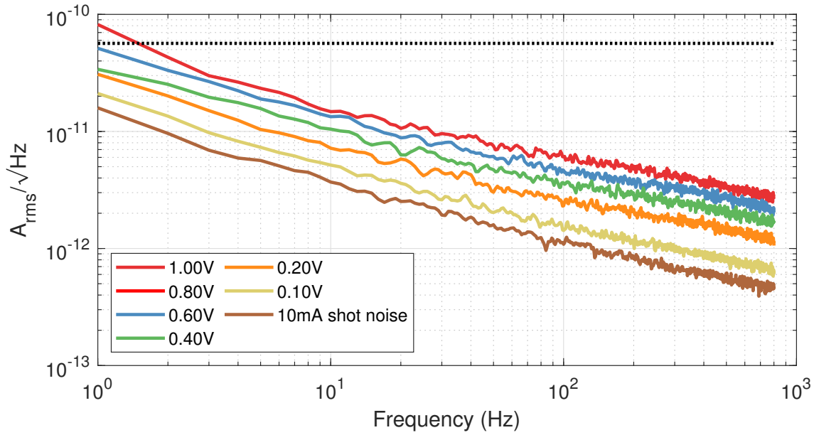
Figure A.6: Dark noise of the G12182-010k at 22°C for a series of reverse biases.
