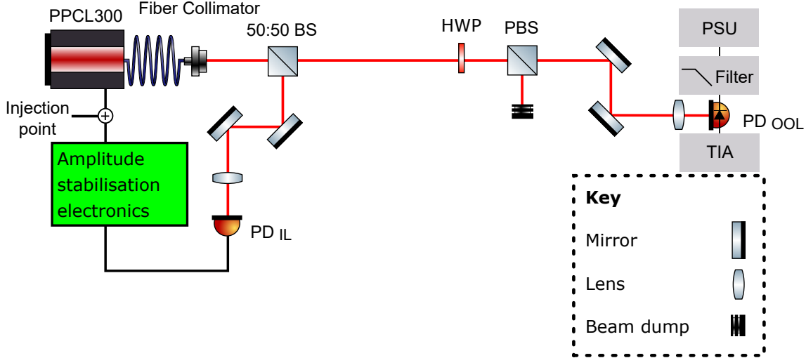
Figure 7.1: Optical layout used for measuring the effect that increasing the reverse bias of a photodiode had on its quantum efficiency and saturation limit. The out-of-loop photodiode, \text{PD}_{\text{OOL}} , was the photodiode under test (FD10D). A 1.55\mu\text{m} laser was used to assess the optical properties of the photodiode. A combination of half wave plate (HWP) and polarised beam splitter (PBS) allowed for the power of the beam to be set, and a lens was used to set the size of the beam on the photodiode under test. Amplitude stabilised light was needed to ensure the increase in photocurrent seen when the bias was increased was due to an improvement in quantum efficiency. The photodiode circuit (TIA) (see Appendix B.2) allowed for shot noise limited measurements of current around 10\text{mA} and for the bias to be selected. The calibration signal was added onto the amplitude stabilisation error signal.
