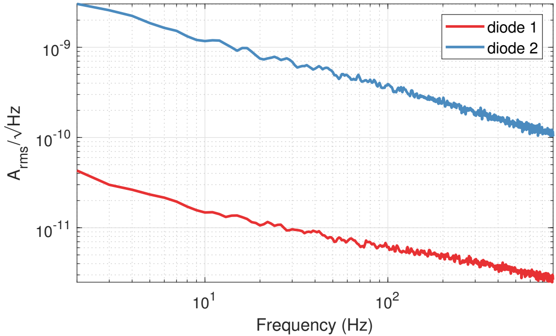
Figure 7.7: The difference in dark noise between two nominally identical photodiodes (g12182-010k) under the same operating conditions (room temperature at 1 V bias). Photodiode 1 performs nearly 100 times better than photodiode 2. For the duration of this experiment, the photodiodes were handled with suitable ESD precautions. This difference in noise may be explained by differing numbers of defects or by ESD damage prior to purchase.
