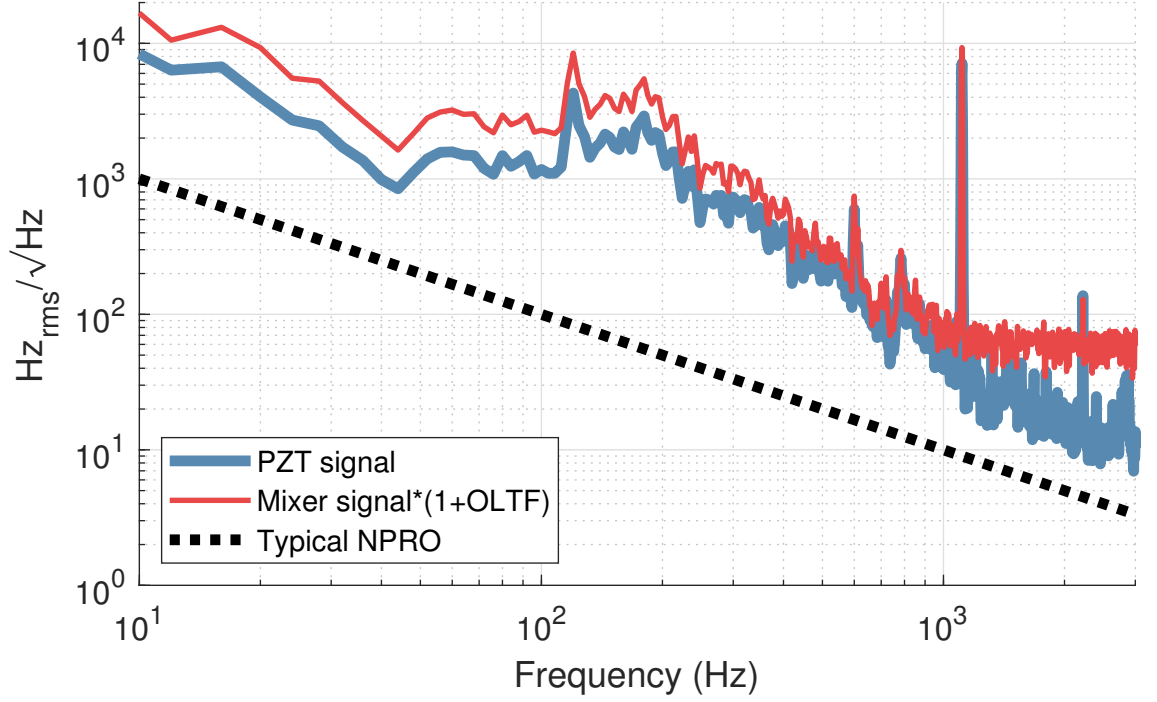
Figure 2.29: The mixer signal combined with the open-loop transfer function is shown in red. This is equivalent to the frequency noise of the system. The PZT signal should agree with this measurement below the unity gain point ( \sim 800 Hz). A signal was applied to the PZT at 1111 Hz. This is below the corner frequency of the PZT and above the unity gain point for the servo. This should match with the mixer signal. There is a factor of two between these two measurements. This can be attributed to imperfect calibration due to nominal parameters of the PMC being used. The typical noise expected from an NPRO is shown by the dashed black line. Between 100 Hz and 1000 Hz, there is a bulge in the frequency noise. This is likely due to acoustically driven noise of the PMC as the PMC is not vacuum sealed. This can be converted to length noise with a factor of \sim 10^{-14} m/Hz.
