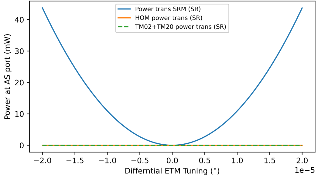
Figure 3.4: The minimum of the dark fringe is at 0^\circ differential ETM detuning, as shown by the blue line. A slight offset causes light to be at the AS port. This result was used to determine tunings for simulating what effect focal length errors in SR3 and SR2 have on the beam transmitted through the SRM. The orange line and dashed green line show that the beam has a negligible HOM content.
