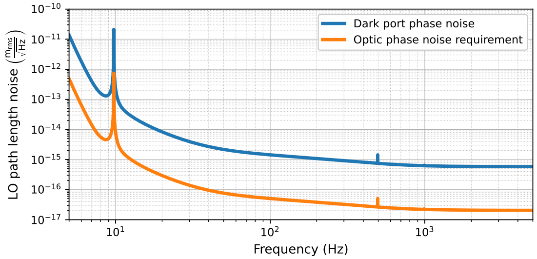
Figure 4.5: The sensitivity curve for A+ sets the limit on the amount of path length noise that is acceptable between the AS and LO beams. The blue line shows sensitivity curve in units of path length noise between the AS and LO beams, and the orange line shows the longitudinal motion requirement for the optics which combine the LO and signal beam. At 5 Hz, the longitudinal motion requirement for the optics is 4.9 \times 10^{-13} \text{ m}_{\text{rms}}/\sqrt{\text{Hz}} .
