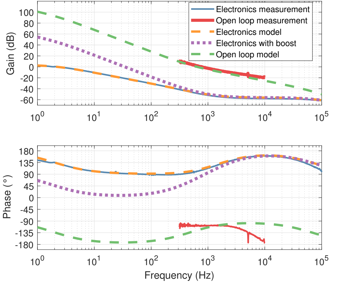
Figure 2.28: The open-loop transfer function was measured using the layout shown in Figure 2.24. This is shown in red. The transfer function of the electronics without the ‘boost’ provided by an extra integrator stage was measured and is shown in blue. The model of this is shown in orange. The boosted electronics model is shown in purple. The green line shows the expected servo gain based on the boosted electronics model and the measurements shown in Figures 2.26 and 2.27. This model is within 2 dB of the measurement above the unity gain point. The PZT inducing unintended motion in the cavity as it goes through resonance may explain the phase a gain discrepancy between the model and the measurement below the unity gain point. The unity gain point was measured to be at \sim 800 Hz.
