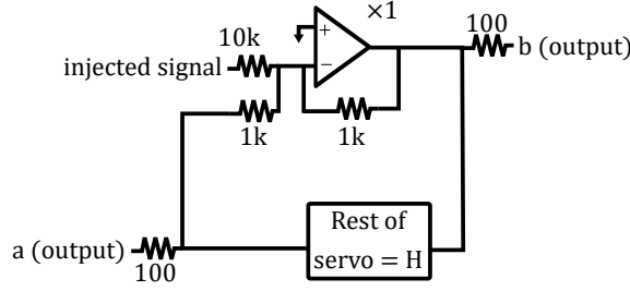
Figure 2.18: The transfer function of every component except in the loop is represented by the block labelled H . A signal was injected at a unity gain summing point in the servo. The signals a and b were measured, and as a = bH , the ratio a/b = H .
