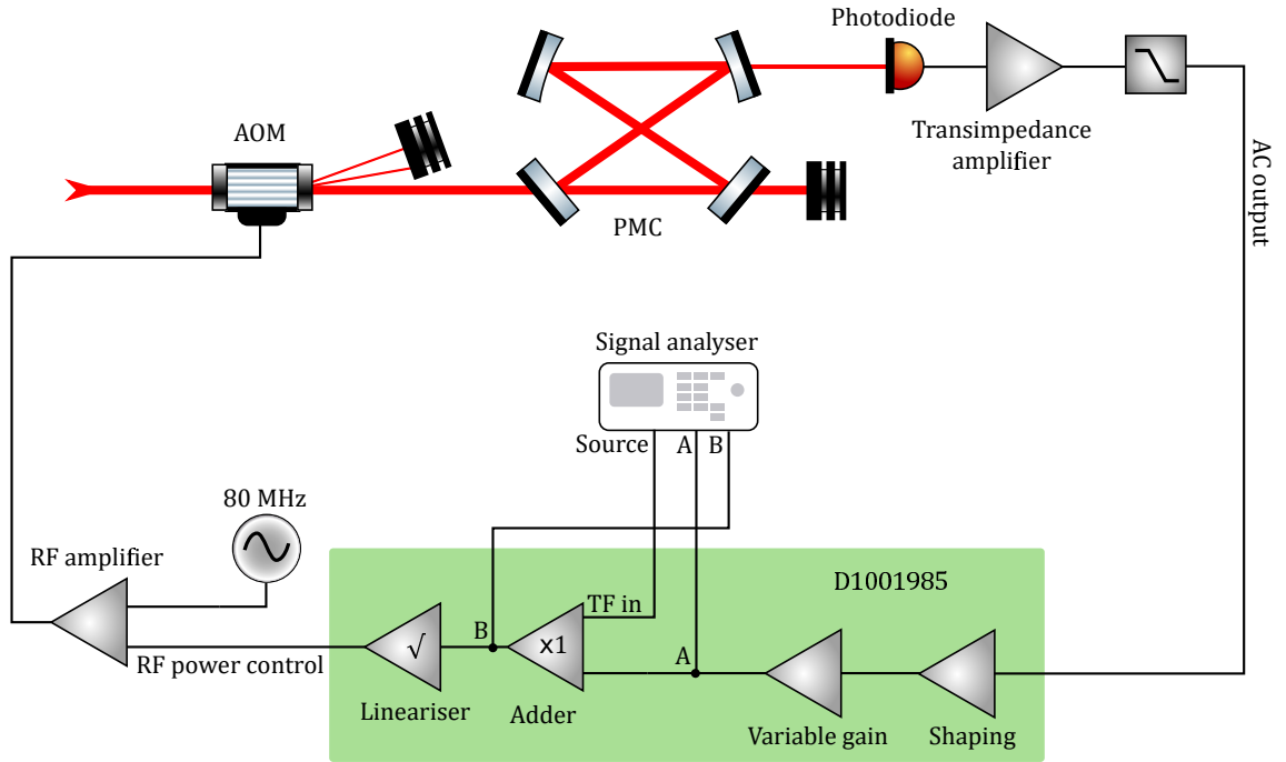
Figure 2.19: Sketch of the amplitude stabilisation servo. By measuring the ratio of the signal at point B and point A, the transfer function of all the parts in the servo (apart from the \times 1 adding stage) can be measured (see Figure 2.18).
