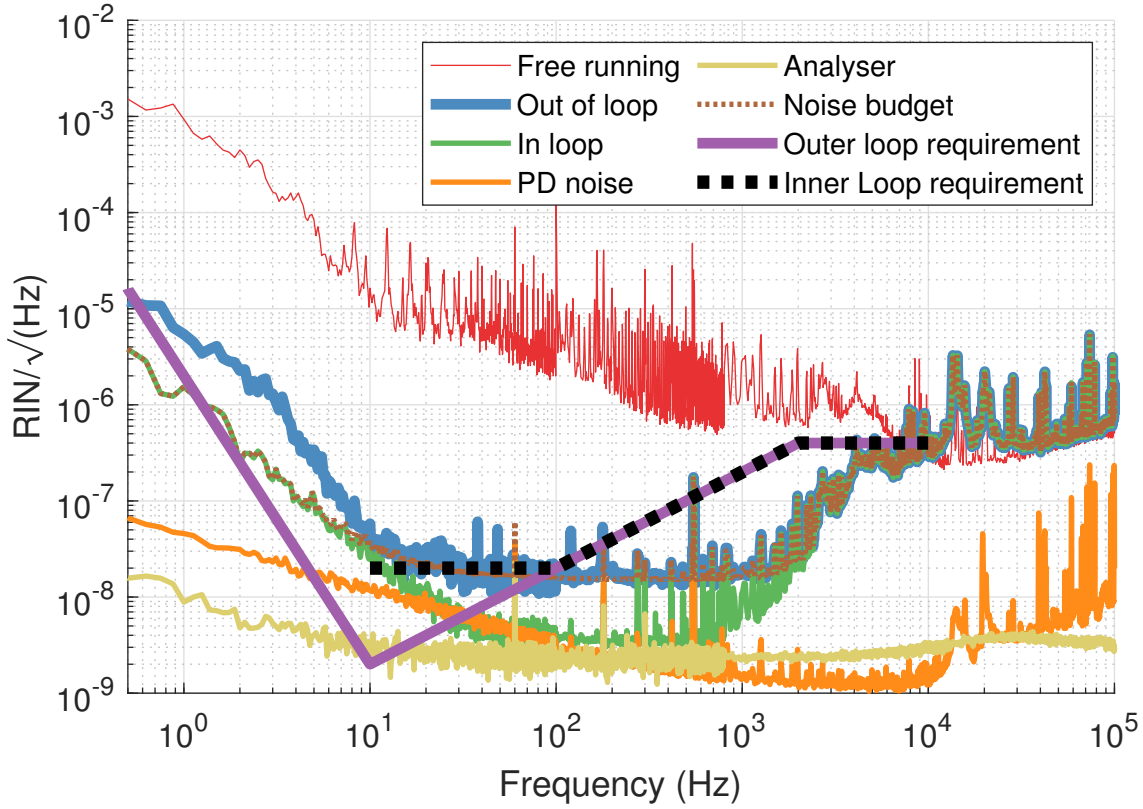
Figure 2.22: The free-running noise of the laser is shown in red. The noise of the light transmitted by the PMC is shown in blue; this meets the requirement that is shown by the dashed black line. The noise level is determined by the in loop noise, shown in green, the shot noise and other technical noise sources; the sum of these is shown by the dotted brown line. Between 10 Hz–100 Hz, the noise of the laser is limited by shot noise. There is a discrepancy between the noise budget and the measured noise. This is likely due to dust falling through the beam or scattered light. Near the unity gain point of the servo, the noise is enhanced by the servo due to gain peaking.
