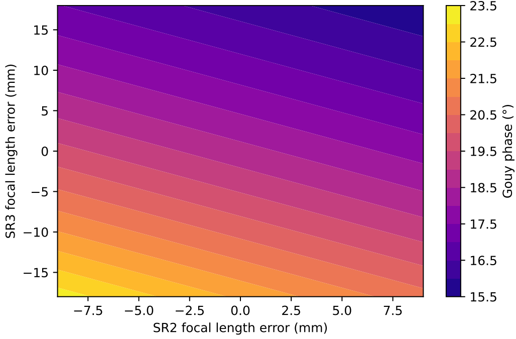
Figure 3.8: The Gouy phase between the ITMs and the SRM as a function of the error ( \pm 3\sigma ) in SR3 and SR2. When the SR3 focal length error > 6 mm and SR2 error is zero, the SRC cavity is unstable (see Figure 3.10), so this area of the parameter space is unlikely to correspond to the beam at the SRM at LLO.
