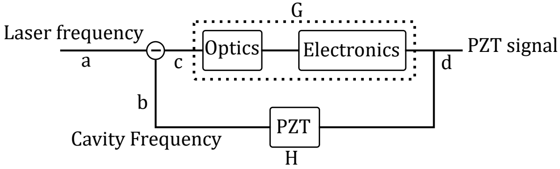
Figure 2.25: The servo can be considered as being made of three parts: the optics, the shaping electronics and the PZT. The transfer function of the optics represents how a difference in frequency between the laser and the cavity transforms into a signal after the demodulator. When at resonance and below the cavity pole, this is a flat transfer function that is proportional to the difference in frequency. Since this cavity pole is in the 1 MHz region and this measurement will only go to the kHz region, the cavity pole can be ignored. The transfer function of the electronics includes everything after the demodulator up to and including the final high power op amp. The PZT transfer function converts a voltage to a cavity frequency. The PZT has capacitance, so a low pass filter is formed by this and the series resistor at the output of the electronics.
