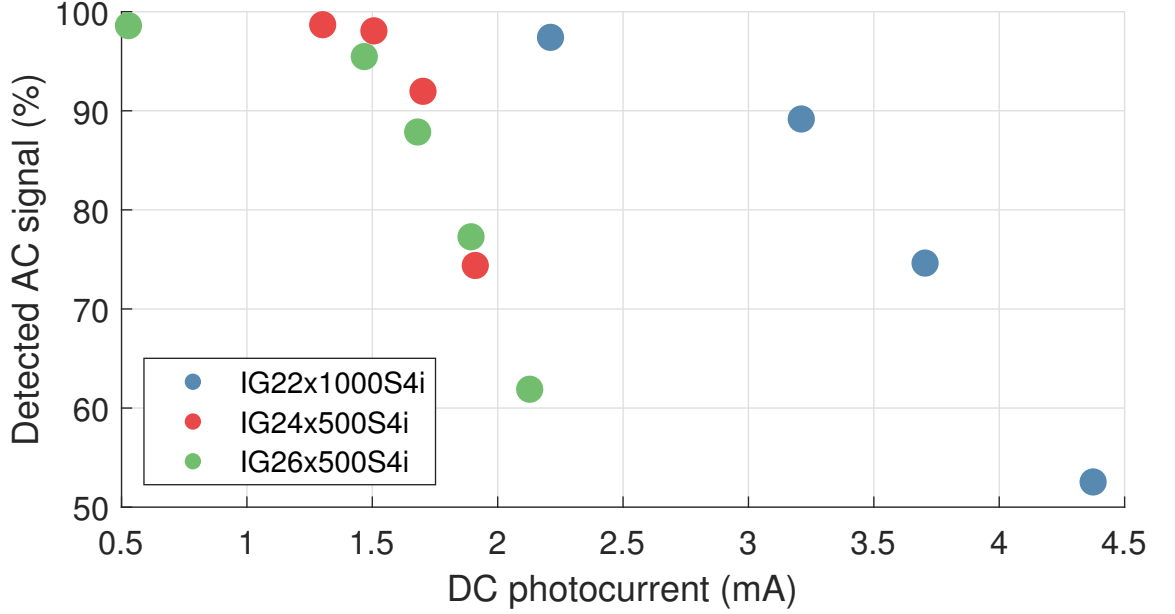
Figure 6.10: The saturation limit of the IG22x1000S4i, IG24x500S4i and IG26x500S4i photodiodes was measured. The photodiodes were biased so that their noise at 10 Hz was equal to the shot noise of a 10 mA current. The IG24x500S4i and IG26x500S4i were exposed to a beam with a 3\sigma width of 220 \mu\text{m} and the IG22x1000S4i was exposed to a beam with a 3\sigma width of 1000 \mu\text{m} . The size of the light modulation of known size was tracked as the DC photocurrent was increased. As the photodiodes saturated, the relative size of the AC signal decreased. The uncertainty in these measurements was \pm 1\% . These photodiodes had low saturation limits compared to the FD10D, which showed no signs of saturation up to 16.5 mA (see Figure 6.4).
