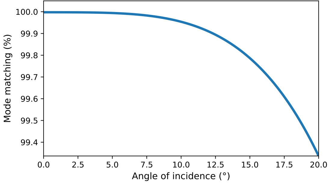
Figure 5.3: Astigmatism is a source of loss. When designing the layout shown in Figure 5.1, the AOI for the curved mirrors was altered to explore how sensitive it was to astigmatism. Using Equation (5.2), the loss was computed. This effect is negligible up to 10^\circ after which it starts to become significant compared to the losses summarised in Table 5.2.
