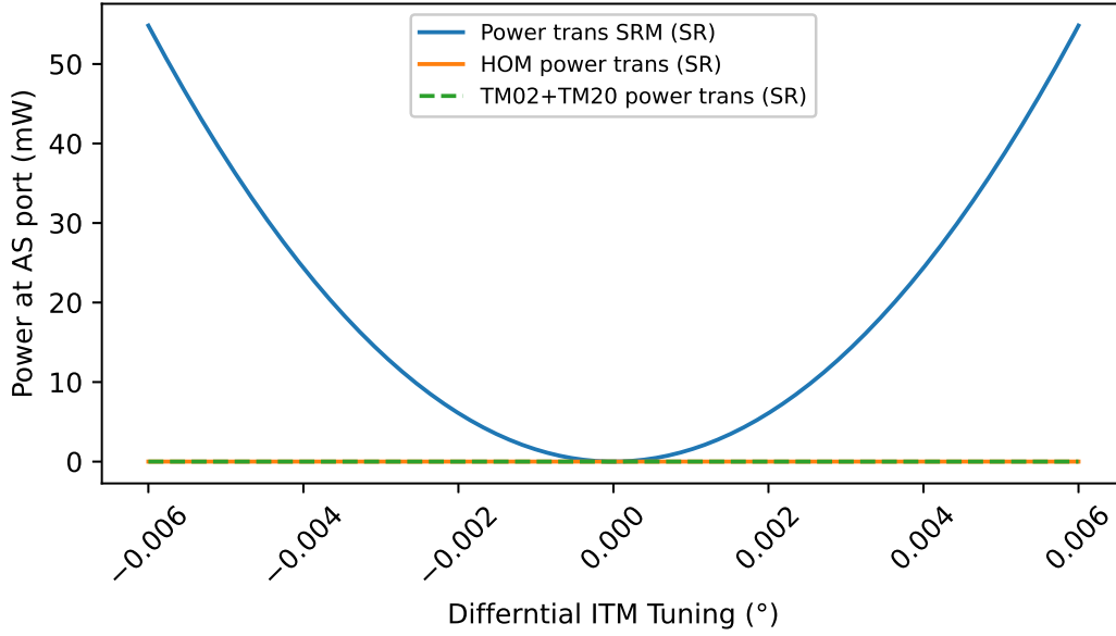
Figure 3.5: The minimum of the dark fringe is at 0^\circ differential ITM detuning, as shown by the blue line. A slight offset causes light to be at the AS port. This result was used to determine tunings for simulating what effect focal length errors in SR3 and SR2 have on the beam transmitted through the SRM. The orange line and dashed green line show that the beam has a negligible HOM content.
