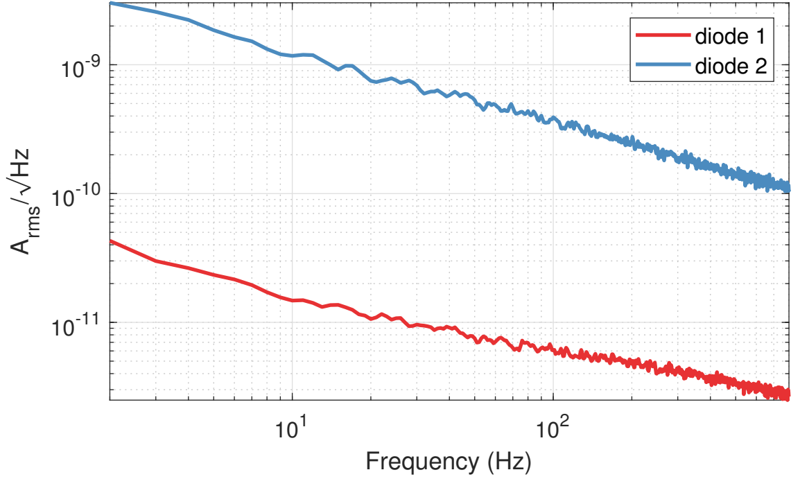
Figure 6.7: The difference in dark noise between two nominally identical photodiodes (g12182-010k) under the same operating conditions (room temperature at 1 V bias). Photodiode 1 performs nearly 100 times better than photodiode 2. For the duration of this experiment, the photodiodes were handled with suitable ESD precautions. This difference in noise may be explained by differing numbers of defects or by ESD damage prior to purchase.
