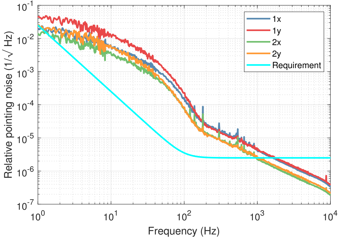
Figure 2.23: The four relative pointing degrees of freedom for the beam into the PMC was measured with the DBB. The requirement [128] is shown in light blue. The pointing noise is above the requirement, however the TnT lab has a higher amount of environmental noise than the PSL. Measurements below 200 Hz were be affected by scattering.
