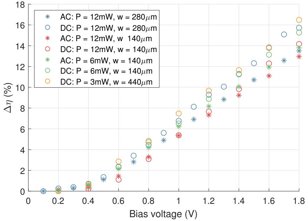
Figure 6.2: The FD10D’s quantum efficiency depends on its reverse bias; the increase in quantum efficiency was 15 \pm 1\% when the bias was increased to the maximum value specified in its datasheet. Two types of measurement were used to determine the increase in quantum efficiency as the bias was increased. The first method was to measure the photocurrent with a voltmeter as the bias was increased, and the corresponding results are shown as circles (‘DC’). The second method involved modulating the bias and measuring the resulting modulation in the photocurrent, i.e. an AC measurement, and these are shown by the stars. Each set of measurements was done with a different intensity by changing either the beam’s width or power. Further detail on both methods is given in Section 6.4.1.
