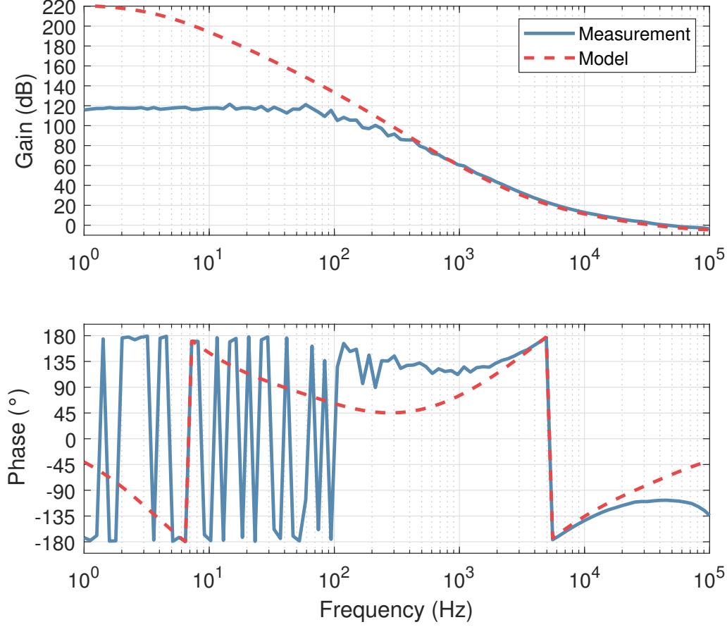
Figure 2.20: The open-loop transfer function was measured using the layout shown in Figure 2.19. The unity gain point is at 48 kHz with 70^\circ of phase margin. The shaping of the servo is 1/f at the unity gain point, but to achieve higher gain at low frequency, the servo has a 1/f^3 slope between 10 Hz—5 kHz. The measurement saturated below 100 Hz. The model and measurement do not agree well below a few kHz due to the measurement saturating.
