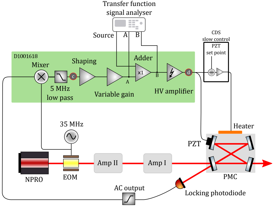
Figure 2.24: A sketch of the servo for locking the PMC. An EOM creates 35 MHz sidebands which are used to produce a PDH locking signal. A PZT controls the length of the cavity at high frequencies. A heater and a digital loop is used to provide slow control that corrects for frequency drifts associated with change in the NPRO temperature and the room temperature. This is required as otherwise the PZT would run out of range. The open-loop transfer function was measured using signals at A and B. The frequency noise was measured using the error point and control signals marked by c and d , with this notation corresponding with the notation in Figure 2.25 and Equation (2.1).
