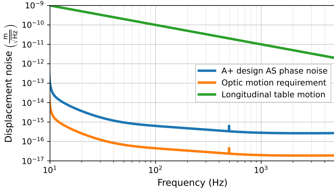
Figure 1.6: The phase noise between the LO and the AS beams causes noise. The sensitivity curve for A+ sets the limit on how much path length noise is acceptable between the AS and LO beams. The blue line shows sensitivity curve is shown in units of path length noise between the AS and LO beams, and the orange line shows the requirement of HRTS mirror motion. The table motion was modelled as 1/f noise.
