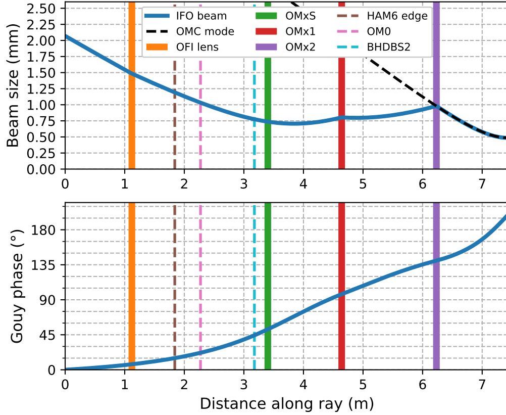
Figure 1.8: Top panel: the radius of the beam as it travels from the SRM ( z = 0 ) to the waist of the OMC. Significant points along the axis are marked with vertical lines. Less significant, but useful reference points, are marked by dashed vertical lines. Bottom panel: The gouy phase shift accumulated by the beam as it propagates along the optical axis.
