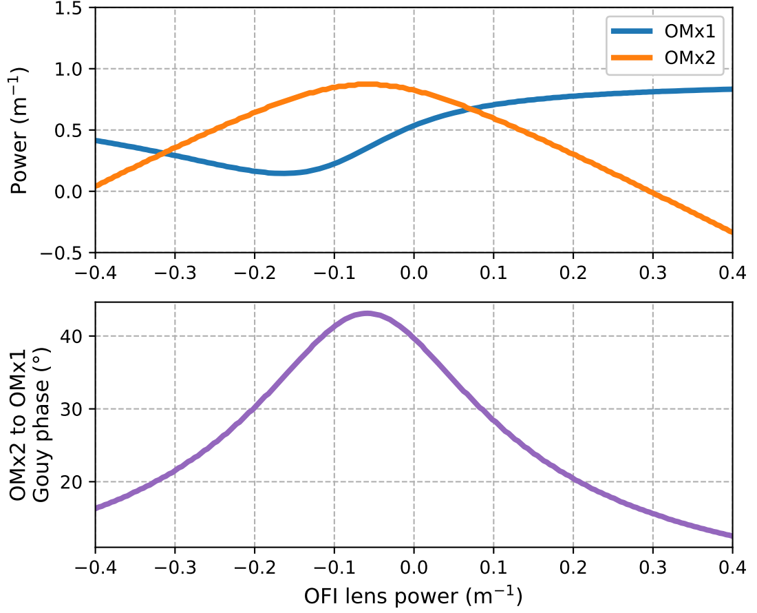
Figure 1.9: Top panel: The choice of OFI lens power effects the combination of OMx1 and OMx2 power required for 100% mode matching. Bottom panel: The best choice of OFI lens corresponds to where the Gouy phase separation between the pair of OMx1 and OMx2 mirrors that give 100% mode matching is closest to 45^\circ . The optimal Gouy phase separation between OMx1 and OMx2 achievable by this layout is 43^\circ .
