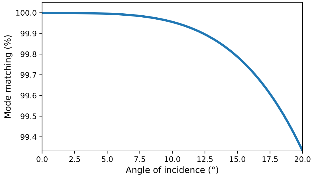
Figure 1.10: Astigmatism is a source of loss. When designing this layout, to explore how sensitive it was to astigmatism, the AOI for the curved mirrors was altered. Using equation 1.16, the loss was computed. This effect is negligible up to 10^\circ , after which it starts to become significant compared to the losses summarised in table 1.1.
