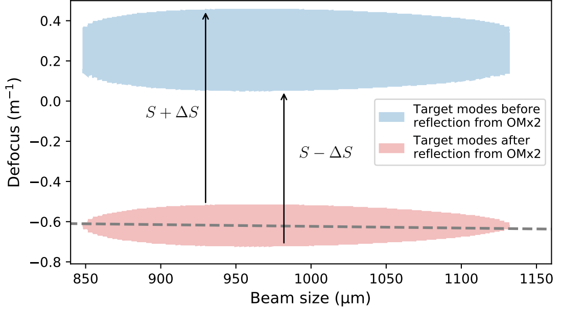
Figure 1.12: This is the WS space at the OMx2 plane. The effect of OMx2 in the plane of OMx2 is to move a mode vertically in WS space. After reflection from OMx2, a mode must be at least 98% mode matched to the OMC as there are no further active mode matching elements in the layout of HAM6. Modes with at least 98% are shown by the red region. The blue region represents which modes can be reached from the red region by either S_{\text{OMx2}} \pm \Delta S , and was constructed by applying transformations to the modes in the red region. The red region was split into two parts, ‘upper’ and ‘lower’, indicated by the dashed line that connects the two extremes in width of the region. To create the lower edge of the blue region, modes in the lower edge of the red region had the transformation corresponding to a mirror power of S_{\text{OMx2}} - \Delta S applied to them. To construct the upper edge of the blue region, upper edge of the red region had the transformation corresponding to a mirror power of S_{\text{OMx2}} + \Delta S applied to them.
