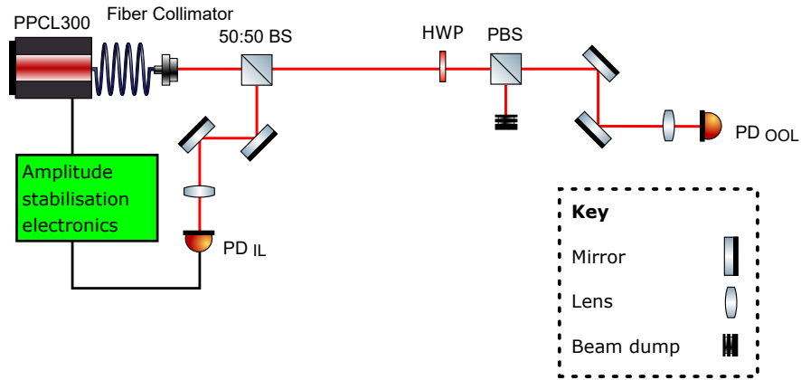
Figure 8.3: Layout of experiment. \text{PD}_{\text{IL}} is the in-loop photodiode (C30641gh) and \text{PD}_{\text{OOL}} is the photodiode being tested. The PPCL300 is a 1550 nm fibre laser from pure photonics. Since the C30641gh is a well-characterised diode, this was used as the in-loop diode for the amplitude stabilisation
