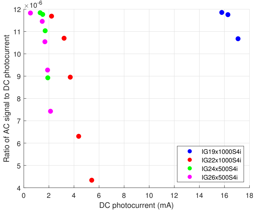
Figure 8.10: Using the apparatus shown in figure 8.3, the DC photo-current that the Laser Components extended InGaAs photodiodes could be operated with while still being linear (i.e. the AC component of the signal would scale linearly with the DC photo-current) was investigated. The spot size on the photodiodes was made as large as possible while still containing 99% of the light power on the photodiode, and were operated with the maximum reverse bias voltage that would still give 1/f noise less than 10mW shot noise at the frequencies of interest for the a gravitational wave detector. The laser's amplitude was modulated. Using a lock-in technique the AC response was measured and divided by the DC photo-current. This was compared to the AC/DC response of the in-loop regular InGaAs photodiode which behaved linearly. When the AC/DC ratio starts to become smaller, the photodiode is no longer behaving linearly. As these diodes become more extended, they perform more poorly.
