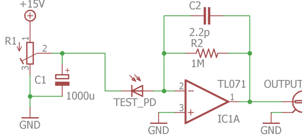
Figure 8.1: The transimpedance amplifier used to measure the dark noise of a variety of photodiodes. For large feedback resistors ( R_2 in the circuit above), a JFET style OP amp such as the TL071 performs better since these have low current noise (e.g. see [27] for a description of noise sources in OP amp circuits). In this application, the TL071 is optimised for between 100\text{ k}\Omega to 10\text{ M}\Omega .
