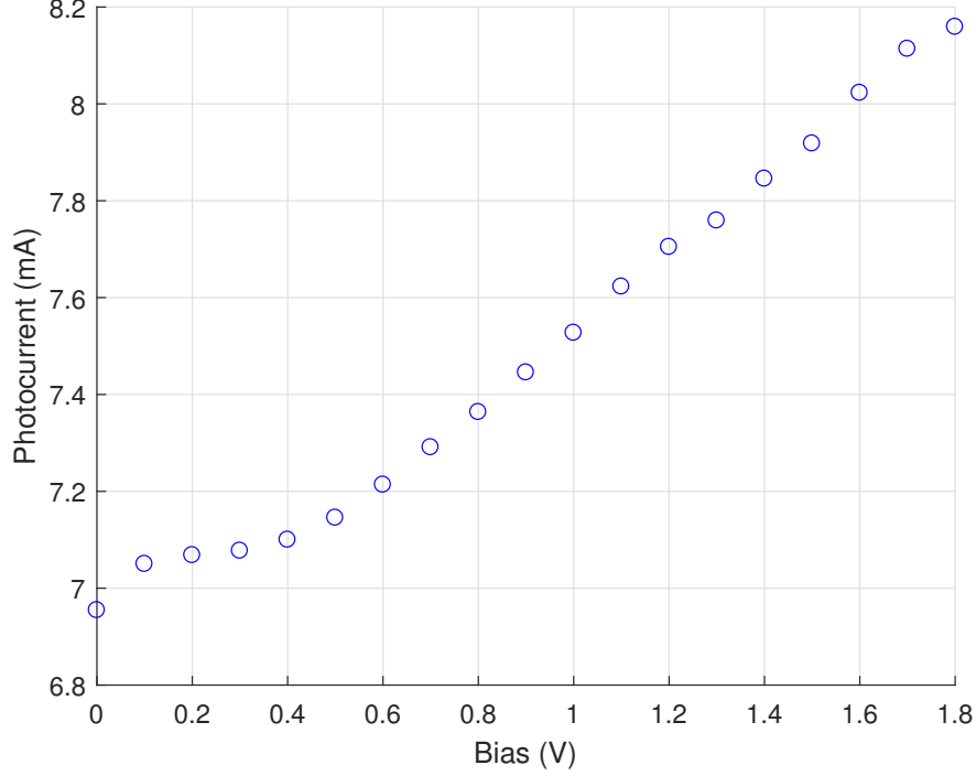
Figure 8.6: A 1550nm laser was used to illuminate the FD10D at room temperature. As the reverse bias is increased, the photo-current out of the FD10D increases by about 17%. This increase in photo-current is due to an increase quantum efficiency since the noise of photo-current matched shot noise.
