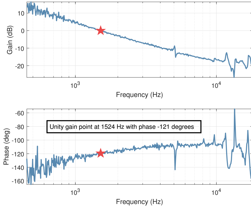
Figure 2.2: Open loop gain of frequency stabilisation loop
