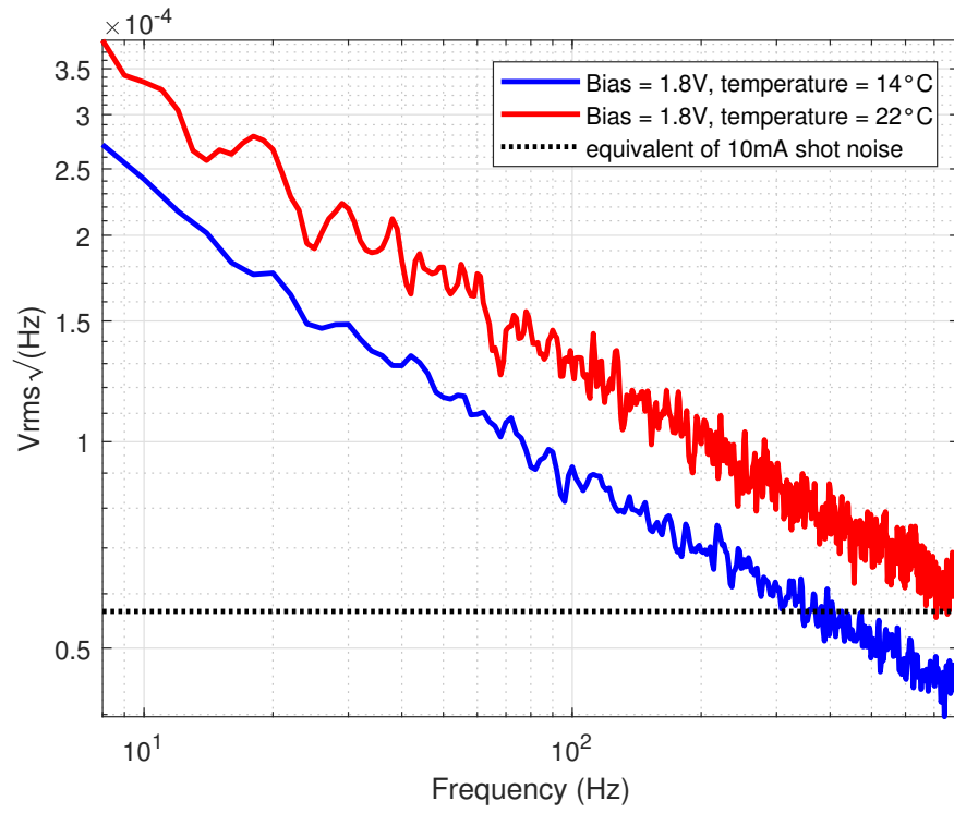
Figure 8.5: The dark noise of the FD10D with a reverse bias of 1.8V at room temperature and 14°C. Although there is a slight reduction in noise, this comes at the expense of less quantum efficiency near the cut off wavelength.
