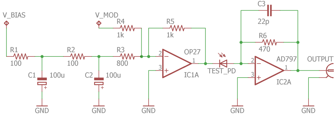
Figure 8.2: Transimpedance amplifier used to measure the quantum efficiency and linearity of photodiodes for up to 20 mW of 1550 nm laser light. The reverse bias supplied to the photodiode is provided by the first OP amp (OP27). The two inputs V_{\text{bias}} and V_{\text{mod}} allows for a quiet low passed DC bias to be set while also being able to perform lock-in type measurements.
