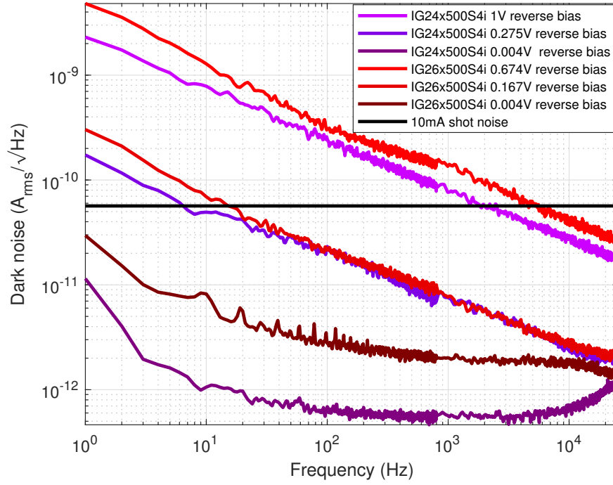
Figure 8.9: The dark noise of two different extended InGaAs photodiodes from Laser Components measured at room temperature. The noise curve for the IG24x500S4i at 0.004V is limited by the noise of the circuit shown in Figure 8.1. As the reverse bias is reduced, so is the 1/f noise. The IG26x500S4i had to be used at a lower reverse bias than the IG24x500S4i to achieve the same noise performance.
