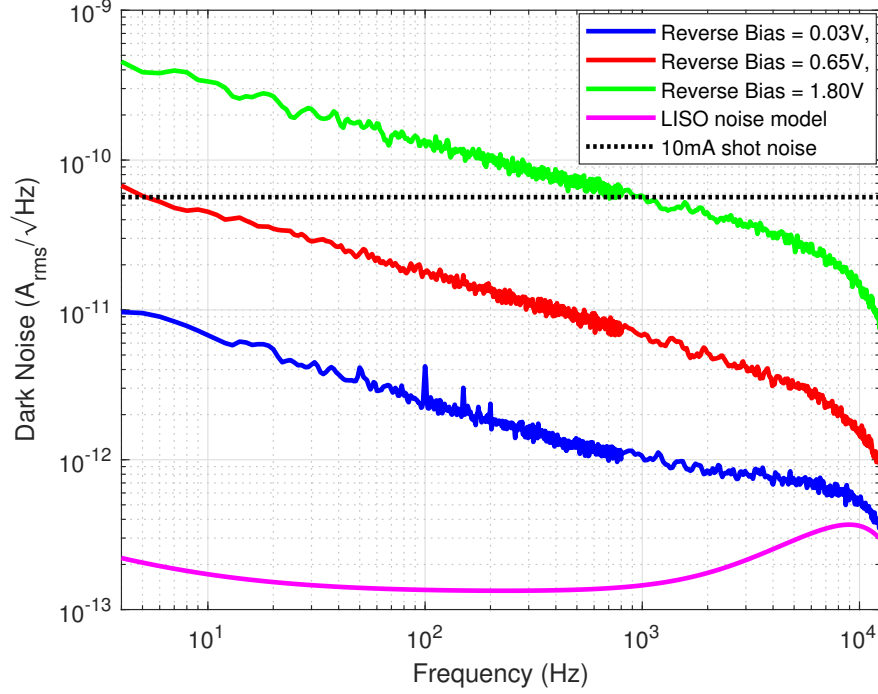
Figure 8.4: The dark noise of the FD10D at different reverse biases. The maximum datasheet value is 1.8V, above this voltage electrons can start tunnelling across the band gap. The rolling off above 9 kHz is an artefact of the circuit. Above 0.65 V reverse bias, the 1/f noise becomes larger than shot noise. At this reverse bias, the quantum efficiency is \sim 70\% . These measurements were made at room temperature.
