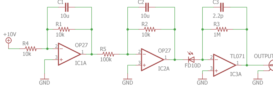
Figure 8.7: Low noise fixed bias voltage dark noise measurement circuit. The 10V reference is generated by an AD587, in this circuit the noise is limited by the voltage noise of the second OP27, but it still reaches 5 \text{ nV}_{\text{rms}}/\sqrt{\text{Hz}} at 10 Hz which is 10 times smaller than the amount of voltage noise which could be converted to current noise that would cause the signal at the output of the TL071 not to be limited by the current noise of the TL071, given the typical dynamic impedance for extended InGaAs photodiodes.
