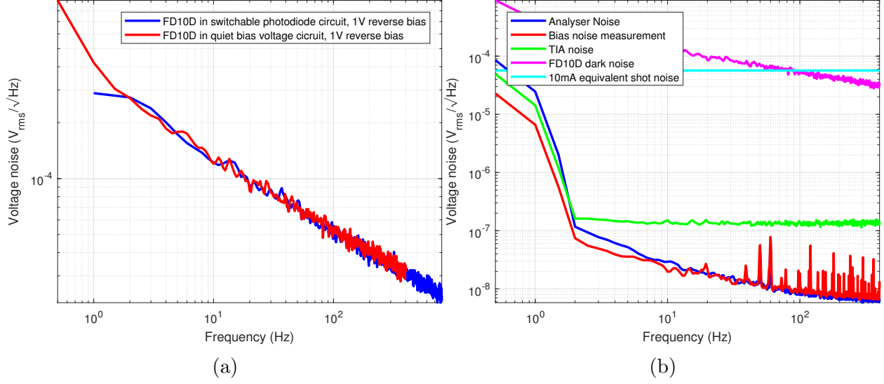
Figure 8.8: The left panel shows that the quiet reverse bias voltage source, shown in figure 8.7, and the more noisy but more flexible bias voltage source, shown in figure 8.1, gave the same results when the dark noise of the FD10D was measured. This means that the flexible reverse bias source is suitable to use for measuring the dark noise of other photodiodes. The bias voltage noise in the quiet bias voltage circuit was found to meet the requirements as shown in the right panel.
