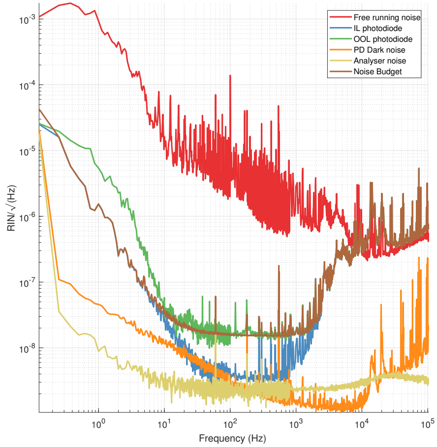
Figure 3.1: Free running and stabilised noise of laser
