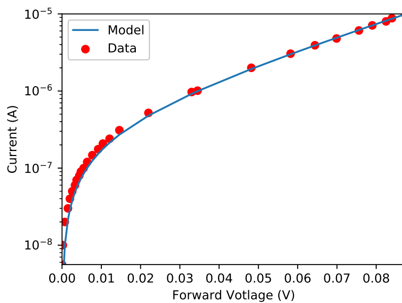
Figure 8.11: The forward IV curve of the IG24x500S4i.
