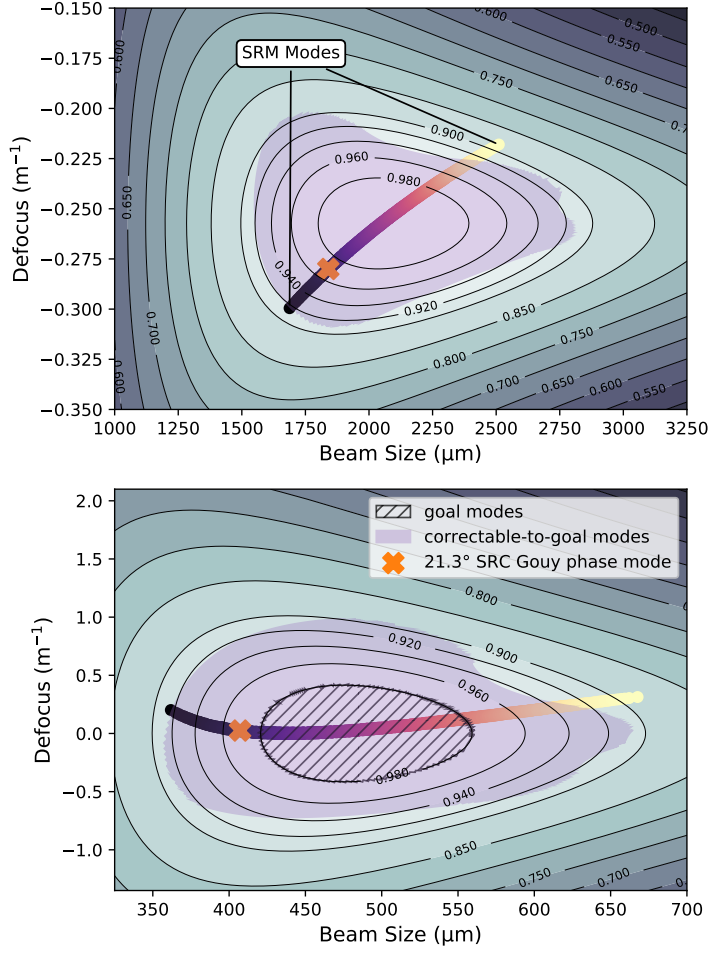
Figure 1.7: Top panel: the set of modes that could be present at the SRM is shown by the black-purple-orange-white curve, as described in chapter 2. The purple region shows which modes can reach 98% mode matching by using the the AWC in HAM6. The orange cross indicates the mode that corresponds to the SRC having a single pass Gouy phase of 21.3^\circ . The contours indicate the mode matching between the arm mode and the OMC mode.
