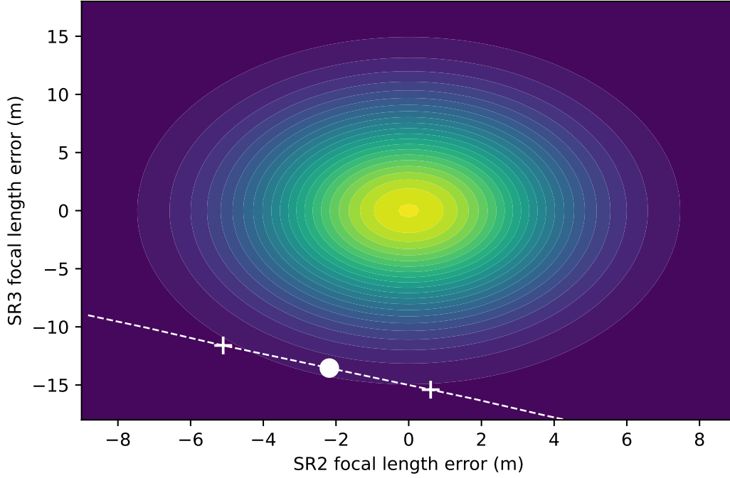
Figure 4.10: The measurement error of SR3 and SR2 follows a normal distribution. These were combined to make a 2-D normal distribution. Dark blue corresponds to the least likely combinations of SR3 and SR2, and bright yellow corresponds to the most likely. The measured Gouy phase was 21.3^\circ [131], this is indicated by the white dashed line. The white circle marks the most likely combination of SR3 and SR2 which gives 21.3^\circ of Gouy phase, and the white crosses show 1 standard deviation from this. The white circle and crosses indicate that the focal length of SR2 is -3.205 \pm 0.003 m and the focal length of SR3 is 17.971 \pm 0.002 m.
