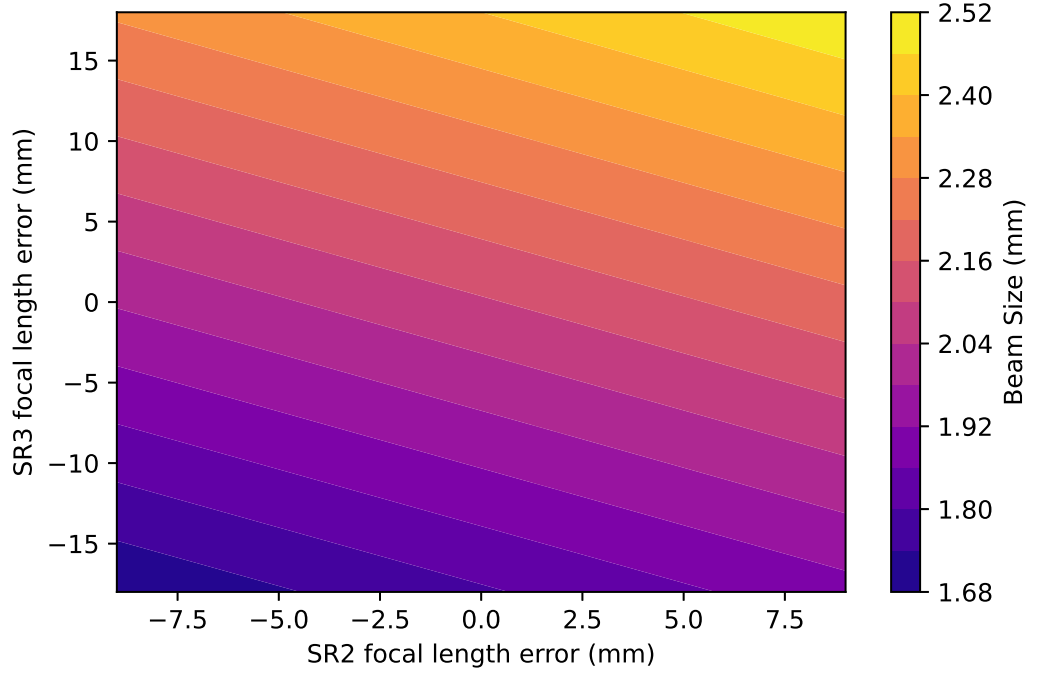
Figure 4.5: The Gaussian width of the beam that is transmitted through the SRM as a function of the error ( \pm 3\sigma ) in focal length of SR3 and SR2. The Gaussian beam width is strongly dependent on the error in SR3's focal length, whereas SR2's focal length error is less important. When the SR3 focal length error > 6 mm and SR2 error is zero the SRC cavity is unstable (see figure 4.9), so this area of the parameter space is unlikely to correspond to the beam at the SRM at LLO.
