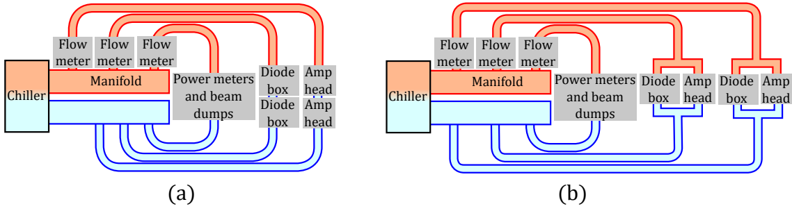
Figure 3.8: Cartoons of water cooling layout for the prototype laser. Panel (a): The laser will be run with the amplifier heads cooled in series with each other to reduce jitter. Panel (b): To perform the amplifier head temperature experiment, the water cooling was arranged so that the amplifiers temperature could be independently controlled.
