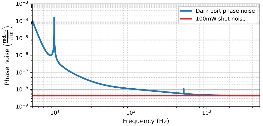
Figure 5.4: The sensitivity curve for the A+ detectors expressed in units of \text{rad}_{\text{rms}}/\sqrt{\text{Hz}} . At frequencies above 1 kHz the noise is flat as it is dominated by shot noise. The red line shows the level of shot noise; this is 4.4 \times 10^{-9} \text{ rad}_{\text{rms}}/\sqrt{\text{Hz}} . At lower frequencies, the noise is increased relative to shot noise due to radiation pressure, coating thermal noise and other noise sources. At 5 Hz, the noise is 1 \times 10^{-4} \text{ rad}_{\text{rms}}/\sqrt{\text{Hz}} .
