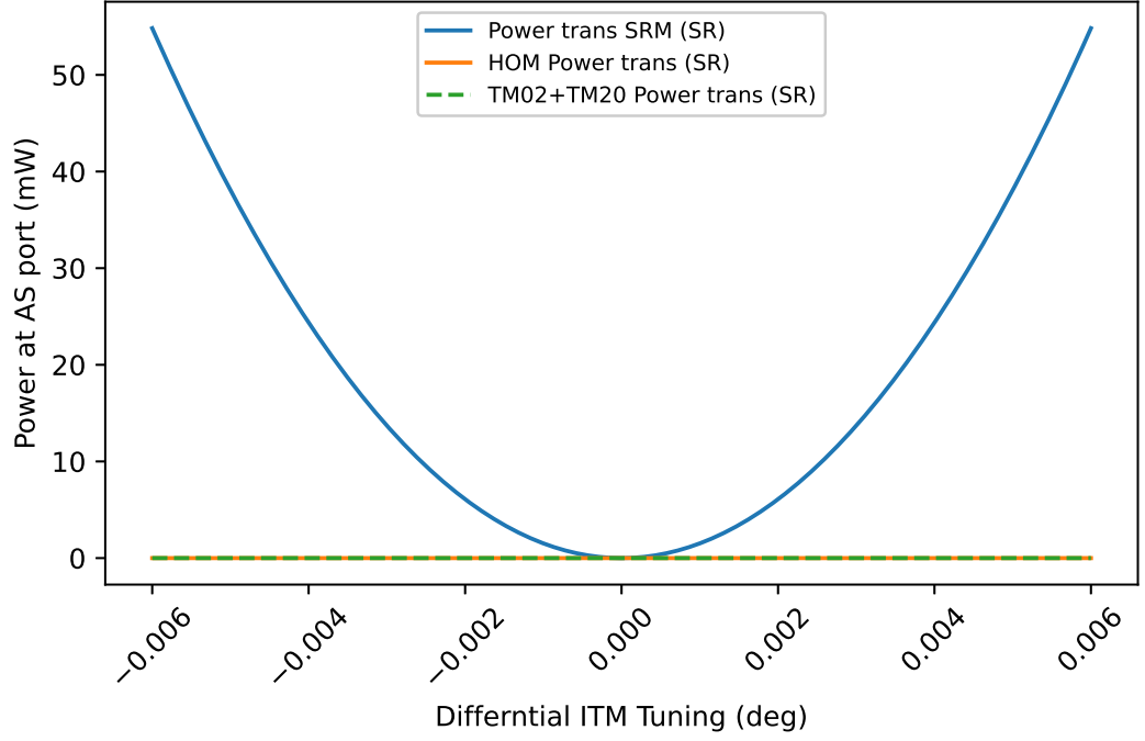
Figure 4.4: The minimum of the dark fringe is at 0^\circ differential ITM detuning, as shown by the blue line. A slight offset causes light to be as the AS port. This result was used to determine tunings for simulating what effect focal length errors in SR3 and SR2 have on the beam transmitted through the SRM. The orange and green dashed line show the HOM content of the beam.
