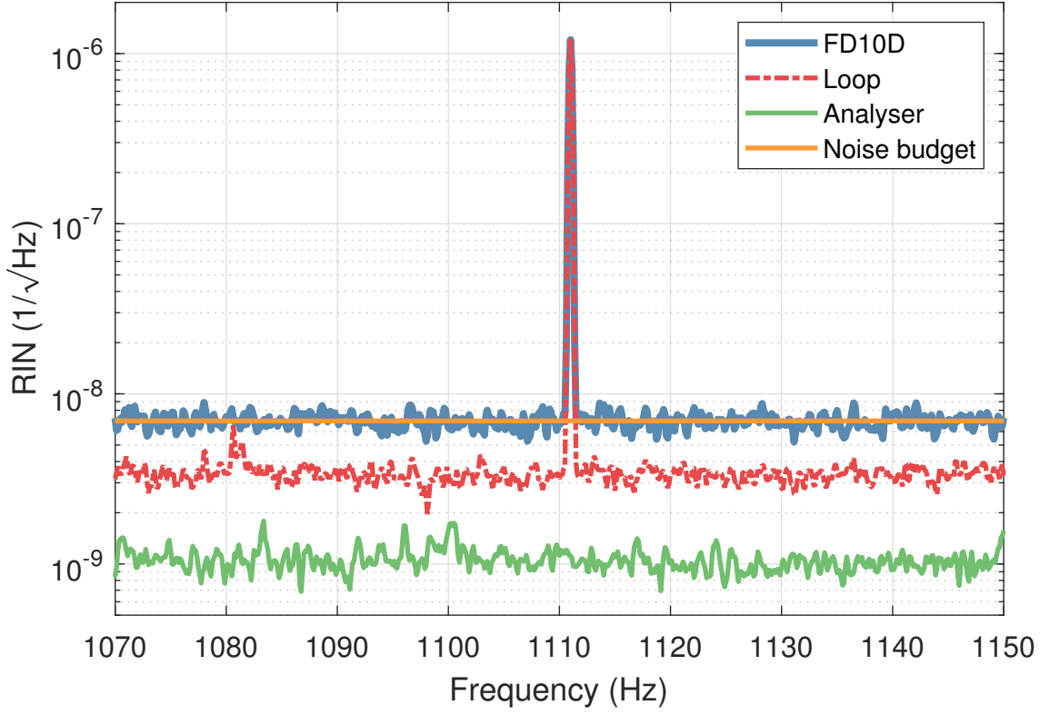
Figure 8.3: The bias of the FD10D was set to 0.6 V, and it was exposed to 15 mW of 1.55 \mu\text{m} light. 15 mA of photocurrent was generated. The noise of the photocurrent produced by the FD10D (blue line) corresponds to the level predicted by Equation 8.3 (orange line) meaning that the quantum efficiency of the FD10D did increase rather than the increase in photocurrent being the result of an avalanche process. The 1111 Hz signal was used to calibrate the measurement.
