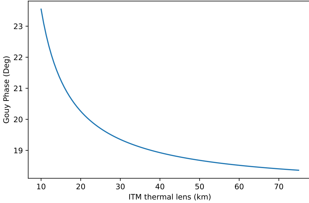
Figure 4.8: Gouy phase between the ITMs and the SRM as a function of the thermal lens in the ITMs for nominal values of SR3 and SR2. The nominal ITM thermal lens is 50 km, and this corresponds to about 19°. More heating results in a greater thermal lens, however at LIGO this is compensated for by the thermal compensation system (TCS).
