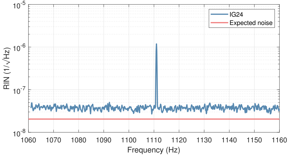
Figure 8.11: The noise of a 1.3 mA photocurrent made by the IG24x500S4i (blue) exceeded the expected amount (red) based on Equation 8.3 by a factor of 1.84. Note that the height of the 1111 Hz peak cannot be expressed in terms of amplitude spectral density units; however, this peak was measured to be the right level, so this beam was not saturating the photodiode.
