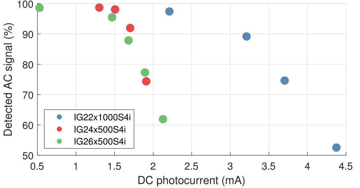
Figure 8.10: The saturation limit of the IG22x1000S4i, IG24x500S4i and IG26x500S4i photodiodes was measured. The photodiodes were biased so that their noise at 10 Hz was equal to the shot noise of a 10 mA current. The IG24x500S4i and IG26x500S4i were exposed to a beam with a 3\sigma width of 220 \mu\text{m} and the IG22x1000S4i was exposed to a beam with a 3\sigma width of 1000 \mu\text{m} . The size of the light modulation of known size was tracked as the DC photocurrent was increased. As the photodiodes saturated, the relative size of the AC signal decreased. The uncertainty in these measurements was \pm 1\% . These photodiodes had low saturation limits compared to the FD10D, which showed no signs of saturation up to 16.5 mA (see Figure 8.4).
