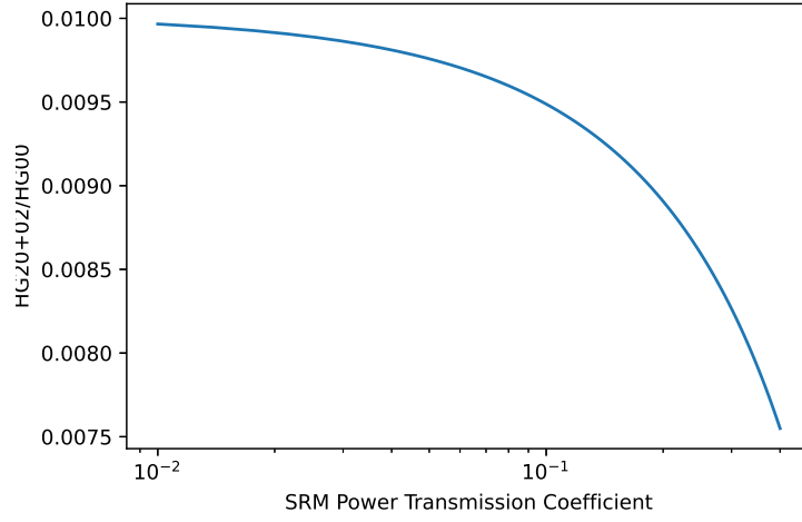
Figure 2.13: Ratio of HG20+02 to HG00 as the transmission of the SRM is increased for a mode mismatch between the arm cavity and the SRC. The interferometer is in RSE mode. A mode mismatch was introduced by setting the focal length of SR3 to be 12 mm shorter than the nominal amount.
