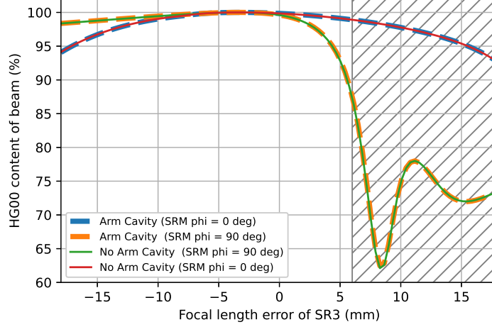
Figure 2.11: The percentage of light which is in the HG00 mode as the focal length of SR3 changes compared to the total light power does not depend on whether there are arm cavities. It is determined by the detuning of the SRM. The blue dashed line shows the behaviour of the beam with arm cavities present and with the SRC in signal recycling mode (SRM \phi = 0^\circ ). The red line shows how the beam changes with focal length error for a single bounce measurement and with the SRC in RSE mode (SRM \phi = 90^\circ ). The orange dashed line corresponds to the interferometer having arm cavities and being in RSE mode (SRM \phi = 90^\circ ). The green line shows behaviour of the beam when the interferometer is configured for a single bounce measurement and is in signal recycling mode. The hatched region indicates where the SRC becomes unstable (see figure 2.9), so the behaviour of the interferometer cannot be accurately simulated for these values of focal length.
