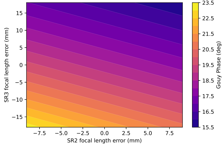
Figure 2.7: Gouy phase between the ITMs and the SRM as a function of the error ( \pm 3\sigma ) in SR3 and SR2. When the SR3 focal length error > 6 mm and SR2 error is zero the SRC cavity is unstable (see figure 2.9), so this area of the parameter space is unlikely to correspond to the beam at the SRM at LLO.
