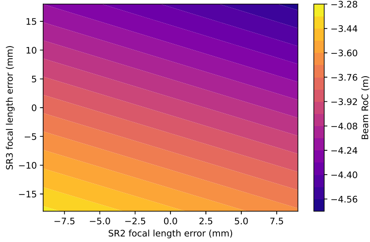
Figure 2.6: The RoC of the beam that is transmitted through the SRM as a function of the error ( \pm 3\sigma ) in focal length of SR3 and SR2. If the arm cavities and the SRC are well mode matched, then the RoC of the beam transmitted through the SRM would be \frac{5.67\text{m}}{1.45} = 3.91\text{m} . When the SR3 focal length error > 6\text{ mm} and SR2 error is zero the SRC cavity is unstable (see figure 2.9), so this area of the parameter space is unlikely to correspond to the beam at the SRM at LLO.
