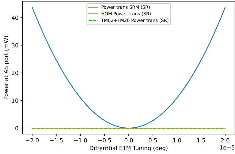
Figure 2.3: The minimum of the dark fringe is at 0^\circ differential ETM detuning, as shown by the blue line. A slight offset causes light to be as the AS port. This result was used to determine tunings for simulating what effect focal length errors in SR3 and SR2 have on the beam transmitted through the SRM. The orange and green dashed line show the HOM content of the beam.
