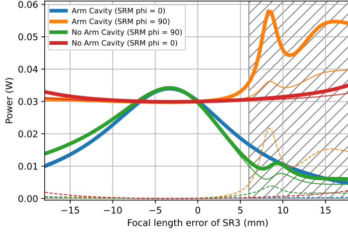
Figure 2.12: The total power transmitted through the SRM for each simulation, is shown in the thick pale lines. The thin solid lines corresponds to the power in the HG00 mode, and the thin dashed lines correspond to the power in the higher order modes. Blue lines show the behaviour when the interferometer has arm cavities and is in signal recycling mode, and the orange lines shows when it is in RSE mode. Green lines show how the power changes when the interferometer is configured for a single bounce measurement and is in signal recycling mode, and the red line shows when its in RSE mode. The hatched region indicates where the SRC is becomes unstable, and so the behaviour of the interferometer cannot be accurately simulated for these values of focal length.
