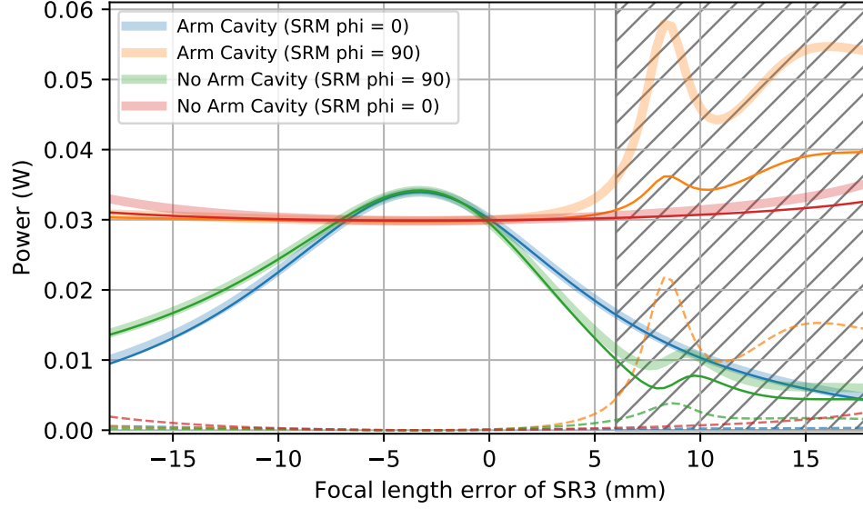
Figure 4.14: The total power transmitted through the SRM for each simulation is shown by the thick pale lines. The thin solid lines correspond to the power in the HG00 mode, and the thin dashed lines correspond to the power in the higher order modes. Blue lines show the behaviour when the interferometer has arm cavities and is in signal recycling mode, and the orange lines shows when it is in RSE mode. Green lines show how the power changes when the interferometer is configured for a single-bounce measurement and is in signal recycling mode, and the red line shows when its in RSE mode. The hatched region indicates where the SRC is becomes unstable, and so the behaviour of the interferometer cannot be accurately simulated for these values of focal length.
