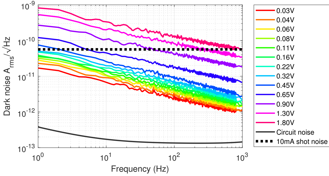
Figure 1.5: FD10D dark noise
