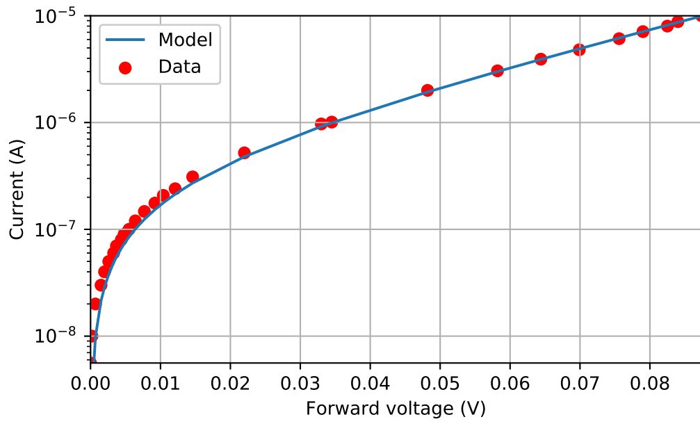
Figure 1.13: I_0 = (360 \pm 10) \text{ nA} , n = 1.02 \pm 0.01
