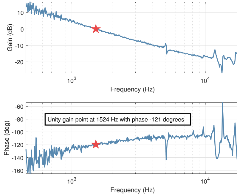
Figure 2.4: Open loop gain of frequency stabilisation loop
