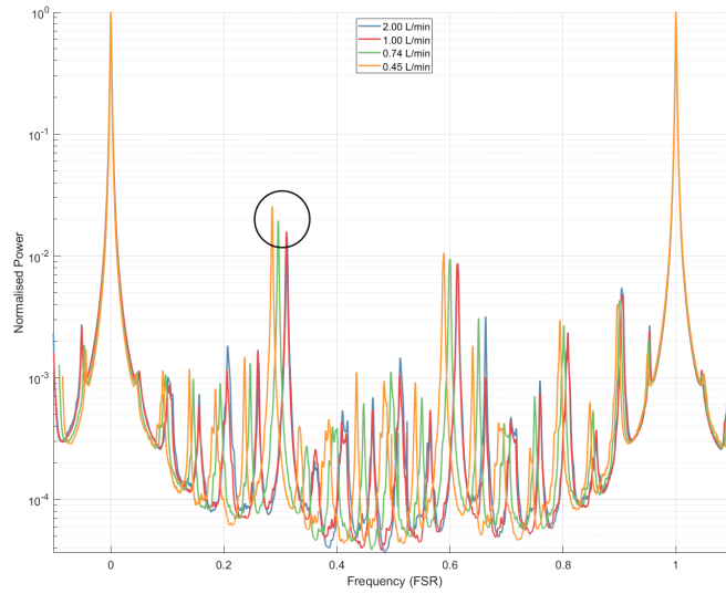
Figure 2.5: Flow rates affecting the thermal lensing, resulting in increased ellipticity
