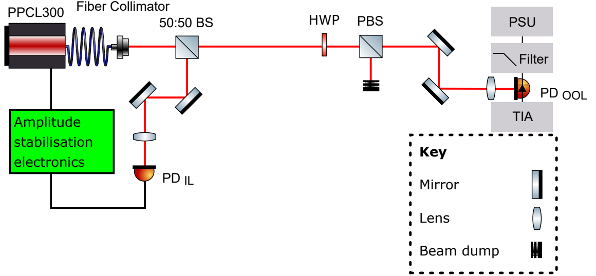
Figure 8.1: Optical layout used for measuring the effect that increasing the reverse bias of a photodiode had on its quantum efficiency and saturation limit. The out-of-loop photodiode, PD_{OOL} , was the photodiode under test (FD10D). A 1.55\ \mu\text{m} laser was used to assess the optical properties of the photodiode. A combination of half wave plate (HWP) and polarised beam splitter (PBS) allowed for the power of the beam to be set and a lens was used to set the size of the beam on the photodiode under test. Amplitude stabilised light was needed to ensure the increase in photocurrent seen when the bias increased was due to an increase in quantum efficiency. The photodiode circuit (TIA) (see Appendix B.2) allowed for shot noise limited measurements of currents around 10 mA and for the bias to be selected.
