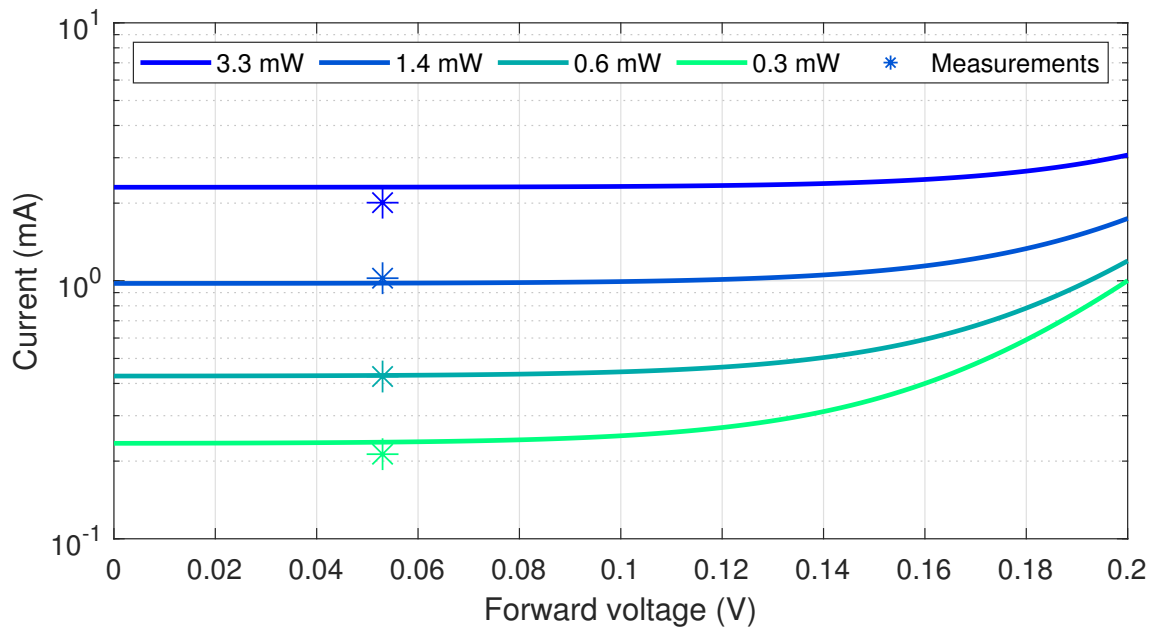
Figure 8.14: Different light levels were shone onto the photodiode and the current produced at 0.05 V forward bias was recorded. These measurements are shown by the stars. Based on the model obtained from the data shown in Figure 8.13, the current flowing through the photodiode was predicted (shown by the lines). The model and the measurements agree with each other, although the photodiode may have been saturating for the 3.3 mW measurement.
