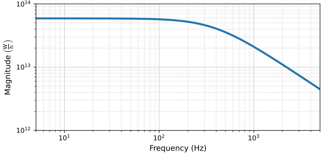
Figure 5.3: The linear response function between strain and light power, expressed in units of light power/gravitational wave strain, at the AS port. The corner frequency at \approx 380 Hz comes from the pole of the coupled SRC-arm cavity.
