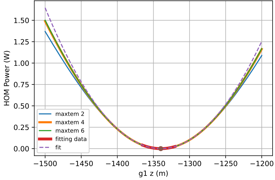
Figure C.1: Optimisation of parameters used in the gauss command to mode match the laser to the arms in the simulations described in chapter 4 and section C.3. The blue, green and orange lines show how the mode matching changes as the beam waist location is changed. As the mode matching becomes larger, more HOM are required, as the blue and green/orange lines diverge. A quadratic was fitted to the data highlighted in red, and the minimum value was used as the waist location parameter for the gauss command.
