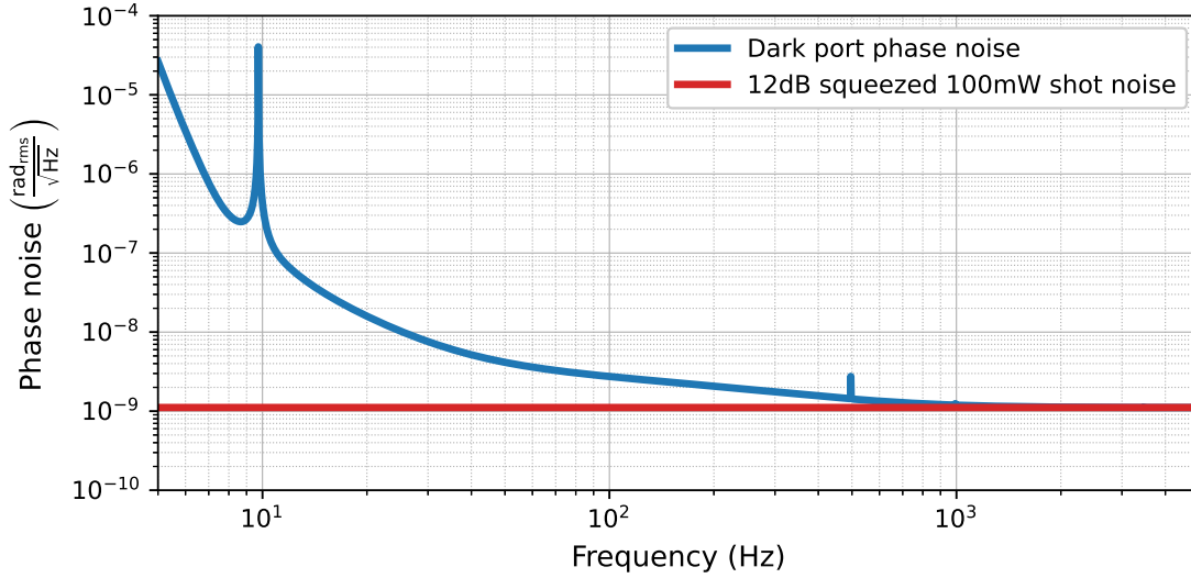
Figure 5.4: The sensitivity curve for the A+ detectors expressed in units of \text{rad}_{\text{rms}}/\sqrt{\text{Hz}} . At frequencies above 1 kHz the noise is flat as it is dominated by shot noise. The red line shows the level of shot noise; this is 1.1 \times 10^{-9} \text{rad}_{\text{rms}}/\sqrt{\text{Hz}} . At lower frequencies, the noise is increased relative to shot noise due to radiation pressure, coating thermal noise and other noise sources. At 5 Hz, the noise is 2.6 \times 10^{-9} \text{rad}_{\text{rms}}/\sqrt{\text{Hz}} .
