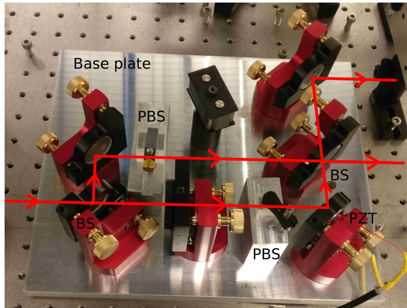
Figure 7.3: Photograph of the Mach-Zehnder base plate. The polarising beam splitters were part of an earlier design; they were removed when the measurements with this apparatus were made.
