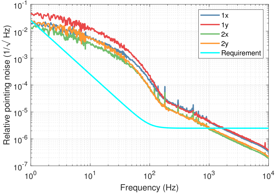
Figure 3.21: The four relative pointing noise degrees of freedom for the beam into the PMC was measured with the DBB. The requirement [122] is shown in light blue. The pointing noise is above the requirement, however the TnT lab has a higher amount of environmental noise; this pointing noise will be less in the PSL. Measurements below 100 Hz may be affected by scattering.
