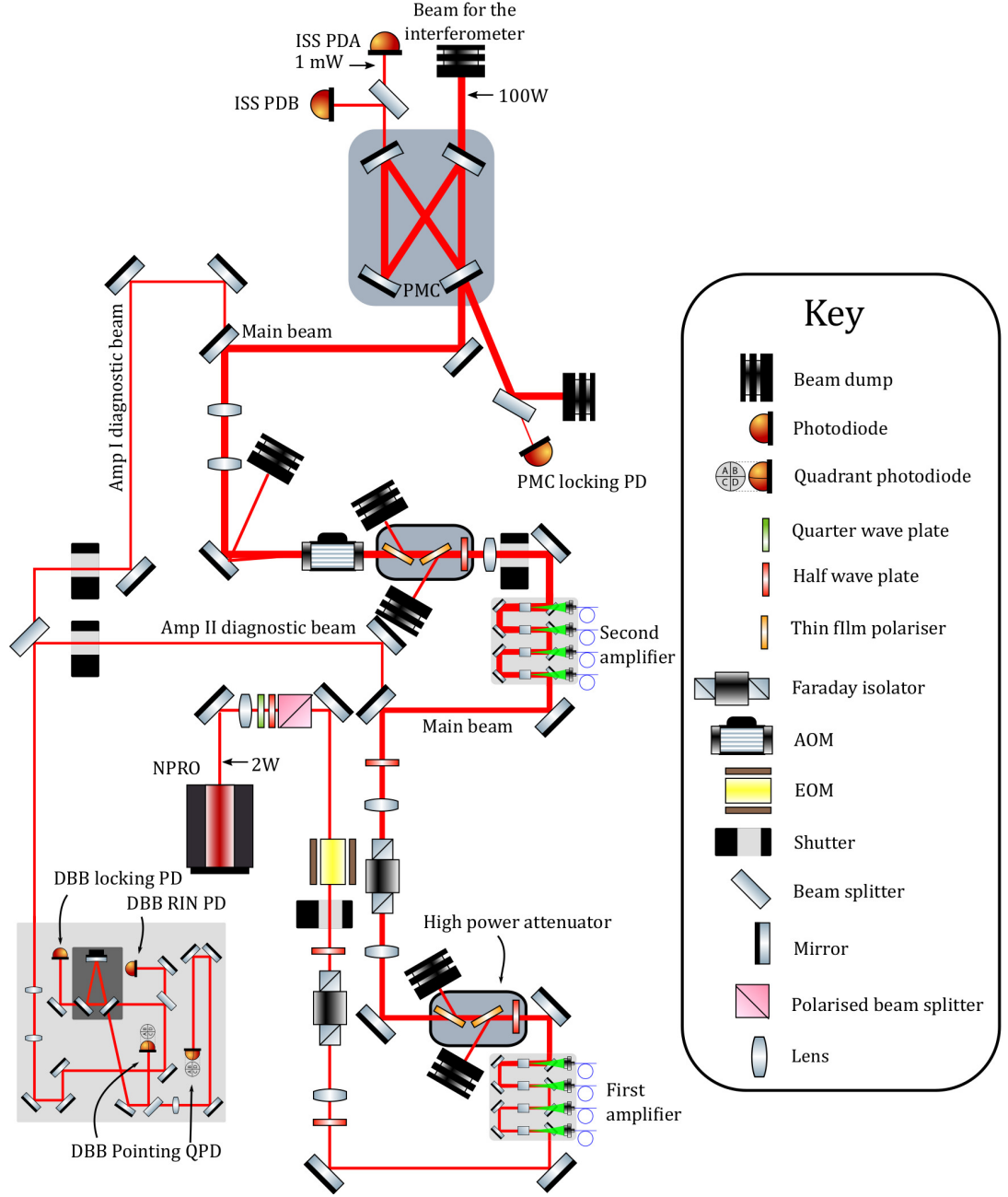
Figure 3.2: Sketch of the prototype optical layout for the PSL. The main and diagnostic beam paths are shown. This sketch shows all the optics in the main beam path as well as the pick-off points for the diagnostic beams.
