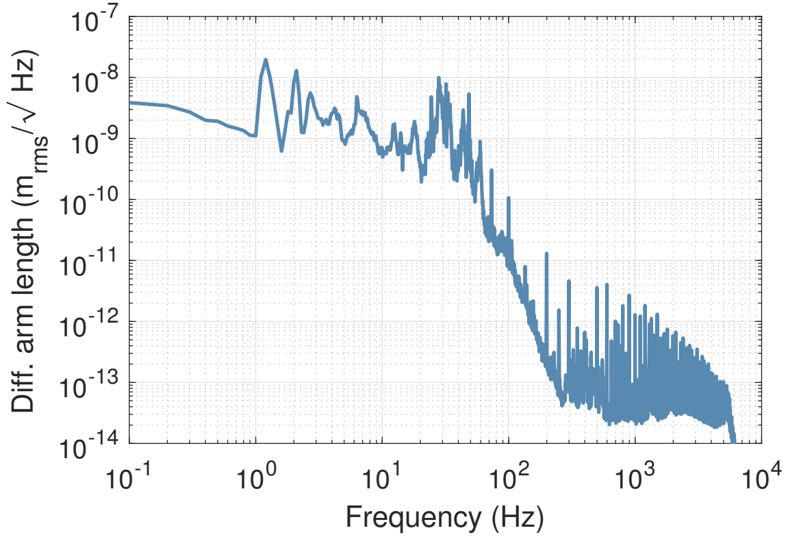
Figure 8.13: Scattering caused there to be a high level of noise in the differential arm length signal. Many peaks related to the balanced homodyne detector suspension can be seen around 30 Hz, and this motion generated phase modulations in the scattered light. The noise was caused by the interference between the scattered light and the signal-carrying light on the photodiodes. For this measurement, shot noise would have been at \sim 10^{-15} \text{ m}/\sqrt{\text{Hz}} .
