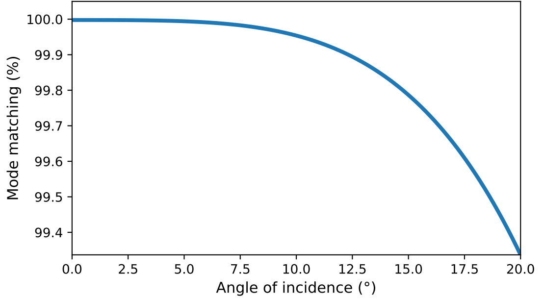
Figure 6.3: Astigmatism is a source of loss. When designing the layout shown in Figure 6.1, the AOI for the curved mirrors was altered to explore how sensitive it was to astigmatism. Using Equation (6.2), the loss was computed. This effect is negligible up to 10^\circ after which it starts to become significant compared to the losses summarised in Table 6.2.
