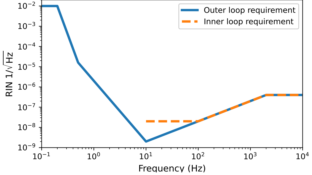
Figure 3.11: A reproduction of the intensity noise requirement from [93]. The outer-loop requirement is shown in blue and the inner-loop is shown by the dashed orange line. To lock the IMC, the inner-loop requirement must be met. At frequencies below 10 Hz, the outer-loop requirement is determined by the radiation pressure noise that is expected to arise due to imbalances in the arm power. The requirement is most stringent at 10 Hz. The requirement relaxes above 10 Hz due to the PRC cavity pole. The inner-loop requirement is less extreme than the outer-loop as it is only used to stabilise the laser in the initial locking sequence.
