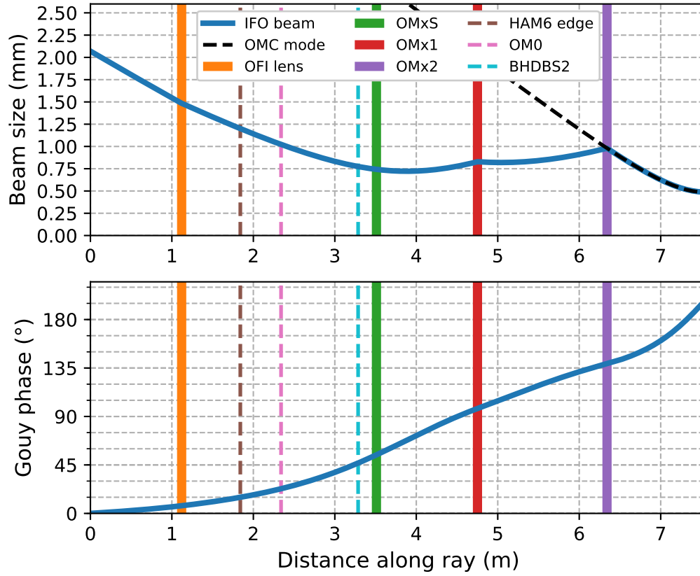
Figure 6.4: The top panel shows the radius of the beam as it travels from the SRM ( z = 0 ) to the waist of the OMC. Significant points along the axis are marked with vertical lines. Less significant, but useful, reference points are marked by dashed vertical lines. The bottom panel shows the Gouy phase shift accumulated by the beam as it propagates along the optical axis.
