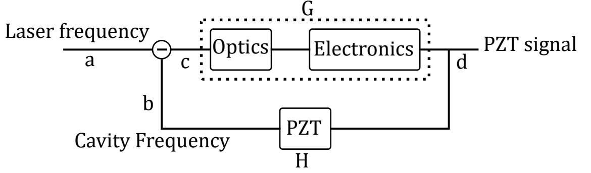
Figure 3.23: The servo can be considered as being made of three parts: the optics, the shaping electronics and the PZT. The transfer function of the optics represents how a difference in frequency between the laser and the cavity transforms into a signal after the demodulator. When at resonance and below the cavity pole, this is a flat transfer function that is proportional to the difference in frequency. Since this cavity pole is in the MHz region and this measurement will only go to the kHz region, the cavity pole can be ignored. The transfer function of the electronics includes everything after the demodulator up to and including the final high power OP amp. The PZT transfer function converts a voltage to a cavity frequency. The PZT acts as a low pass filter due to it having capacitance.
