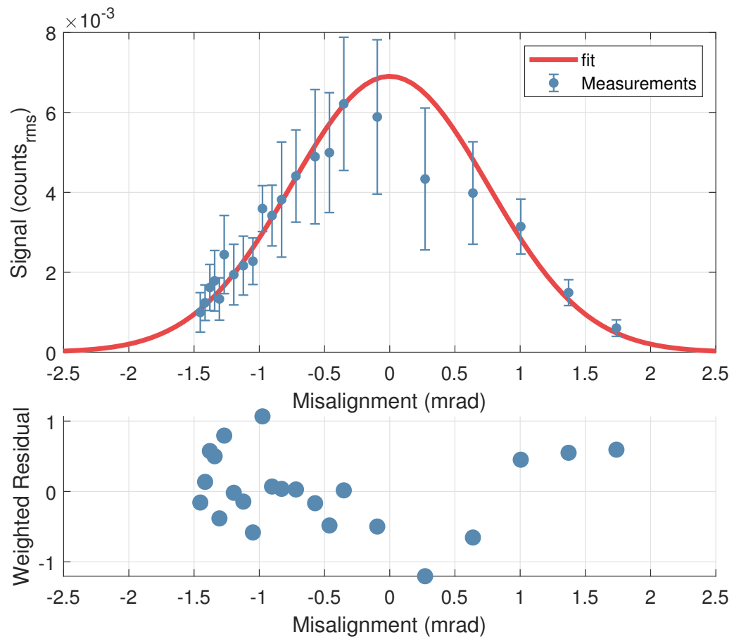
Figure 8.14: Top panel: As the Mach-Zehnder was misaligned, the signal due to the differential arm length modulation decreased. The blue points show the measured signal as a function of misalignment. The data was fit to Equation (8.2), and this is shown in red. Bottom panel: the weighted residuals of the measurements to the fit show no pattern, indicating that the model used was appropriate.
