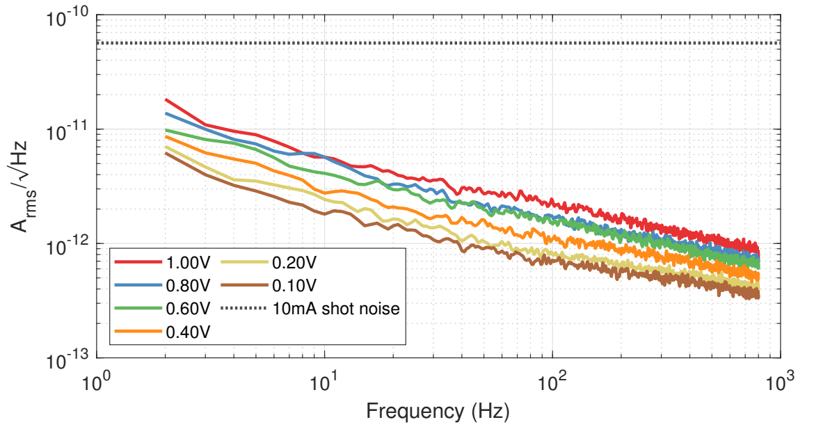
Figure A.7: Dark noise of the G12182-005k at 22°C for a series of reverse biases.
