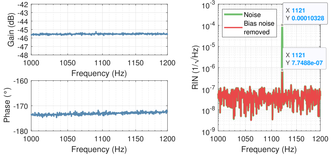
Figure 7.12: A noise projection measurement was performed to determine if the excess noise in the photocurrent produced by the IG24x500S4i (see Figure 7.11) was due to bias noise. The Bode plot of the transfer function between the photodiode's cathode and the output of the transimpedance amplifier when the photodiode was producing 1.3 mA of photocurrent is shown in the left-hand panel. The effect of subtracting bias noise from the signal at the output of the transimpedance amplifier is shown in the right-hand panel. The peak at 1121 Hz was a modulation applied to the photodiode's cathode; 42.5 dB of this signal was removed by using the noise projection technique, and this is approximately the amount expected from the measured transfer function (45.5 dB at 1121 Hz). However, the level of the broadband noise remained unchanged thus indicating that the excess noise witnessed in the photocurrent produced by the IG24x500S4i was not due to bias noise.
