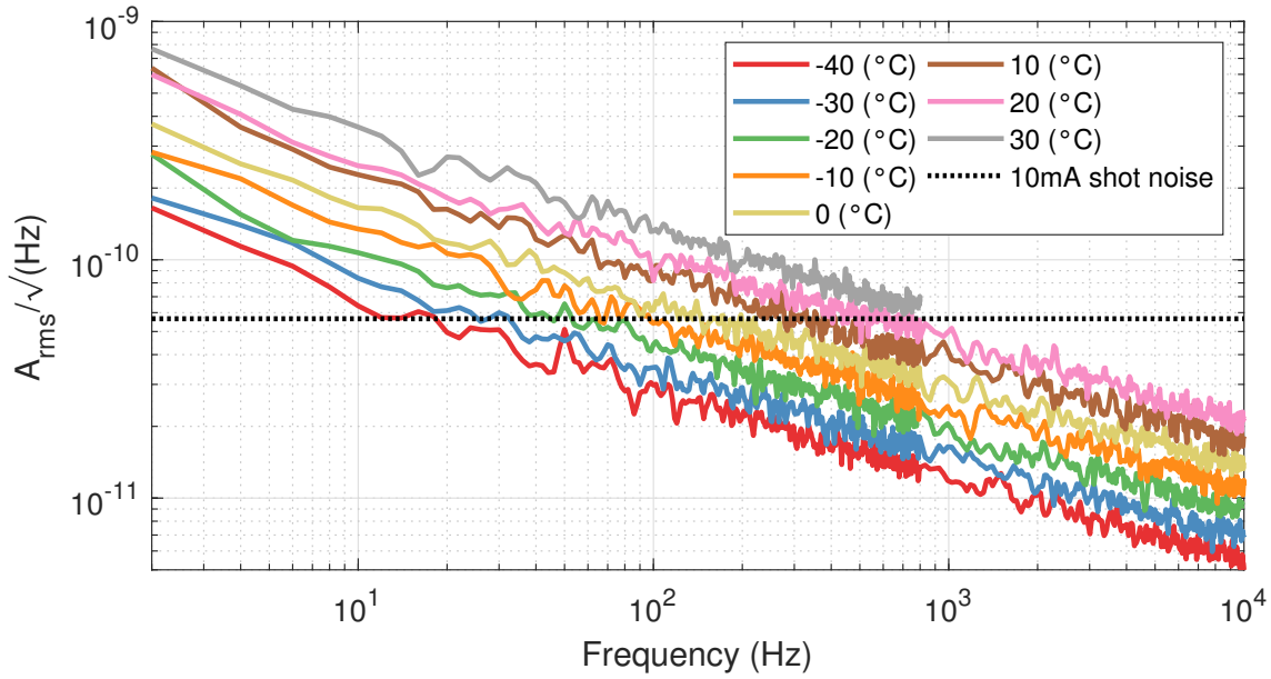
Figure A.8: The dependence of dark noise on temperature for the FD10D at 1.8V reverse bias.
