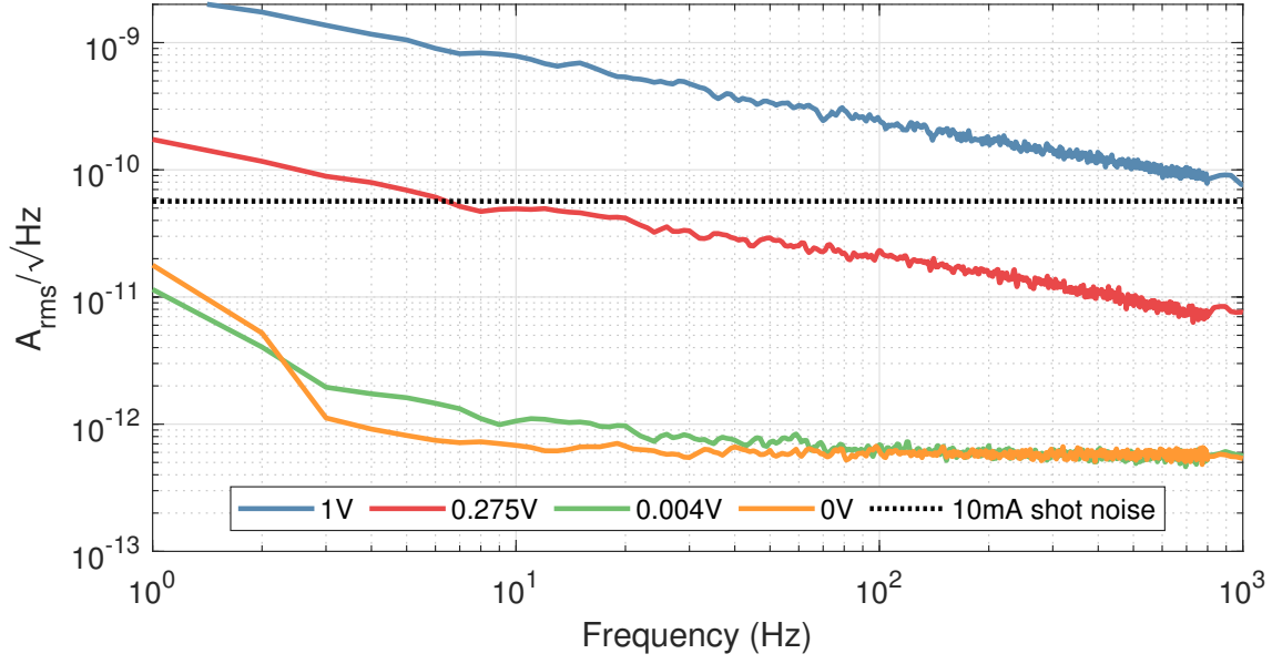
Figure A.1: Dark noise of the IG24x500S4i at 22°C for a series of reverse biases.
