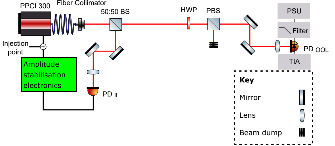
Figure 7.1: Optical layout used for measuring the effect that increasing the reverse bias of a photodiode had on its quantum efficiency and saturation limit. The out-of-loop photodiode, PD_{OOL} , was the photodiode under test (FD10D). A 1.55\ \mu\text{m} laser was used to assess the optical properties of the photodiode. A combination of half wave plate (HWP) and polarised beam splitter (PBS) allowed for the power of the beam to be set, and a lens was used to set the size of the beam on the photodiode under test. Amplitude stabilised light was needed to ensure the increase in photocurrent seen when the bias was increased was due to an improvement in quantum efficiency. The photodiode circuit (TIA) (see Appendix B.2) allowed for shot noise limited measurements of current around 10 mA and for the bias to be selected. The calibration signal was added onto the amplitude stabilisation error signal.
