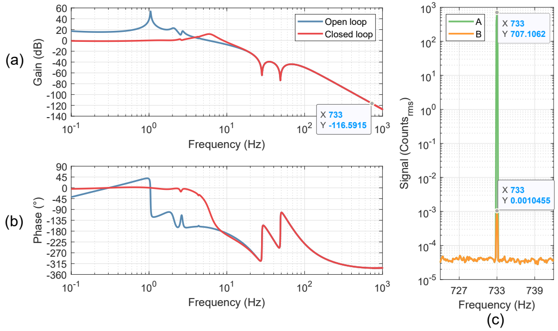
Figure 8.12: Panel (a) and Panel (b) show the Servo's open and closed-loop transfer function. This was calibrated using the factors from 8.1. Panel (c) shows a measurement where a signal was injected at point A in the servo and measured at point B (see Figure 8.11); these two points are separated by a times one block, and so the ratio of these signals represents the closed-loop transfer function of the servo. These measurements are in agreement with the model to within 0.1 dB.
