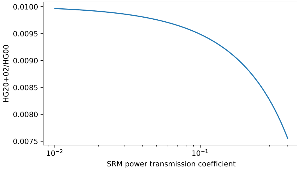
Figure 4.15: Ratio of HG20+02 to HG00 as the transmission of the SRM is increased for a mode mismatch between the arm cavity and the SRC. The interferometer is in RSE mode. A mode mismatch was introduced by setting the focal length of SR3 to be 12 mm shorter than the default amount.
