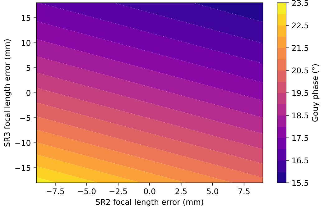
Figure 4.8: The Gouy phase between the ITMs and the SRM as a function of the error ( \pm 3\sigma ) in SR3 and SR2. When the SR3 focal length error > 6 mm and SR2 error is zero, the SRC cavity is unstable (see Figure 4.10), so this area of the parameter space is unlikely to correspond to the beam at the SRM at LLO.
