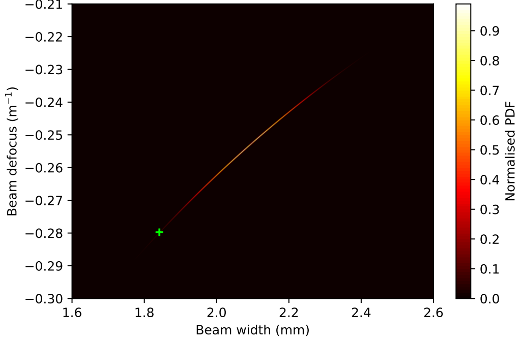
Figure 4.12: The beam parameter at the SRM was calculated for combinations of SR2 and SR3 focal lengths. The associated probability density for these combinations can be calculated (see Figure 4.11), so the probability of the beam parameter having a certain width and defocus can be calculated. The probability density for each pair of beam width and defocus is indicated with the colour bar. The measured Gouy phase of 21.3^\circ [144] is indicated with a green cross (1.84 mm, -2.80 Dioptre). This is a simplified approach since the beam parameter cannot be such that the SRC is unstable, so certain combinations of beam width and beam defocus are not possible. Beam parameters with a width > \sim 2.25 mm result in an unstable SRC, therefore these beams are unlikely to be present at the SRM at LLO.
