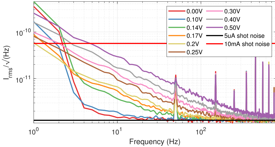
Figure A.15: The noise of the photocurrent produced by the P5968 as a function of bias. The photocurrent due to thermal radiation was expected to be 5\mu\text{A} , and the noise of the photocurrent made by the P5986 at sufficiently low bias reaches the expected shot noise for this current. The benchmark noise corresponding to a 10\text{mA} photocurrent is also shown.
