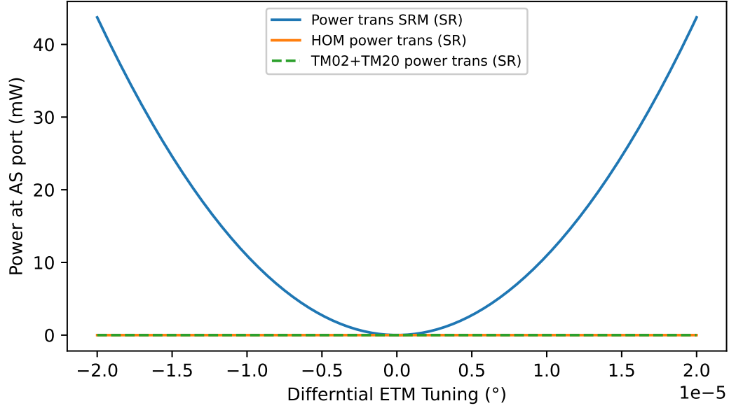
Figure 4.4: The minimum of the dark fringe is at 0^\circ differential ETM detuning, as shown by the blue line. A slight offset causes light to be at the AS port. This result was used to determine tunings for simulating what effect focal length errors in SR3 and SR2 have on the beam transmitted through the SRM. The orange line and dashed green line show the HOM content of the beam.
