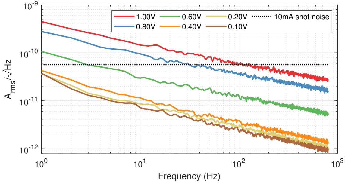
Figure A.5: Dark noise of the G12183-005k at 22°C for a series of reverse biases.
