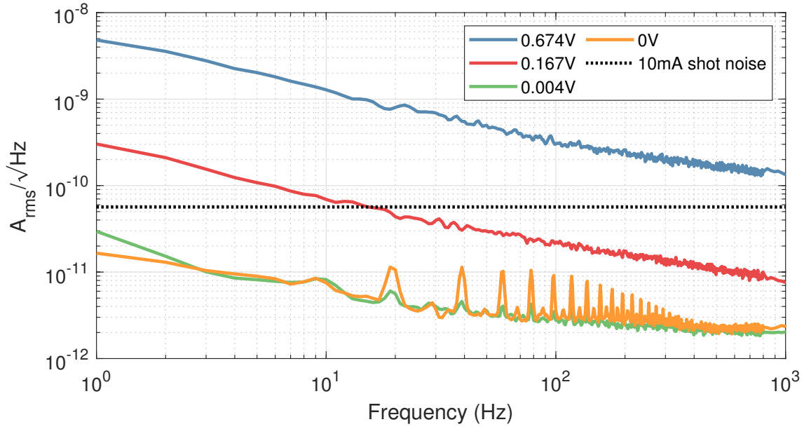
Figure A.2: Dark noise of the IG26x500S4i at 22°C for a series of reverse biases.
