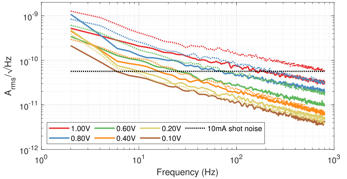
Figure A.4: Dark noise of the G12183-010k at 22°C for a series of reverse biases.
