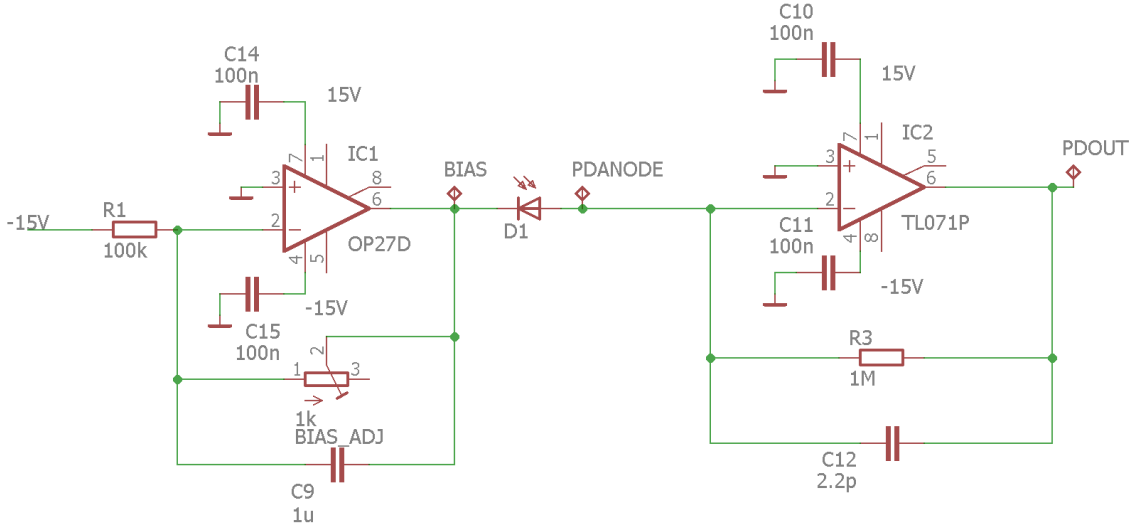
Figure B.2: The circuit used to measure the dark noise of photodiodes. The transimpedance amplifier used is identical to the one shown in Figure B.1. The reverse bias voltage controlled with the potentiometer BIAS_ADJ, and the reverse bias voltage was generated using an OP27 op amp (OP27D) with a gain \ll 1 .
