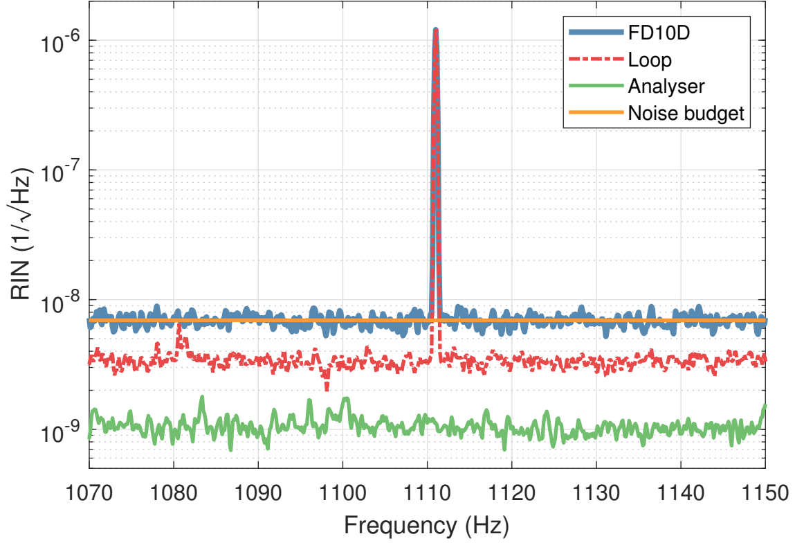
Figure 7.3: The bias of the FD10D was set to 0.6 V, and it was exposed to 15 mW of 1.55 \mu\text{m} light. 15 mA of photocurrent was generated. The noise of the photocurrent produced by the FD10D (blue line) corresponds to the level predicted by Equation 7.3 (orange line) meaning that the increase in photocurrent can only be explained by an increase in quantum efficiency. The 1111 Hz signal was used to calibrate the measurement as this modulation also could be measured on the high-performance in-loop photodiode.
