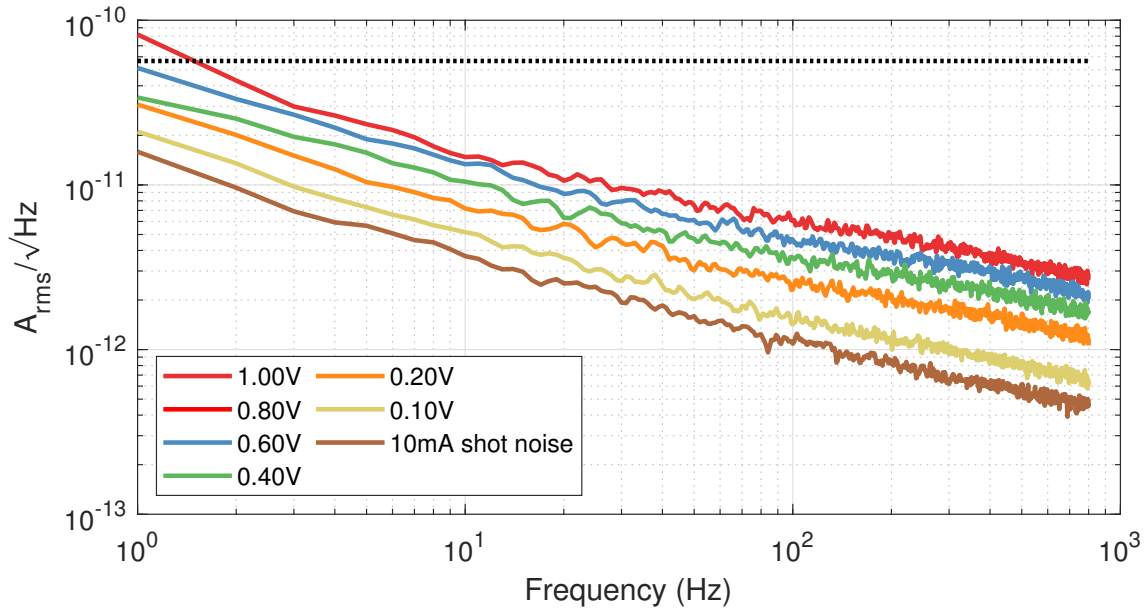
Figure A.6: Dark noise of the G12182-010k at 22°C for a series of reverse biases.
