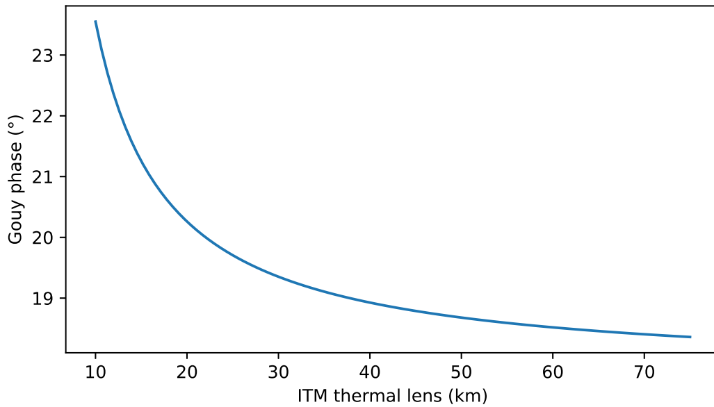
Figure 4.9: The Gouy phase between the ITMs and the SRM as a function of the thermal lens in the ITMs for the default values of SR3 and SR2. The nominal ITM thermal lens focal lengths are 50 km, and this corresponds to about 19°. More heating results in a greater thermal lens, however the LIGO detectors compensate for this with the thermal compensation system (TCS).
