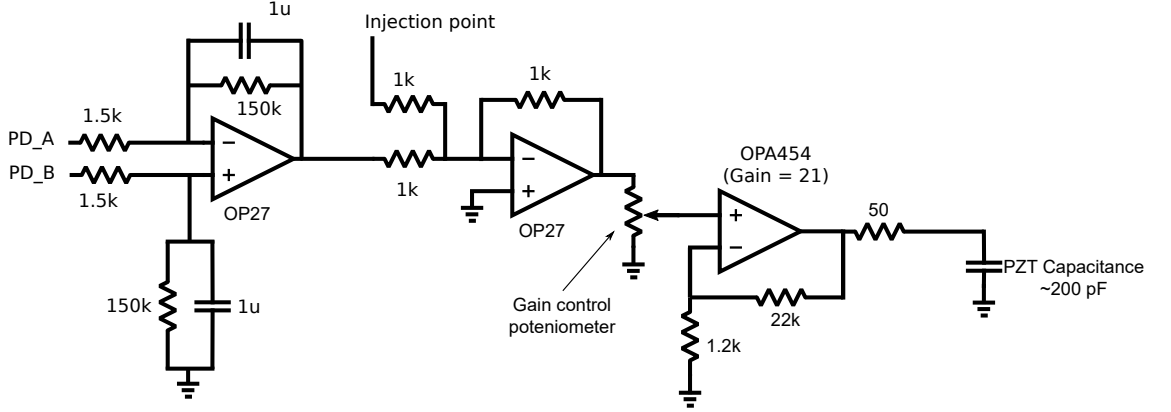
Figure 8.5: Circuit diagram for the electronics used to keep the in-air Mach-Zehnder locked to the middle of a fringe. The inputs PD_A and PD_B connect to two identical transimpedance amplifiers (see Appendix B.2). The first stage subtracts the signals from the photodiodes and provides a 1 Hz roll-off. The second stage allowed for a signal to be applied to the PZT. The final stage boosted the signal to around 100V. The final resistor was used to prevent the OPA454 oscillating when driving the PZT, as the PZT is a capacitive load.
