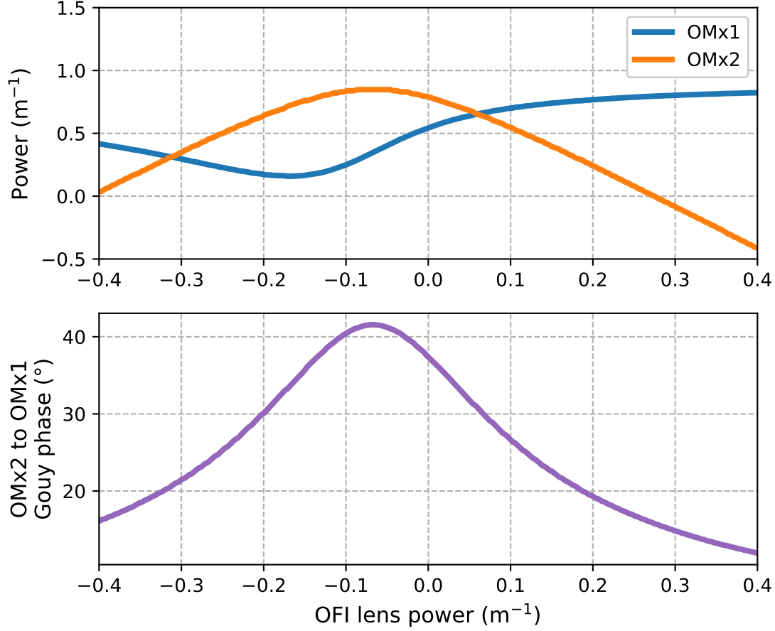
Figure 6.2: Top panel: The choice of OFI lens power affects the combination of OMx1 and OMx2 power that is required for 100% mode matching. Bottom panel: The best choice for of OFI lens that corresponds to obtaining orthogonal control of the beam parameter in HAM6 is where the Gouy phase separation between the pair of OMx1 and OMx2 is closest to 45^\circ . The most Gouy phase separation between OMx1 and OMx2 achievable by this layout is 42^\circ .
