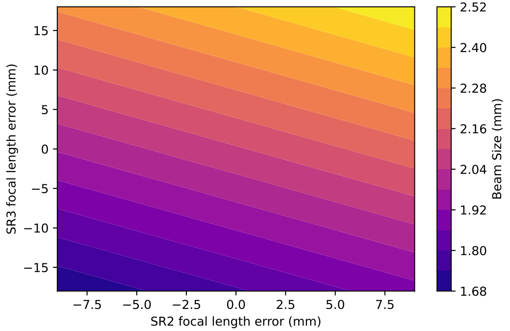
Figure 4.6: The Gaussian width of the beam that is transmitted through the SRM as a function of the error ( \pm 3\sigma ) in focal length of SR3 and SR2. The Gaussian beam width is strongly dependent on SR3’s focal length error, whereas SR2’s focal length error is less important. When the SR3 focal length error > 6 mm and SR2 error is zero the SRC cavity is unstable (see Figure 4.10), so this area of the parameter space is unlikely to correspond to the beam at the SRM at LLO.
