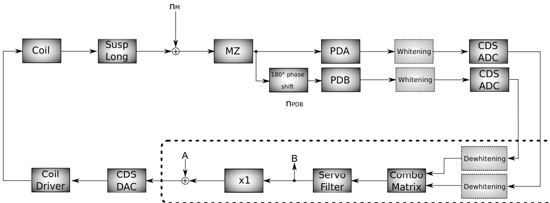
Figure 8.11: Flow diagram showing each block of the servo used to lock the in-vacuum Mach-Zehnder. The digital part of the servo is shown in the dashed area. The injection points A and B were used to calibrate the servo (see Figure 8.12) are around a times one block. The mirrors motion that the servo must correct for is represented by the signal n_M . The information about the Mach-Zehnder differential arm length is encoded by two signals that are 180^\circ out of phase. The whitening and dewhitening filters are paler as these do not affect the gain of the loop.
