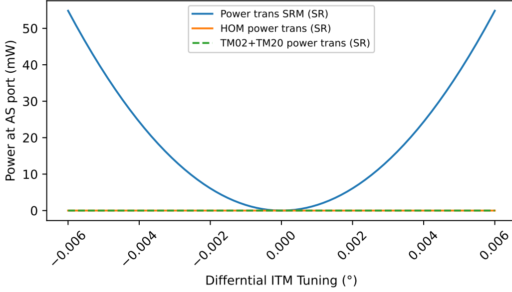
Figure 4.5: The minimum of the dark fringe is at 0^\circ differential ITM detuning, as shown by the blue line. A slight offset causes light to be at the AS port. This result was used to determine tunings for simulating what effect focal length errors in SR3 and SR2 have on the beam transmitted through the SRM. The orange line and dashed green line show the HOM content of the beam.
