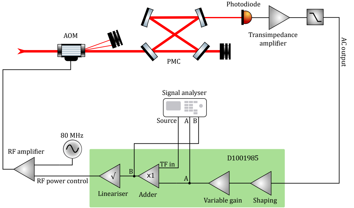
Figure 3.18: Sketch of the amplitude stabilisation servo. The open loop transfer function was measured by injecting a signal into a \times 1 adding stage and measuring the ratio of the signal immediately after and just before this stage.
