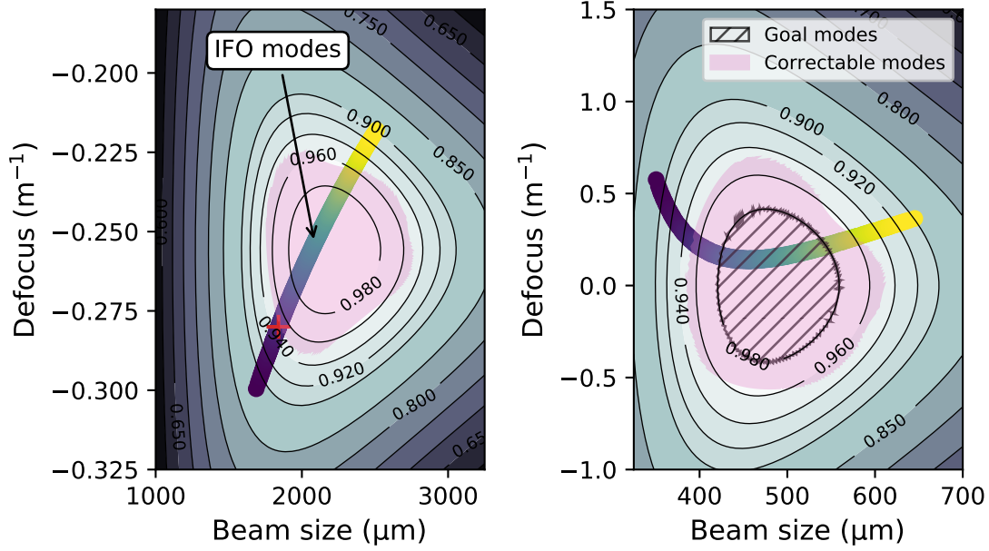
Figure 6.7: The region of WS space covered by the AWC in HAM6 for the layout discussed in Section 6.1. Left panel: the set of modes that is expected to be present at the SRM, as described in Chapter 4, is shown by the purple-blue-green-yellow curve. The pink region shows which modes that can be corrected for so that 98% mode matching is achieved. The contours indicate the mode matching between a mode ( W, S ) and the OMC mode. The red cross indicates the mode size that can be inferred from measurements of the SRC’s Gouy phase at LLO. Right panel: this shows the same modes as the left panel, except they have been transformed by the optical layout to the plane of the OMC waist. Modes within the pink region can be actuated on so they move to the goal region, which is indicated with a hatched area.
