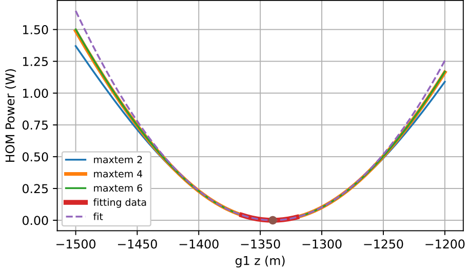
Figure D.1: Optimisation of the parameters used in the gauss command to mode match the laser to the arms in the simulations described in Chapter 4 and Section D.4. The blue, green and orange lines show how the mode matching changes as the beam waist location is changed. As the mode mismatch became larger, more HOM were required; this is why the blue and green/orange lines diverge. A quadratic was fitted to the data highlighted in red, and the minimum value was used as the waist location parameter for the gauss command.
