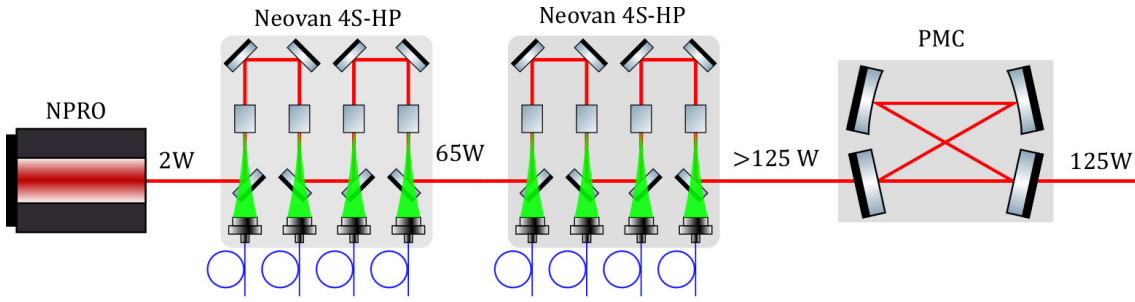
Figure 3.1: Conceptually, the PSL will be made up of four components: the NRPO, two neoVAN-4S-HP amplifiers and the PMC cavity. The NPRO provides seed light with good noise characteristics. These noise characteristics are preserved by the amplifiers, so the resulting beam will have high power and low noise. The PMC filters junk light and RF intensity noise so a spatially pure mode can be sent to the interferometer.
