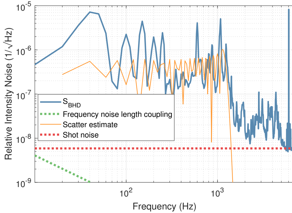
Figure 8.8: The amplitude spectral density of the difference between the two photodiode's signals ( S_{\text{BHD}} ) is shown in blue. The frequency noise that couples via a difference in path lengths between the two arms was estimated, and this is shown in green. The yellow line shows the estimated spectrum due to scattered light.
