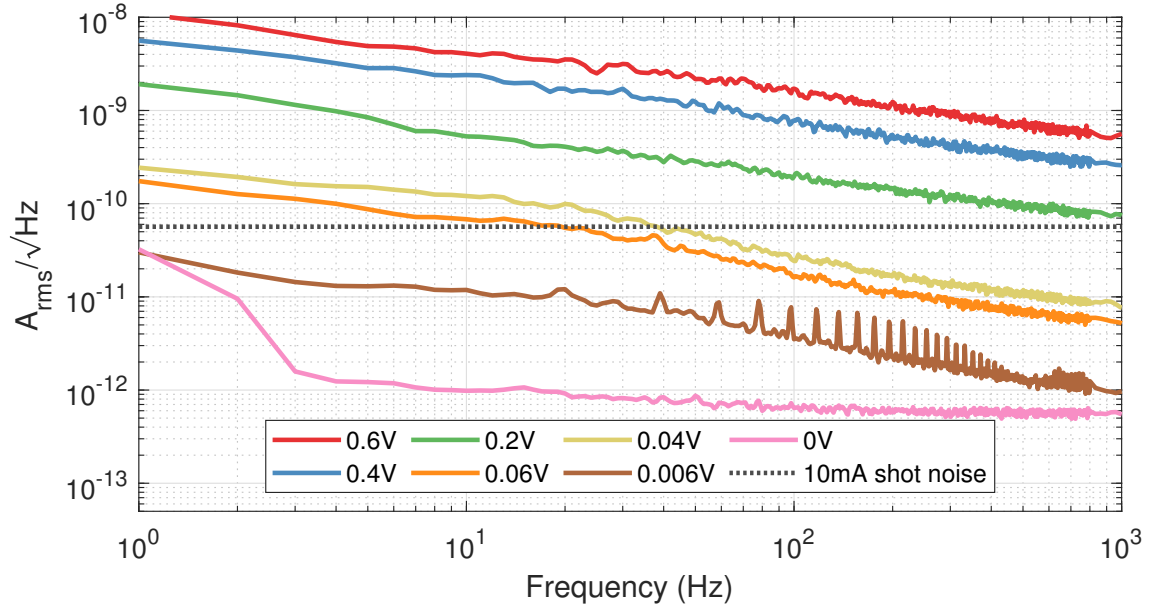
Figure A.3: Dark noise of the IG22x1000S4i at 22°C for a series of reverse biases.
