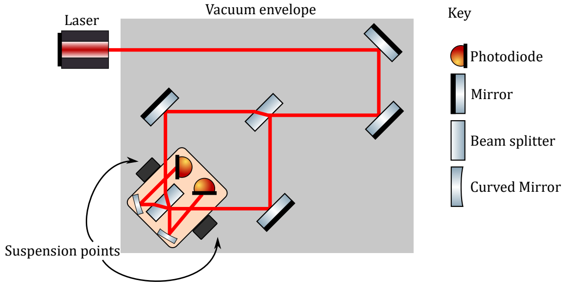
Figure 8.9: Sketch of the in-vacuum Mach-Zehnder. Laser light entered the vacuum system and was steered by suspended optics into a Mach-Zehnder interferometer. The first beam splitter and the two corner mirrors were in identical suspensions. The suspensions are described in Section 8.2.1. The beam splitter for recombining the beam was part of a larger suspended assembly which also included steering mirrors and the photodiodes. Photographs of the components are shown in Figure 8.10. The mirrors and the beam splitter were suspended with identical suspensions, and the recombining beam splitter was part of a larger assembly.
