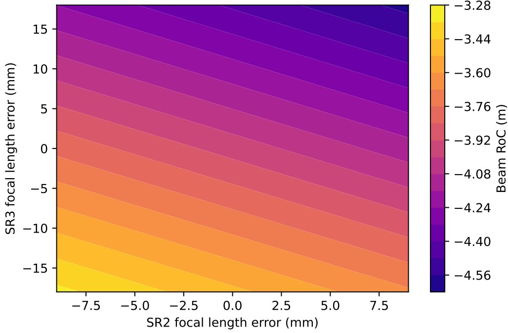
Figure 4.7: The RoC of the beam that is transmitted through the SRM as a function of the error ( \pm 3\sigma ) in focal length of SR3 and SR2. If the arm cavities and the SRC are well mode matched, then the RoC of the beam transmitted through the SRM would be \frac{5.67\text{m}}{1.45} = 3.91\text{m} . When the SR3 focal length error > 6\text{ mm} and SR2 error is zero the SRC cavity is unstable (see Figure 4.10), so this area of the parameter space is unlikely to correspond to the beam at the SRM at LLO.
