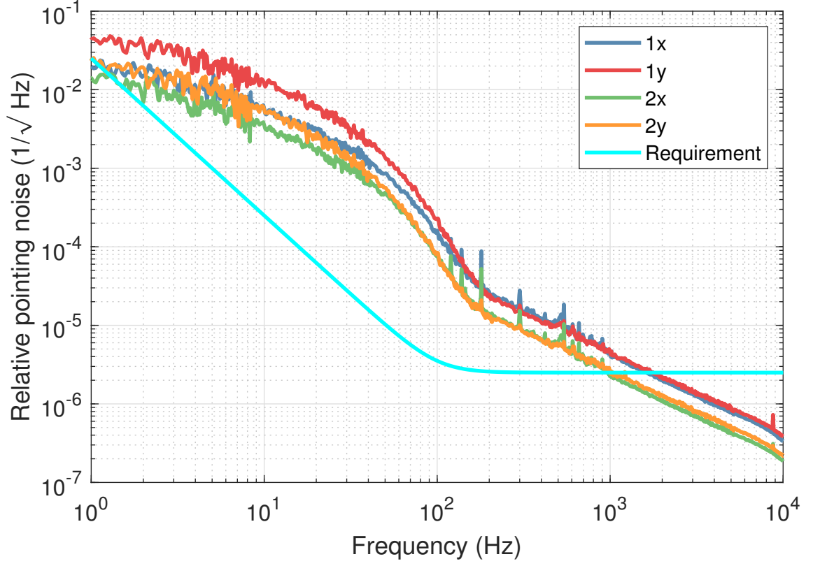
Figure 3.21: The four relative pointing degrees of freedom for the beam into the PMC was measured with the DBB. The requirement [121] is shown in light blue. The pointing noise is above the requirement, however the TnT lab has a higher amount of environmental noise than the PSL. Measurements below 200 Hz were be affected by scattering.
