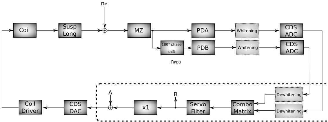
Figure 7.10: Flow diagram showing the each block of the servo used to lock the in-vacuum Mach-Zehnder. The digital part of the servo is shown in the dashed area. The injection points A and B were used to calibrate the servo (see Figure 7.11 are around a times one block. The mirrors motion that the servo must correct for is represented by the signal n_M . The information about the Mach-Zehnder differential arm length is encoded by two signals that are 180^\circ out of phase. The whitening and dewhitening filters are paler as these do not affect the gain of the loop.
