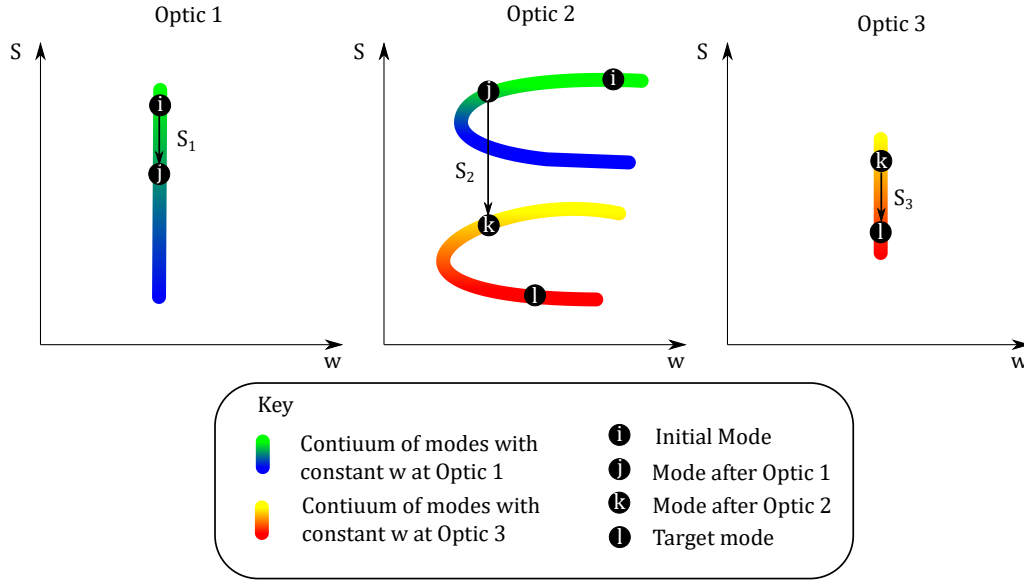
Figure E.2: Sketch of the WS phase space representations of a Gaussian beams at the three positions along the optical axis where a mirror or a lens could be. Examples of such layouts are shown in figure E.1. The optical power of the first optic is given by the difference in the defocus between the initial mode (i) and the second mode (j). The power of the second optic is found by finding the difference in defocus from the blue-green continuum to the red-yellow continuum. There are 2 optical powers that will move the mode j to the red-yellow continuum, and two possible modes in the blue-green continuum that can from which k can be reached, giving 4 possible similar solutions. The algorithm can be set up so that it is only one way of moving between the blue-green and red-yellow continua by limiting their extent. The power of the third optic is found from the difference between the mode k and mode l at optic 3.
