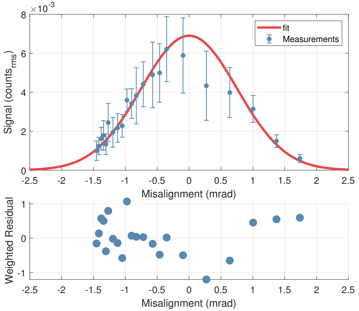
Figure 7.13: Top panel: The in-vacuum Mach-Zehnder was misalignment. As the Mach-Zehnder was misaligned, there was less power in the HG00 mode. The decrease in power for a misalignment \theta is
