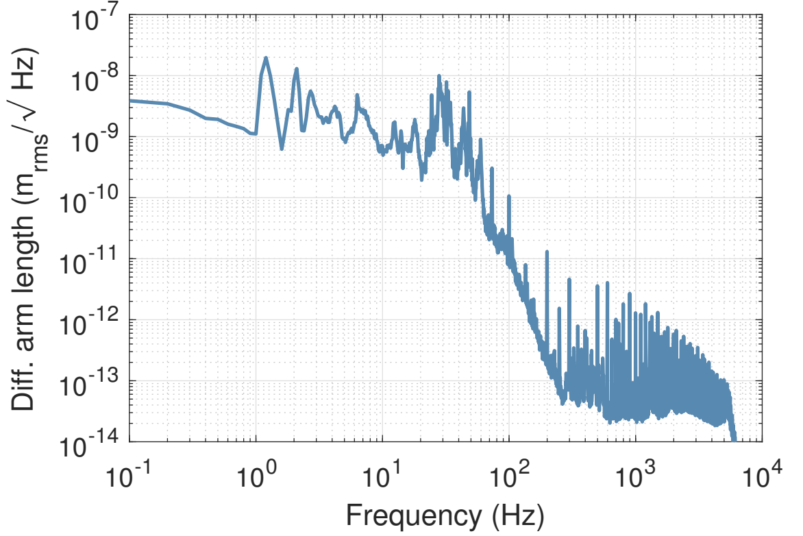
Figure 7.12: Large amounts of scattering caused there to be a high amount of noise in the differential arm length signal's noise floor, this can be seen to limit the noise above \sim 200 Hz. The effect of the pendulums resonance at \sim 1 Hz was mostly removed by the servo but it can still be seen in the noise. Many suspension related peaks can be seen around 30 Hz, these are due to the design of the BHD suspension. The 1/f^4 slope is due to the suspension having two stages. For this measurement, shot noise would have been at \sim 10^{-15} \text{ m}/\sqrt{\text{Hz}} .
