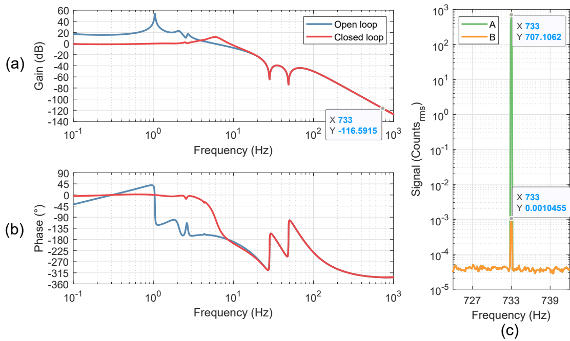
Figure 7.11: Panel (a) and Panel (b) is the Bode diagram of the Servo's open and closed loop transfer function. This was calibrated using the factors from 7.1. Panel (c) shows a measurement where a signal was injected at point A in the servo and measured at point B (see figure 7.10); these two points are separated by a times one block, and so the ratio of these signals represents the closed loop transfer function of the servo. These measurements are in agreement with the model to within 0.1 dB.
