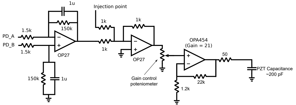
Figure 7.5: Circuit diagram for the electronics used to keep the in-air Mach-Zehnder locked to the middle of a fringe. The first stage subtracts the signals from the photodiodes and provides a 1 Hz roll-off. The second stage allowed for a signal to be applied to the PZT. The final stage boosted the signal to around 100V. The final resistor was used to prevent the OPA454 oscillating.
