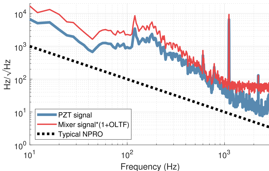
Figure 2.28: The mixer signal combined with the open-loop transfer function is shown in red. This is equivalent to the frequency noise of the system. The PZT signal should agree with this measurement below the unity gain point ( \sim 800 Hz). A signal was applied to the PZT at 1111 Hz. This is below the corner frequency of the PZT and above the unity gain point for the servo. This should match with the mixer signal. There is a factor of two between these two measurements. This can be attributed to imperfect calibration due to nominal parameters of the PMC being used. The typical noise expected from an NPRO is shown by the dashed black line. Between 100 Hz and 1000 Hz, there is a bulge in the frequency noise. This is likely due to acoustically driven noise of the PMC as the PMC is not vacuum sealed. This can be converted to length noise with a factor of \sim 10^{-14} m/Hz.
