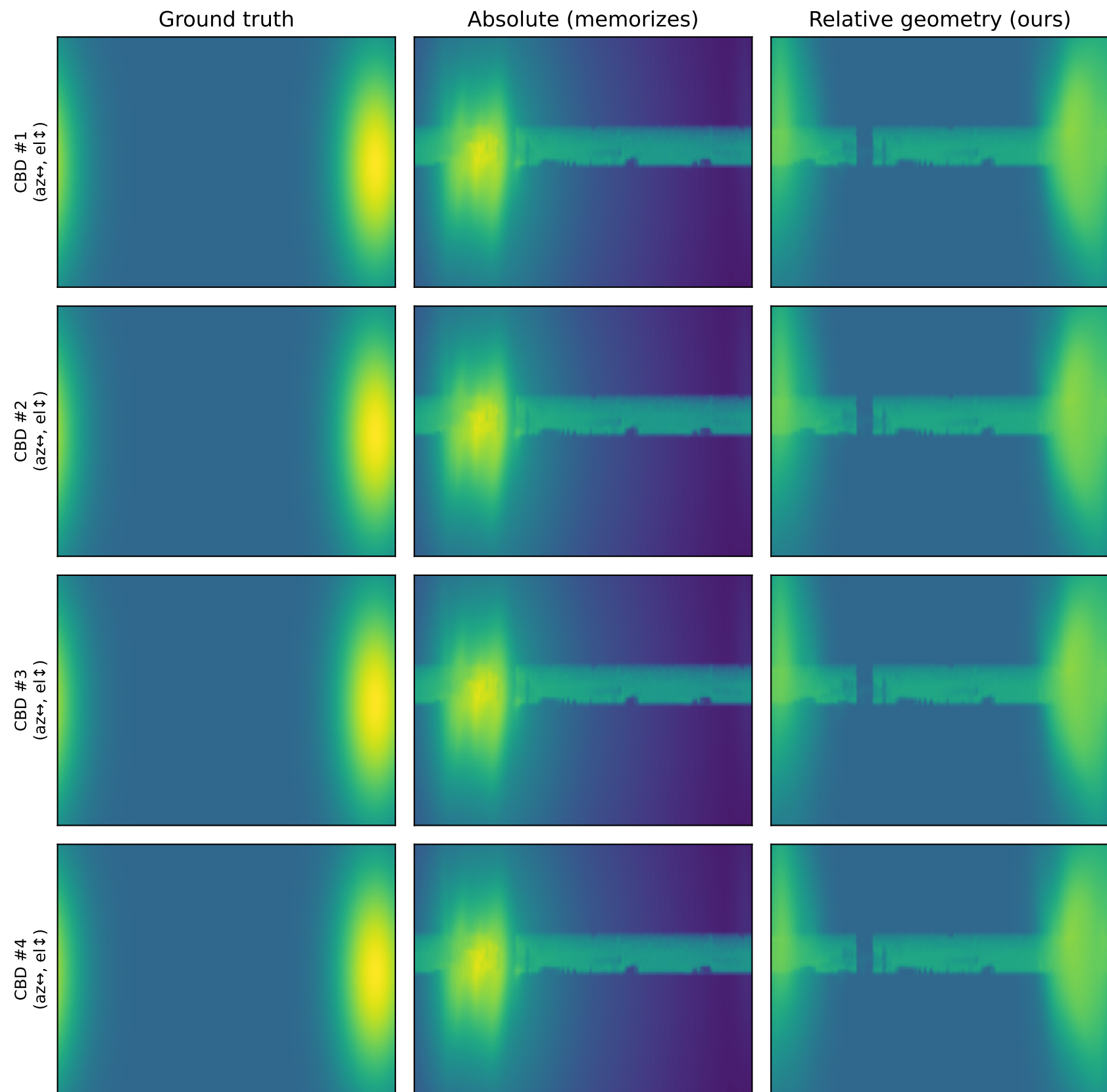
Zero-shot held-out spectra on an UNSEEN scene (CBDcrossroad): relative matches GT, absolute collapses
