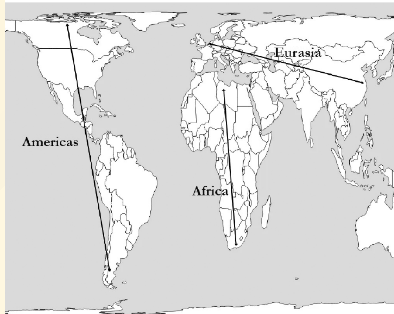
2.3 Verticality and horizontality of the continents based using map in Diamond (1997). Gall-Peters map projection.
